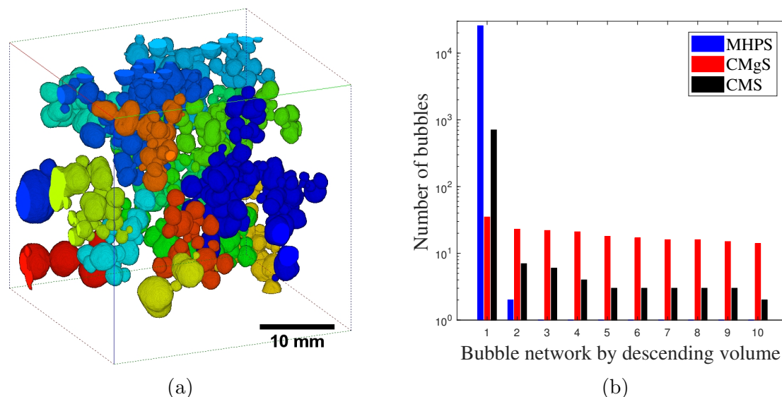
Figure 4: (a) CT reconstruction of the 16 largest bubble networks within 30 Pa CMgS, assigned different colors for visualization (with warmer colors representing reduced network volumes) and (b) a comparison of the number of bubbles comprising the 10 largest bubble networks (sorted by descending bubble volume) for the three Mg(OH) 2 -rich test materials.
