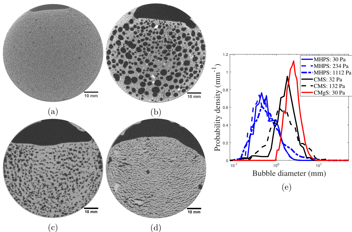
Figure 3: X-ray computed tomography slices through (a) 30 Pa MHPS, (b) 30 Pa CMgS, (c) 32 Pa CMS and (d) 132 Pa CMS following 6 h in situ hydrogen peroxide decomposition (following the cessation of bed expansion), together with (e) bubble size distributions within the three test materials.
