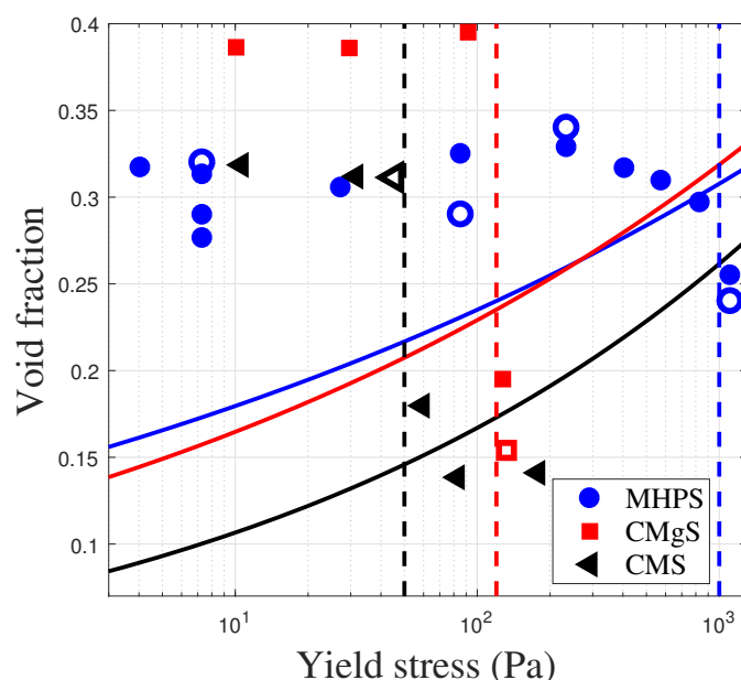
Figure 2: Maximum void fractions observed across a range of yield strength conditions for three \text{Mg}(\text{OH})_2 -rich sediments, (many of the MHPS data are reproduced from Johnson et al. 3 ); solid and open symbols represent 1 and 6.5 L scale tests respectively, the solid line profiles represent the neutral buoyancy condition, whereby the sediment density reaches equilibrium with an aqueous supernatant and vertical dashed lines at \tau = 60, 120 and 1000 Pa indicate apparent transitions to a lower holdup regime above proposed critical fracture strengths .
