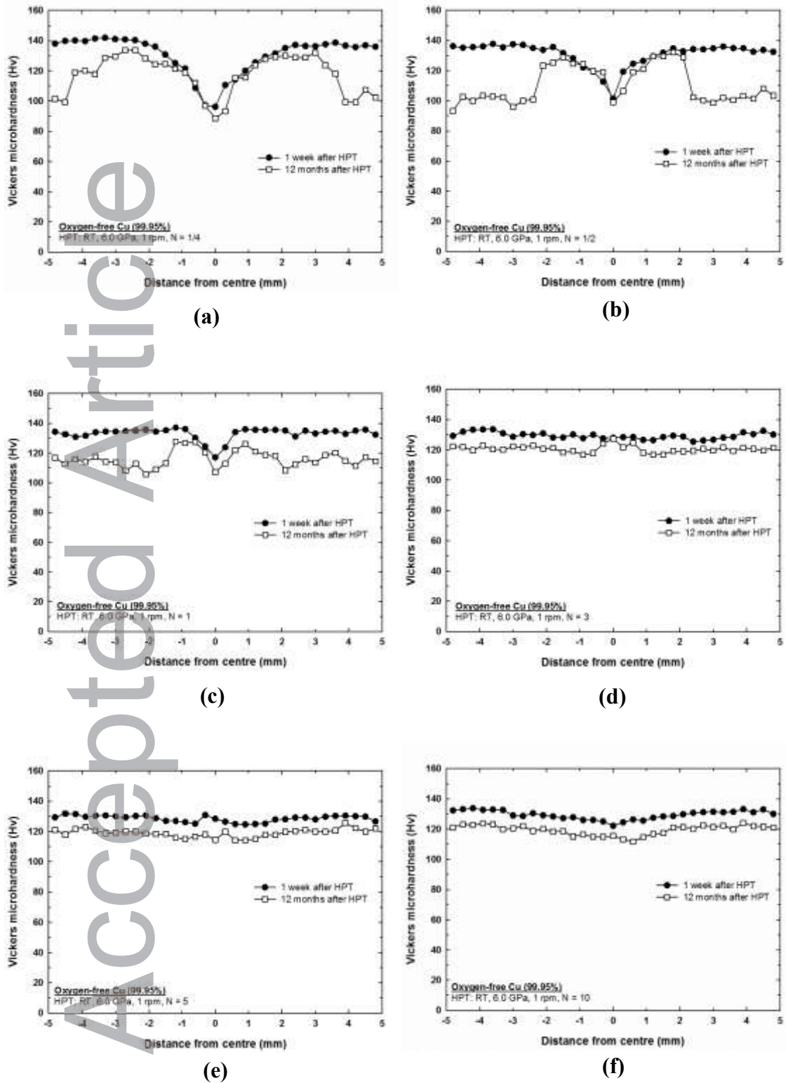
Fig. 1 Vickers microhardness measurements recorded along diameters of oxygen-free Cu discs after 1 week and 12 months of HPT processing for different numbers of turns (a) 1/4, (b) 1/2, (c) 1, (d) 3, (e) 5 and (f) 10 turns.
