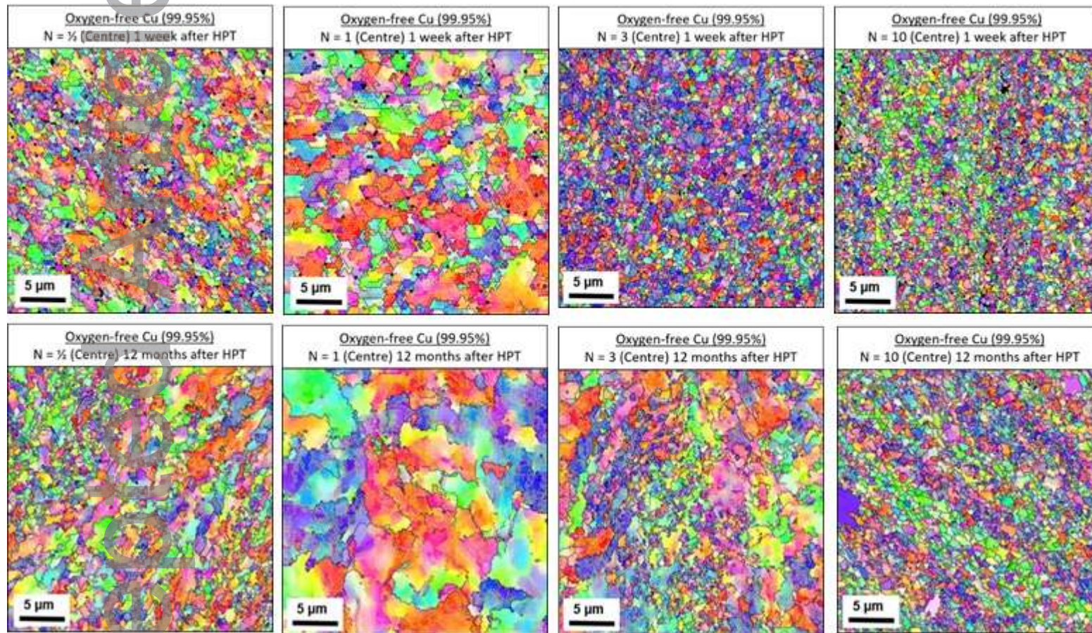
Fig. 2 OIM images of the central regions for oxygen-free copper discs 1 week (upper) and 12 months (lower) after HPT processing for 1/2, 1, 3 and 10 turns.
