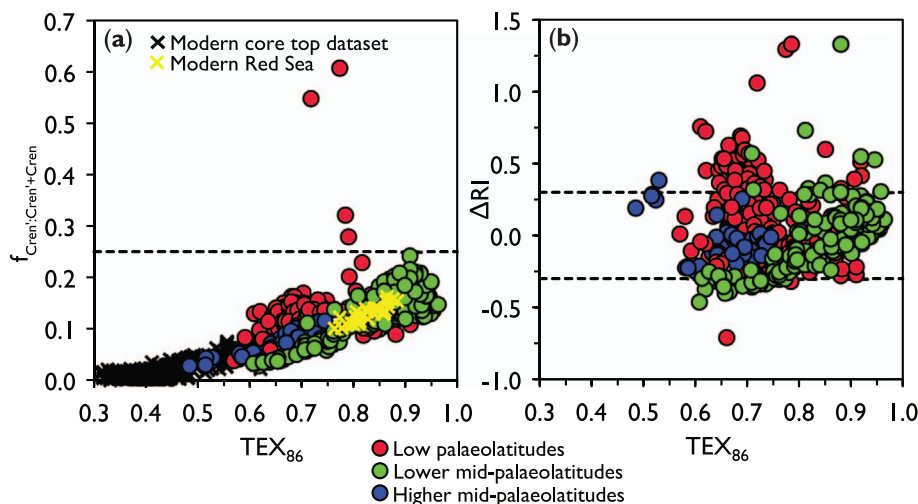
Fig. 5. (a) Proportion of Cren' relative to Cren, f_{Cren':Cren'+Cren} in Cretaceous sediments, categorized by palaeolatitude. f_{Cren':Cren'+Cren} values for the modern core-top dataset, including the Red Sea, are also shown. (b) \Delta RI values for Cretaceous samples, categorized by palaeolatitude.
