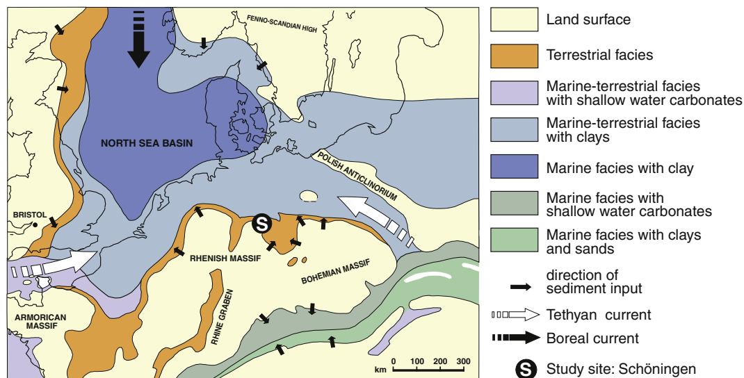
Fig. 1. Palaeogeography of NW Europe during the early Paleogene showing the location of Schöningen. Modified from Riegel et al., 2012.
