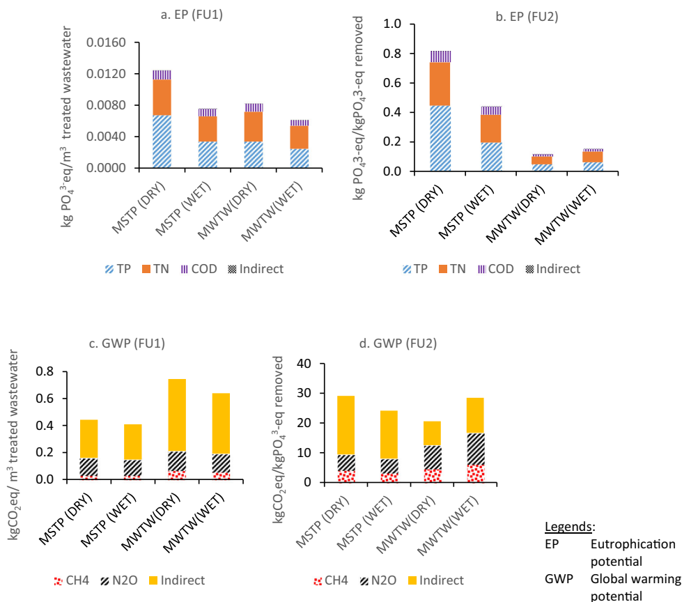
Fig. 5 Comparison of eutrophication potential (EP) and global warming potential (GWP) at Malaysian STP (MSTP) and Millbrook WTW (MWTW) in the dry and wet seasons by using FU1 (per m 3 ) and FU2 (per kgPO 4 3 -eq removed), respectively
