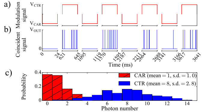
Fig. 4. Dissipative single-photon switching. The raw data: a) The modulation signal applied to the fibre stretcher driving the system between coherent absorption (CAR) and transmission regimes (CTR). b) The coincident photon detection signal between SPD-c & SPD-h and SPD-d & SPD-h. ((a) and (b) share the x-axis, of which broken parts correspond to phase stabilization periods.) c) The coincidence counts distribution of coherent absorption (red) and transmission (blue) cycles.
