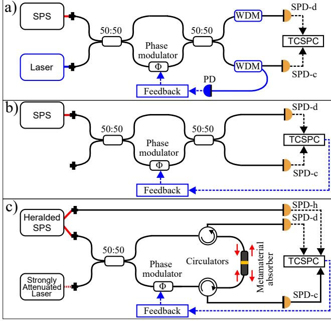
Fig. 1. Stabilization of coherent optical fibre networks operating at the single-photon level. a) A MZI consisting of a single-photon source (SPS), 50:50 BSs and a phase modulator as an example network. Time-correlated single-photon counting (TCSPC) module processes signals of single-photon detectors (SPD). In conventional stabilization schemes (highlighted in blue), a laser light sent through the coherent network is separated and measured by a multiplexer (e.g. WDM) and a photodetector (PD), respectively. b) Optical fibre networks stabilized with single-photons: TCSPC output is used as an input of the feedback system. c) Single-photon absorption control and switching experiment setup, where the second BS is substituted with a metamaterial absorber.
