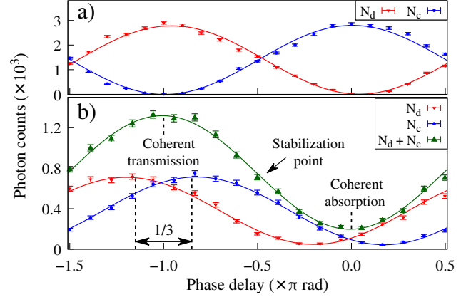
Fig. 3. Single-photon manipulation in coherent optical fibre networks stabilized by single-photons. a) Single-photon interference in a fully-fiberized MZI (Fig. 1(b)). Out-of-phase oscillation of N_c and N_d is in a good agreement with Eqs. (1,2). b) Single-photon absorption control with a CPA (Fig. 1(c)). As each point corresponds to a single measurement, the dispersion is defined by the Poisson distribution.
