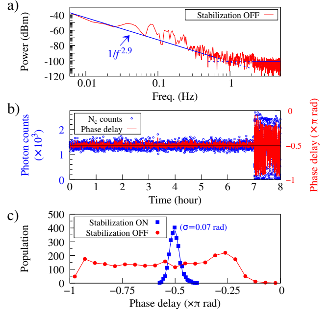
Fig. 2. Long-term phase stabilization in a fully-fiberized MZI. a) The noise spectral density of phase fluctuations of the unstabilized system, measured by sending a CW-laser of \mu\text{W} power through the same interferometer, decreases by 1/f^{2.9} until 1 Hz beyond which a broadband noise dominates. b) The long-term phase stabilization where the system is stabilized for 7 hours, followed by another 7 hours without stabilization (only one hour is shown). Each blue circle corresponds to single-photon counts with the red line being the corresponding phase delay retrieved from these counts. The black line represents the stabilization point. c) The corresponding phase distributions for the stabilized (blue) and unstabilized (red) periods, where the blue line is the Gaussian fit curve.
