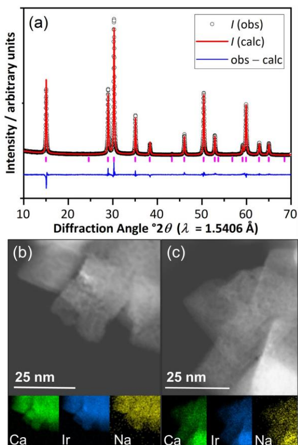
Figure 1: (a) Rietveld fit to powder XRD of (\text{Ca}_{0.70}\text{Na}_{0.24})_2\text{Ir}_2\text{O}_6 \cdot \text{H}_2\text{O} Fd\bar{3}m , a = 10.23978(5) \text{ Å} , and (b) and (c) STEM images and EDXA maps of two regions of the material showing homogeneity of elemental distribution.
