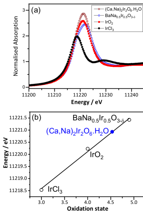
Figure 2: (a) Room temperature Ir L_{III} -edge XANES spectra of (\text{Ca}_{0.70}\text{Na}_{0.24})_2\text{Ir}_2\text{O}_6 \cdot \text{H}_2\text{O} and reference materials and (b) oxidation state calibration graph, with the white line maximum used.
