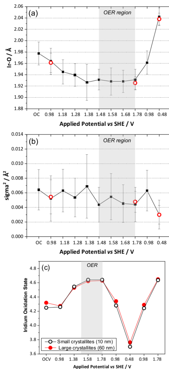
Figure 4: Plots of EXAFS-derived (a) Ir-O distance, (b) Debye-Waller factor, and (c) comparison of Ir oxidation state from XANES for two particles sizes of (\text{Ca}_{0.70}\text{Na}_{0.24})_2\text{Ir}_2\text{O}_6 \cdot \text{H}_2\text{O} showing also recyclability upon a second oxidation sweep. In (a) and (b) the red circles are repeated measurements from a second electrode on a later experimental run to check reproducibility. OC = open circuit.
