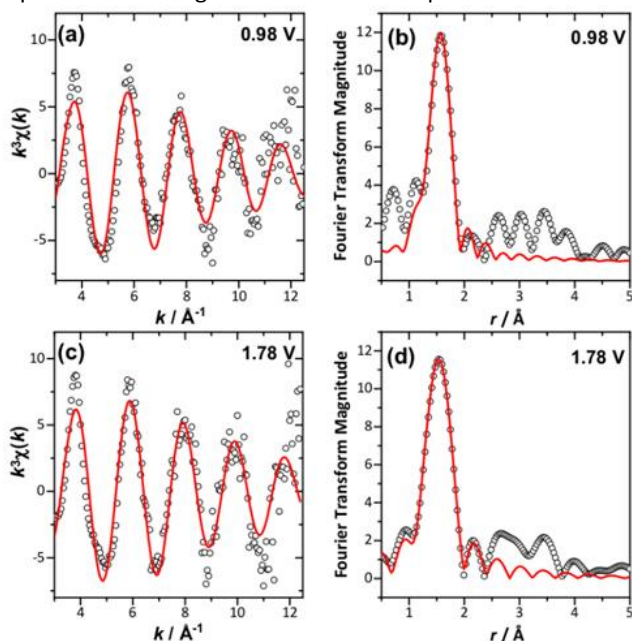
Figure 3: Single-shell fits of k^3 -weighted EXAFS (left), with Fourier transforms (right) from (\text{Ca}_{0.70}\text{Na}_{0.24})_2\text{Ir}_2\text{O}_6 \cdot \text{H}_2\text{O} at (a) and (b) 0.98 V and (c) and (d) maximum applied potential.
