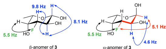
Figure 2. 1 H NMR analysis of 3 in D 2 O
