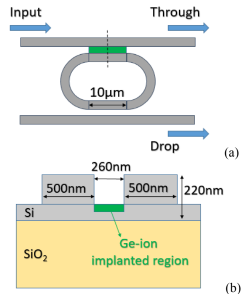
Fig. 1: (a) A schematic of a racetrack resonator and (b) a cross-sectional view of the device.
