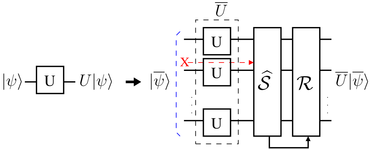
FIGURE 14. General transversal single-qubit gate.
