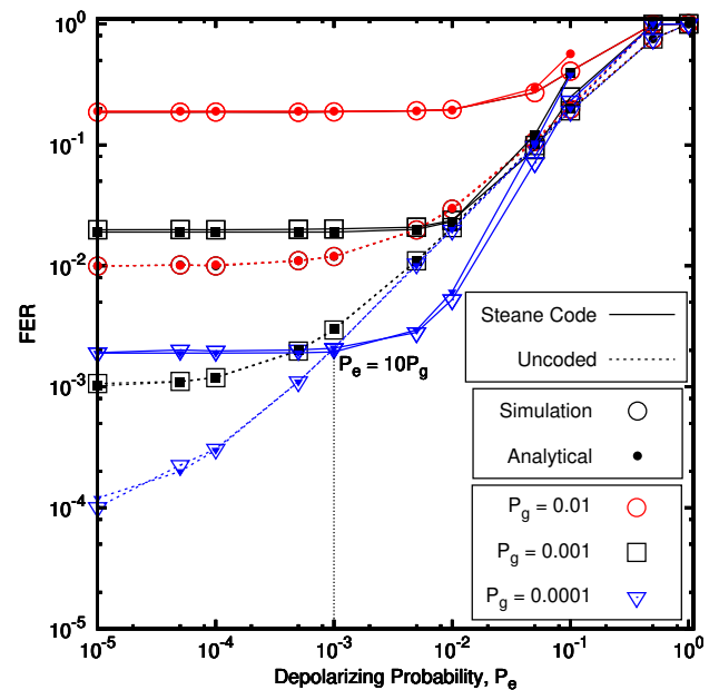
FIGURE 22. FER of a transversal CNOT gate vs. the depolarizing probability P_e parameterized by various gate error probabilities P_g .
