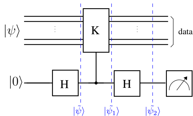
FIGURE 7. Measurement of single stabilizer operator K .
