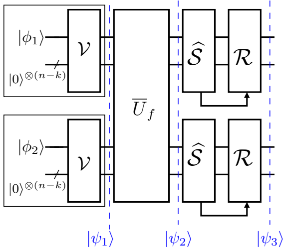
FIGURE 15. General transversal CNOT gate \bar{U}_f scheme.
