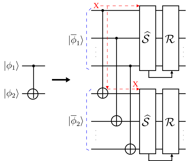
FIGURE 1. Transversal CNOT gate.
