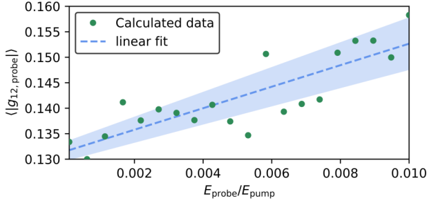
FIG. 7. Average probe coherence for 1 m of ANDi PCF with \Delta\beta_1 = 0 ps/m as a function of the ratio of the probe energy to the pump energy. The pulse durations were constant at 7 ps and the pump energy was held constant at 60 nJ. The shaded region shows the confidence interval of the linear fit to one standard deviation.
