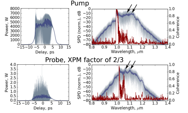
FIG. 3. Orthogonally polarized pump and probe ensembles after co-propagating in silica ANDi PCF with \Delta\beta_1 = 0 ps/m. Left column: time-domain. Right column: normalized spectral power density (SPD, left y-axis) and coherence data (red trace, right y-axis). Blue traces show the ensemble average and fine gray lines show the individual shots. Top: Pump (60 nJ, 7 ps). Bottom: Probe (5 pJ, 7 ps). The arrows mark the two most energetic Stokes peaks.
