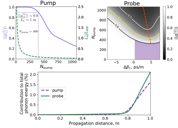
FIG. 6. Top left: Average pump coherence (left y -axis, purple solid line) and L_R^*/L_{WB} (right y -axis, green dashed line) as a function of N_{\text{pump}} for a 1 m length of PCF. Top right: Average probe coherence as a function of N_{\text{pump}} and \Delta\beta_1 for a 1 m length of PCF. The red dashed line in the right-hand plot shows where \langle |g_{12}^{(1)}| \rangle is minimized for a given N_{\text{pump}} . The purple region shows where L_{c \text{ probe}} is shorter than L_{c \text{ pump}} , and therefore where the decoherence for the probe occurs at a higher rate than the pump. Bottom: Energy transferred from the pump and probe pulses to the phonon field as a function of propagation distance ( N_{\text{pump}} = 900 and \Delta\beta_1 = 0 ps/m).
