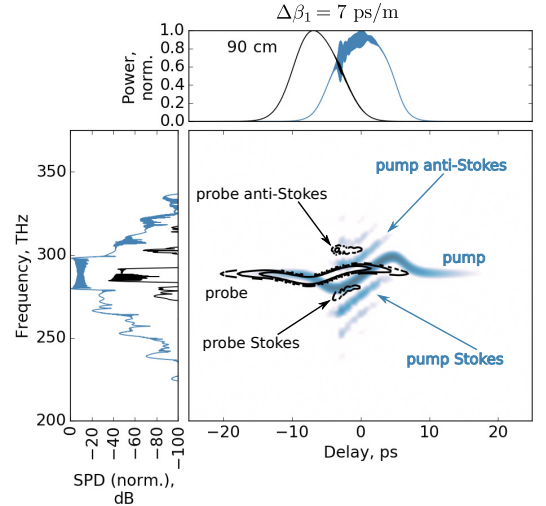
FIG. 4. Spectrograms of orthogonally polarized pump (blue colormap) and probe (black contour) with the same initial central wavelength (1040 nm, 288 THz) after propagating through 90 cm of ANDi PCF with \Delta\beta_1 = 7 ps/m. The spectrograms are normalized to the peak of the pump pulse (-70 to 0 dB).
