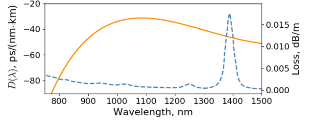
FIG. 2. Left axis (orange solid): Dispersion curve for the silica hexagonal-lattice ANDi PCF. \Lambda = 1.7 \mu\text{m} , and d/\Lambda = 0.3 . Right axis (blue dashed): Loss profile used in the simulations.
