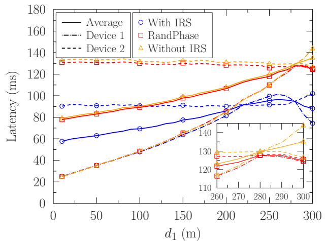
Figure 11: Simulation results of the latency versus the user location in the two-device scenario, where we set d_2 = 280 m, N = 40 , and f_{\text{total}}^e = 50 \times 10^9 cycle/s.
