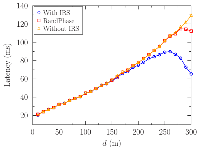
Figure 8: Simulation results of the latency versus the device location in the single-device scenario, where we set N = 40 and f_{\text{total}}^e = 50 \times 10^9 cycle/s.
