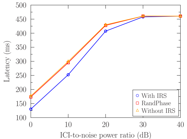
Figure 14: Simulation results of the device-average latency versus the ICI-to-noise ratio. The parameters are set as follows: K = 3 , d = 280 m, \bar{d} = 10 m, r = 10 m, N = 40 , and f_{total}^e = 50 \times 10^9 cycle/s.
