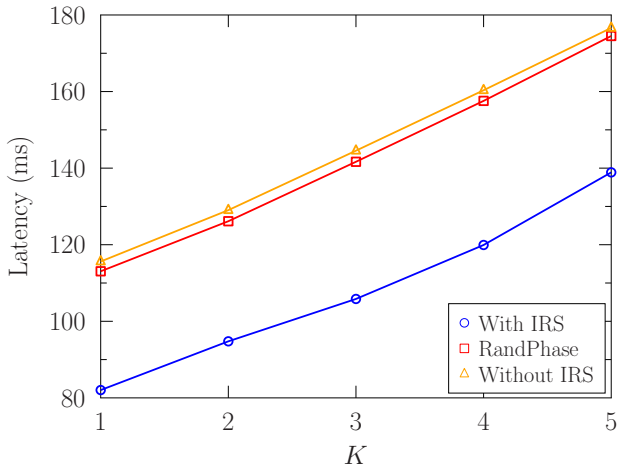
Figure 13: Simulation results of the device-average latency versus the number of devices K . The parameters are set as follows: d = 280 m, \bar{d} = 10 m, r = 10 m, N = 40 , and f_{total}^e = 50 \times 10^9 cycle/s.
