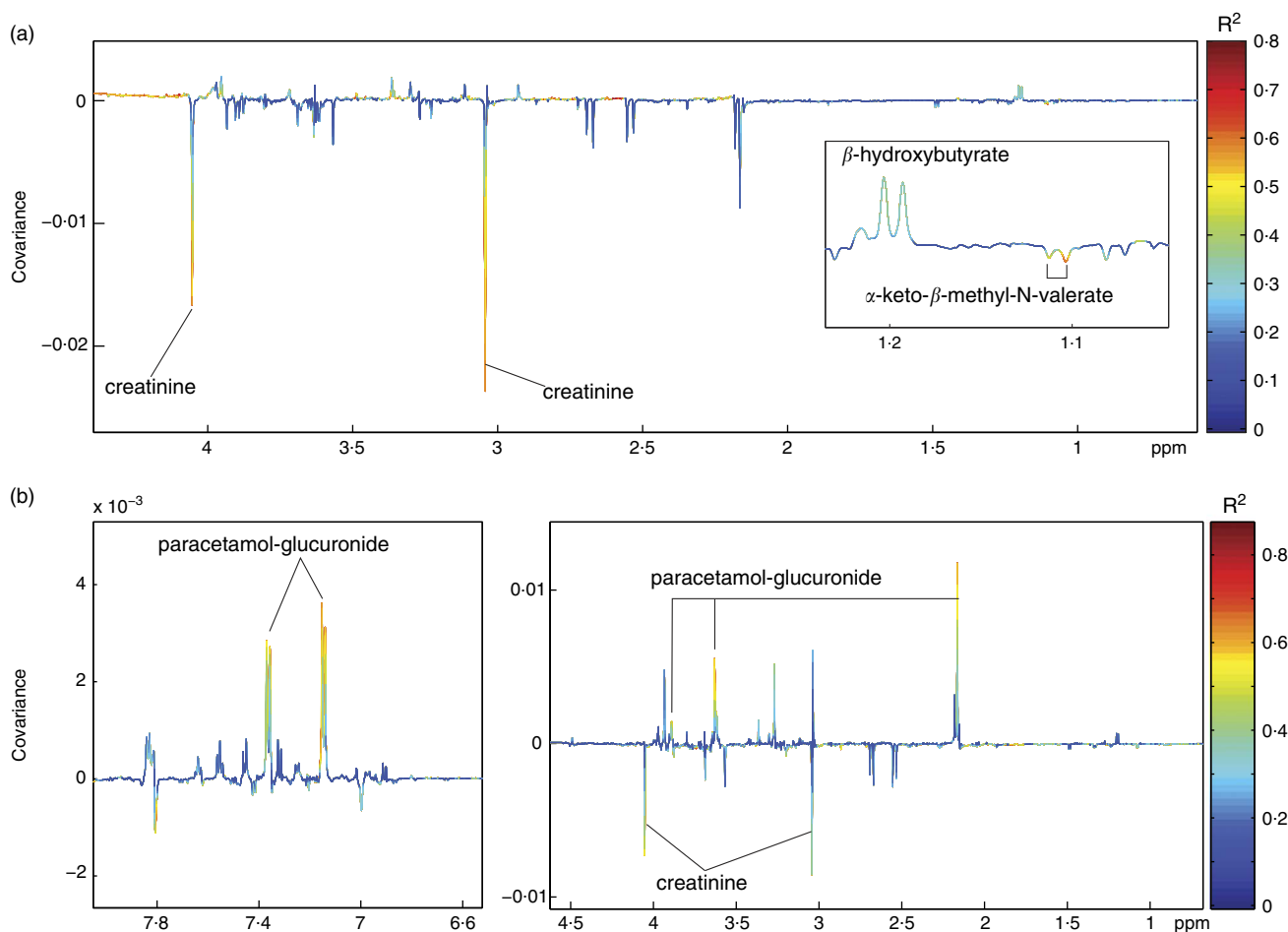
Fig. 10. Orthogonal projection to latent structure models showing metabolic variation associated with fullness following mycoprotein (a) and chicken (b) intake. (a) Colour indicates the correlation of the metabolites with fullness. After mycoprotein intake, creatinine and the deamination product of isoleucine, \alpha -keto- \beta -methyl- N -valerate, were inversely related to fullness and \beta -hydroxybutyrate was positively associated. (b) Significant associations are shown in red. After chicken intake, paracetamol-glucuronide was positively associated with fullness and creatinine was negatively associated.
