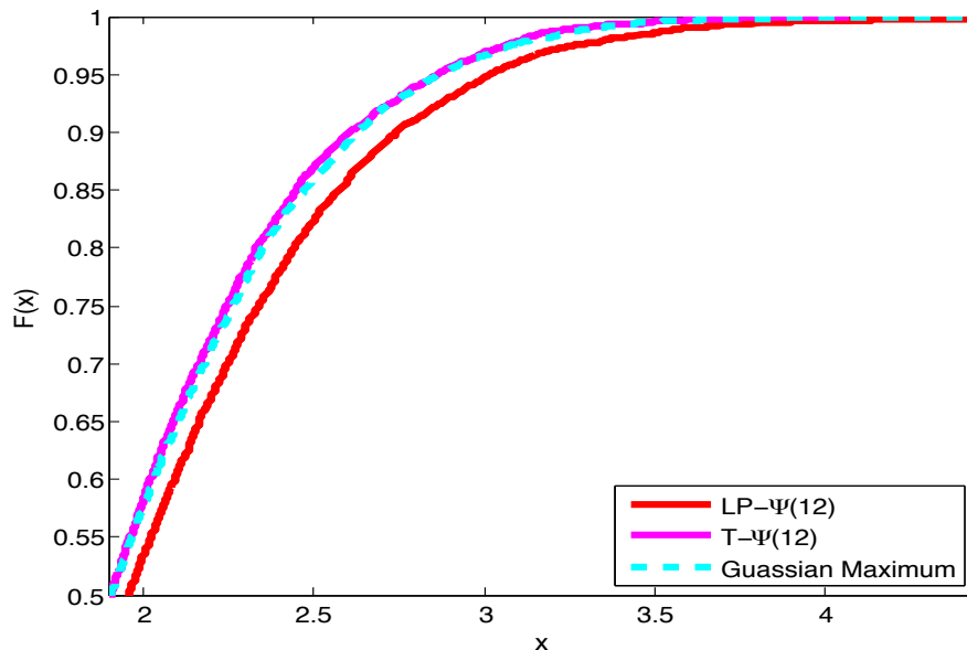
Figure 1: Comparison of the empirical cumulative distributions of LP-\hat{\Psi}(12) , T-\hat{\Psi}(12) and the limiting cumulative distribution with n = 180 and m = 150 . The plot is based on 5000 simulations.
