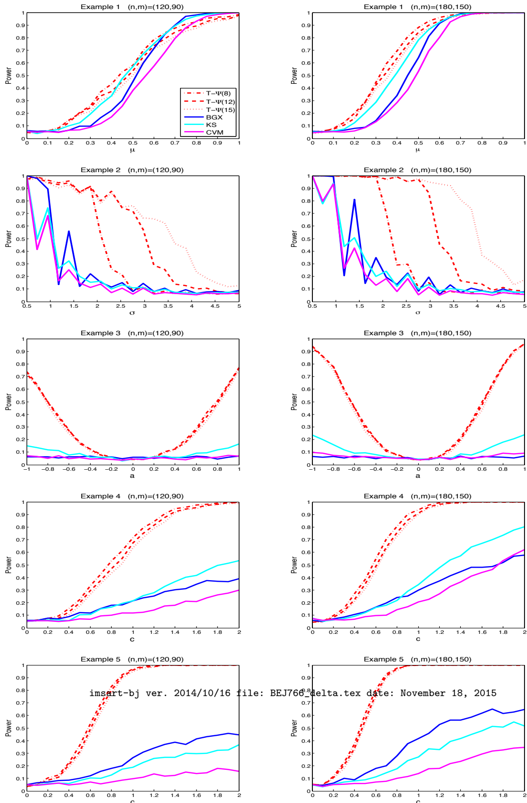
Figure 2: Empirical powers for Examples 1–5 based on 1000 replications with \alpha = 0.05
