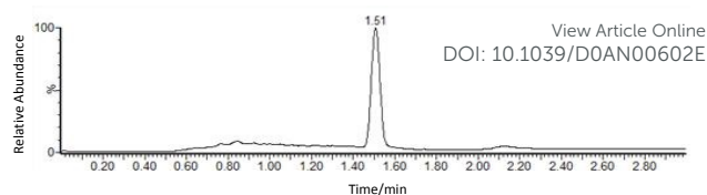
Fig 3 ESI UHPSFC-MS SIM of TPPS at 1 µg/mL (S/N = 161).
