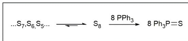
Fig. 1 Derivatization reaction.
