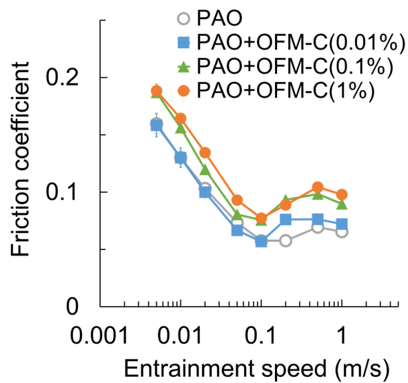
(b) PEEK-steel (50% SRR)
