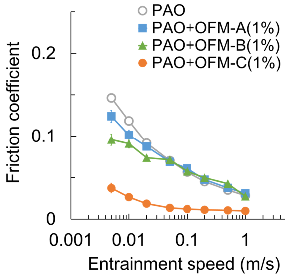
(a) PEEK-PEEK (200% SRR)
