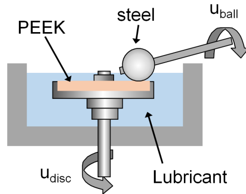
(b) PEEK-steel
