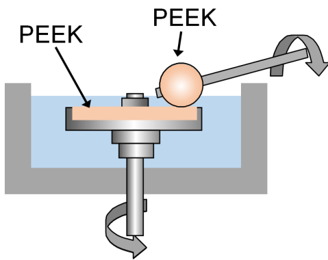
(c) PEEK-PEEK
