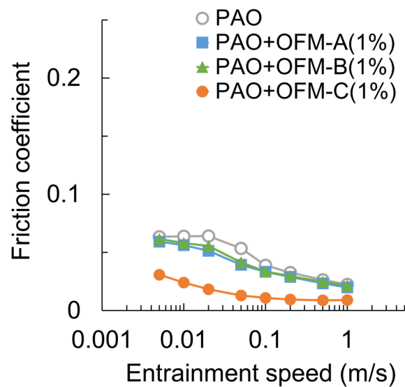
(b) PEEK-steel (50% SRR)
