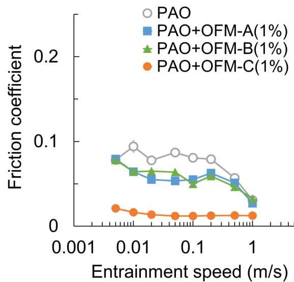
(a) PEEK-steel (200% SRR)
