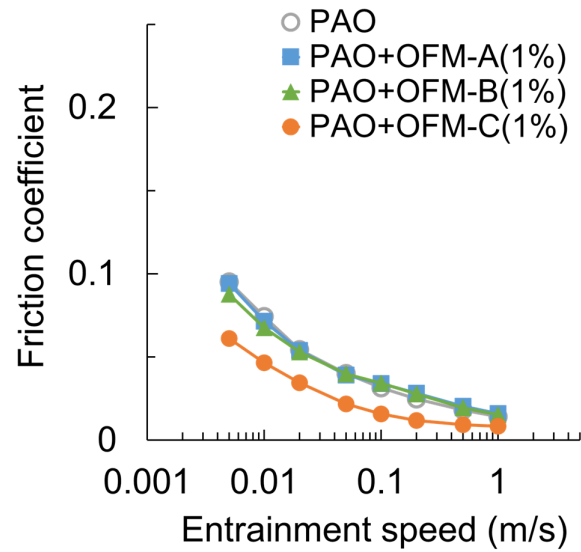
(b) PEEK-PEEK (50% SRR)
