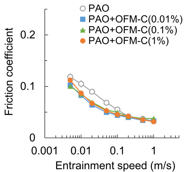
(a) PEEK-steel (200% SRR)
