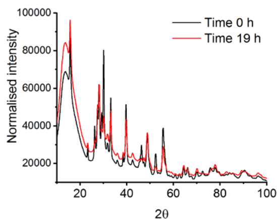
Figure 3: XRD patterns at time 0 h and time 19 h after milling La 2 O 3 and Mn 2 O 3 with a PMMA vibrational mill
