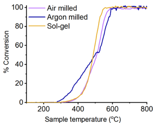
Figure 10: Light-off curve of the percentage of deN 2 O to N 2 over LaMnO 3 catalysts synthesised by mechanochemistry and sol-gel synthesised with 0.5% N 2 O/He at 30 mL min -1 with a pre-treatment of He at 30 mL min -1
