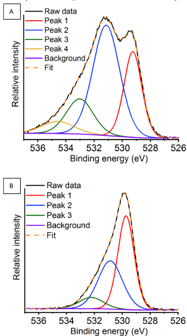
Figure 13: O1s region for the argon milled catalyst showing the deconvoluted peaks at (A) RT and (B) 600 °C under a N 2 O atmosphere
