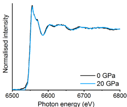
Figure 4: In situ high pressure EDE spectra at 0 GPa and 20 GPa on \text{La}_2\text{O}_3 and \text{Mn}_2\text{O}_3 mixture after high energy ball milling for 30 min
