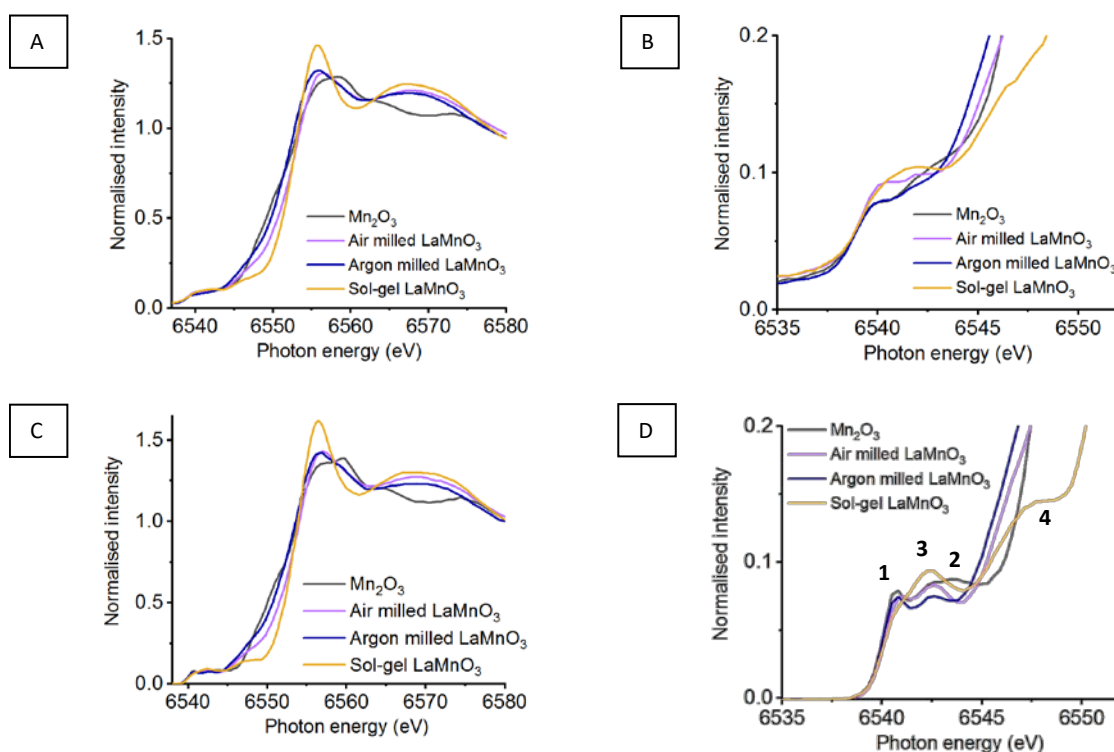
Figure 7: (A) Mn K-edge XANES with (B) highlighted pre-edge region compared to (C) HERFD-XANES with (D) highlighted pre-edge region of mechanochemical synthesis of \text{LaMnO}_3 within air and argon environments compared to sol-gel \text{LaMnO}_3 and precursor \text{Mn}_2\text{O}_3
