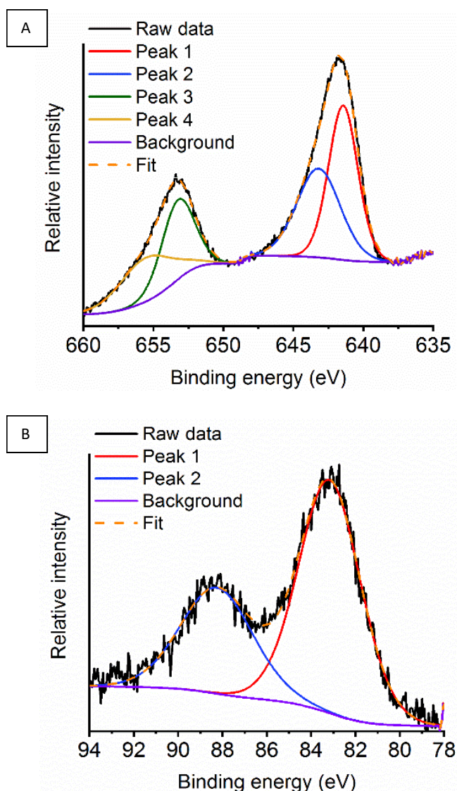
Figure 11: (A) Mn2p region and (B) Mn3s region for the argon milled catalyst at RT under a N 2 O atmosphere
