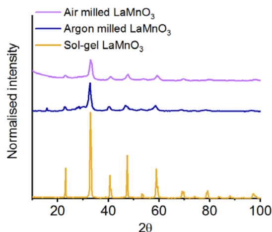
Figure 5: XRD patterns \text{LaMnO}_3 mechanochemically synthesised 4 h under atmospheric and inert (argon) conditions compared to the sol-gel synthesised perovskite
