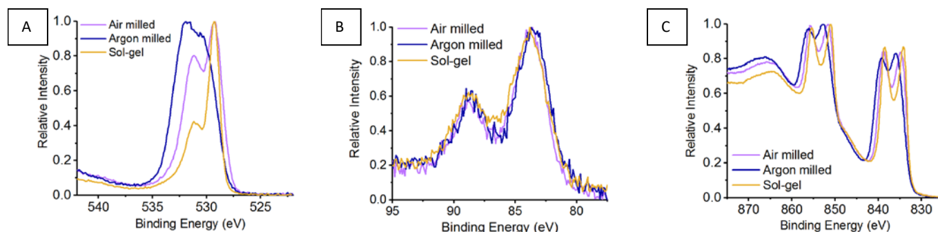
Figure 9: XPS in the (A) O1s, (B) Mn3s and (C) La3d region for LaMnO 3 synthesised by sol-gel and mechanochemistry with air and argon environments
