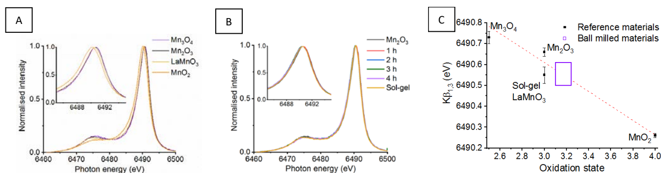
Figure 2: (A) Mn K \beta XES mainlines for Mn reference oxides and sol-gel synthesised LaMnO 3 with (B) 'time-slices' during the mechanochemical synthesis of LaMnO 3 (C) presents the K \beta_{1,3} max as a function of oxidation state, with a line of best fit calculated from the reference materials and used to calculate the oxidation state of the ball milled materials 11
