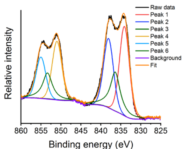
Figure 12: La3d XPS region for the argon milled catalyst showing the deconvoluted peaks at RT under a N 2 O atmosphere
