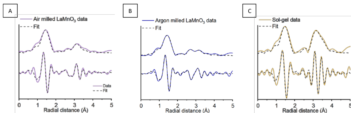
Figure 6: Mn K-edge EXAFS data of \text{Mn}_2\text{O}_3 and after 4 h of milling in atmospheric and inert milling conditions showing the magnitude and imaginary components of the k^2 -weighted FT data and fits compared to sol-gel synthesised \text{LaMnO}_3
