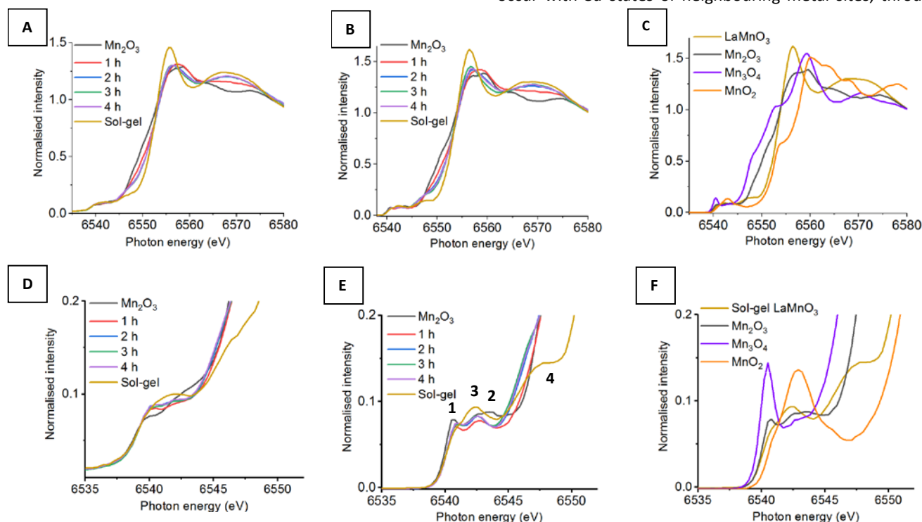
Figure 1: (A) XAS Mn K-edge XANES compared to (B) HERFD-XANES of time-slices during the mechanochemical synthesis of LaMnO 3 compared to (C) reference Mn (II), (III), (IV) oxides and sol-gel synthesised LaMnO 3 with (D-F) their respective highlighted pre-edge region
