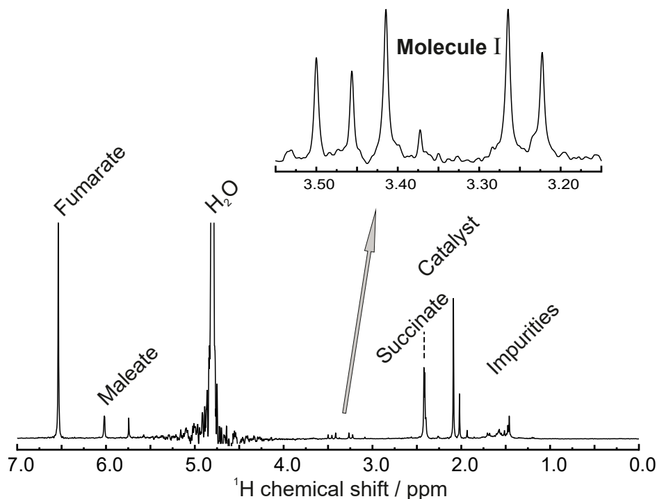
Figure A1. Full ^1\text{H} NMR spectrum (400 MHz) of the reaction solution after hydrogenation. Apart from I , the solution contains several other substances, including fumarate, succinate and maleate.
