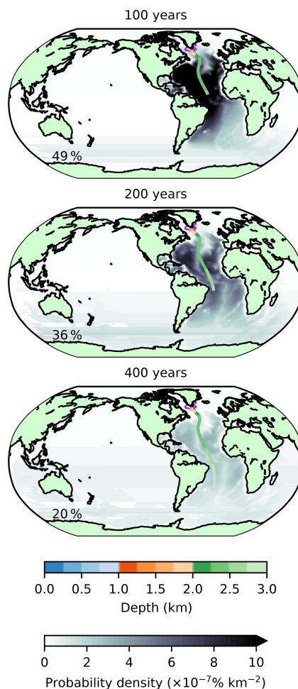
Figure 13. As in Fig. 6 but for subpolar-outcropping model NADW and times of 100, 200, and 400 years.
