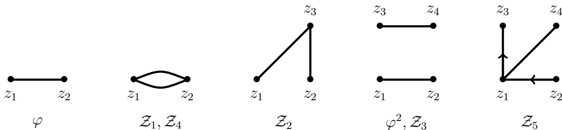
Figure 1: Graphs representing the genus-two modular graph functions \varphi , \mathcal{Z}_i and \varphi^2 where each line represents the Green function \mathcal{G} but presence of derivatives on \mathcal{G} in \mathcal{Z}_5 and the structure of the Abelian differentials is not exhibited. The arrows on two of the lines in \mathcal{Z}_5 indicate the derivatives \partial_1 and \bar{\partial}_1 on \mathcal{G} .
