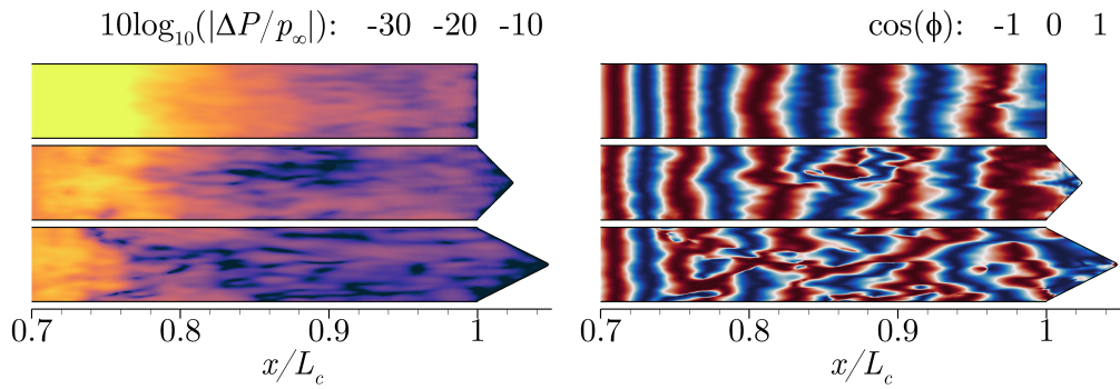
FIGURE 12. Surface contour maps of the Fourier transform of the wall pressure jump at the tonal frequency fL_c/a_\infty = 3.9 : (a) the magnitude in log scale and (b) the phase distribution. The reference phase \phi_{\text{ref}} is the spanwise averaged value at the transition location ( x/L_c = 0.72 ).
