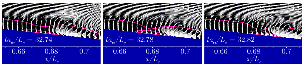
FIGURE 7. Close-up on the velocity vector field near the LSB detachment in the BTE case. Snapshots are synchronised with the ones in figure 6.
