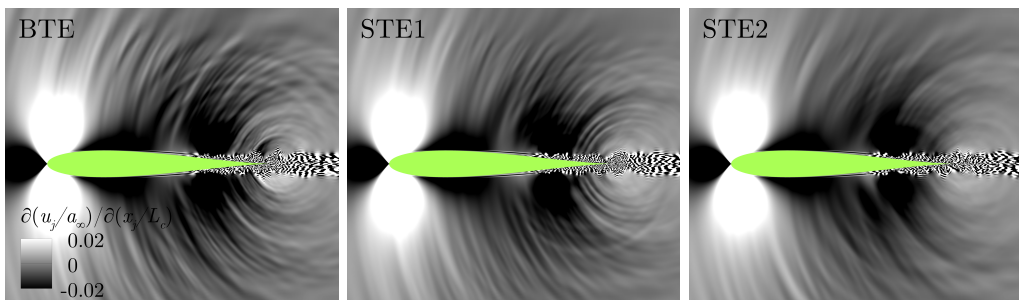
FIGURE 9. Contour map of the divergence of velocity \partial(u_j/a_\infty)/\partial(x_j/L_c) on a mid-span plane comparing the BTE, STE1 and STE2 cases.
