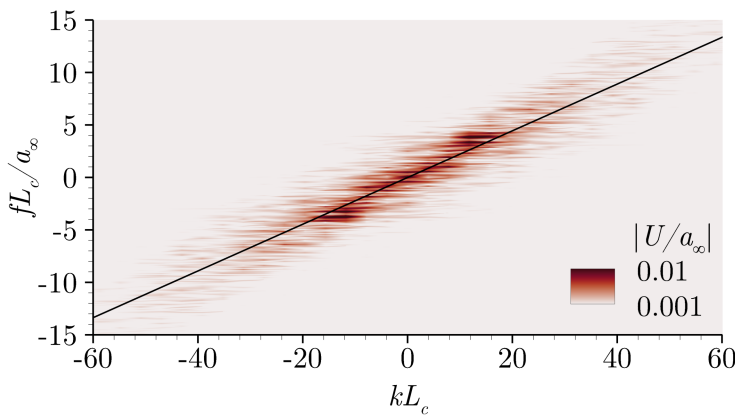
FIGURE 5. A wavenumber-frequency spectrum of the streamwise velocity fluctuation (the magnitude of the Fourier transform) extracted on a mid-span plane along a path-line displaced from the wall by about 20% of the boundary layer thickness at the TE in the BTE case. Least square best fit line with a slope of 0.223 is also displayed.
