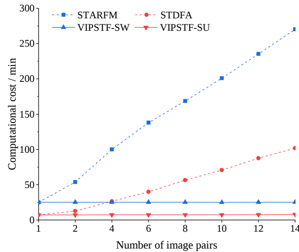
Fig. 12. Computational costs of the methods for Site 1.
