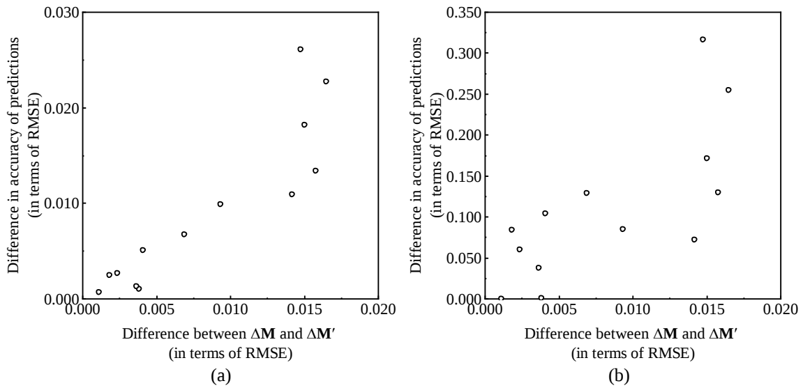
Fig. 11. Scatter plots of reduction in the MODIS level increment (in terms of the difference between \Delta\mathbf{M} and \Delta\mathbf{M}' ) and the corresponding increase of prediction accuracy (in terms of RMSE decrease) for Site 1. (a) STARFM and VIPSTF-SW. (b) STDFA and VIPSTF-SU.
