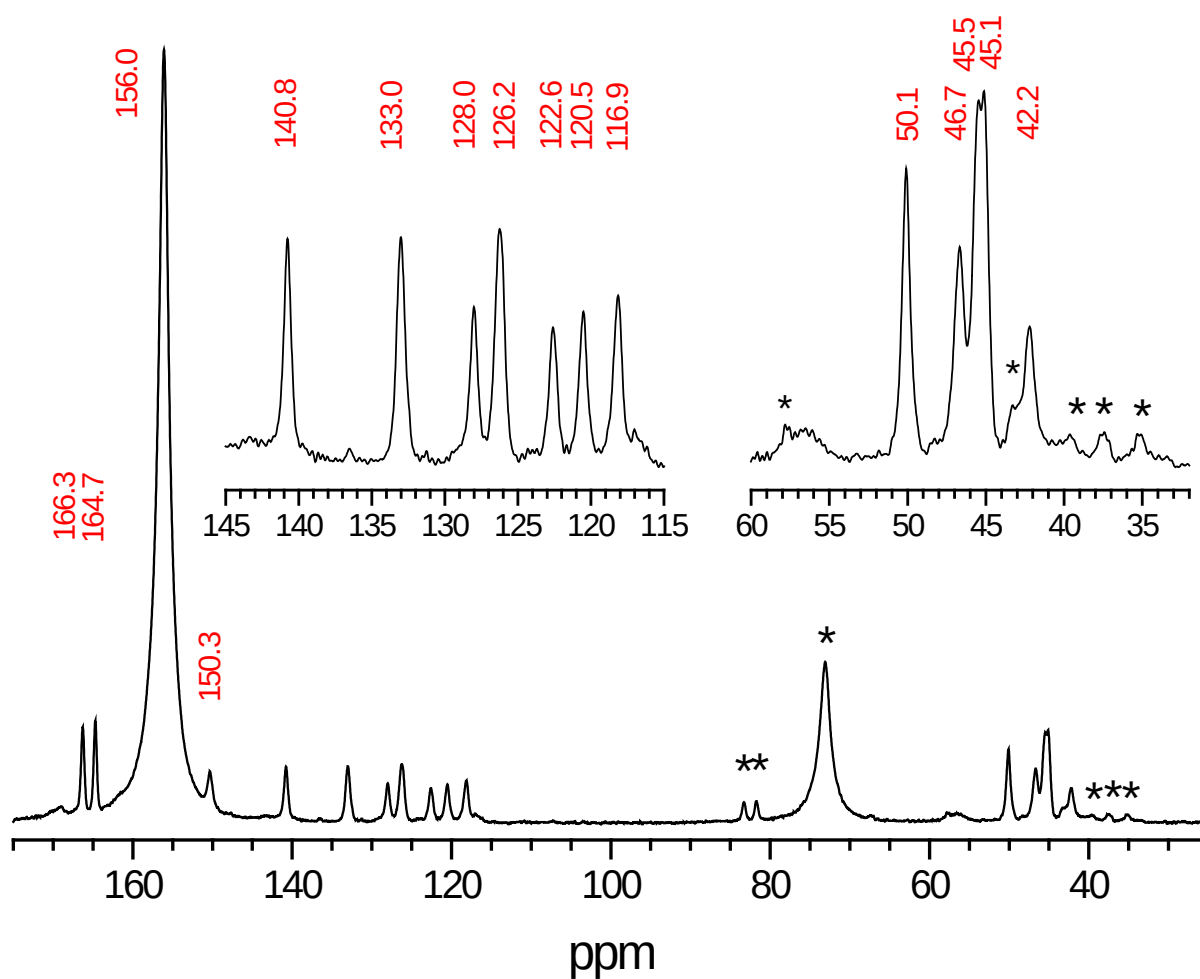
Figure S9. ^{13}\text{C} NMR CP MAS spectrum of 13.\text{Cl}.0.5\text{H}_2\text{O} at 300 K. The asterisks denote spinning sidebands which occur at multiple of sample spinning speed from the main line. The spectrum has been recorded on Bruker AVANCE-2-600 NMR spectrometer with home-built MAS probe for 4x25 mm rotors, ^{13}\text{C} resonance frequency 150.9 MHz, sample spinning rate 12.5 kHz, contact time 2 ms, 1000 scans, relaxation delay 5s.
