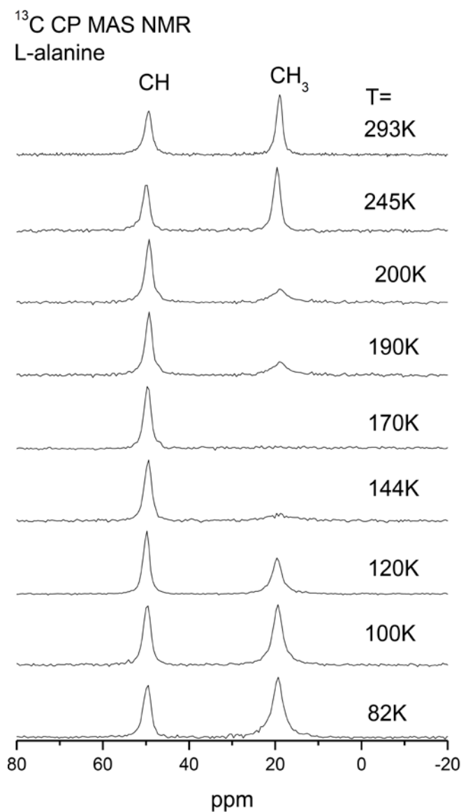
Figure S6. 13 C CP MAS NMR spectra of L-alanine, 13 C isotope enriched in CH and CH 3 positions. The signal of methyl carbons is severely suppressed in a broad temperature range between 100 K to 200 K due to molecular dynamics hindering 1 H to 13 C polarization transfer for methyl carbons (I. Heinmaa, et al S10 ).
