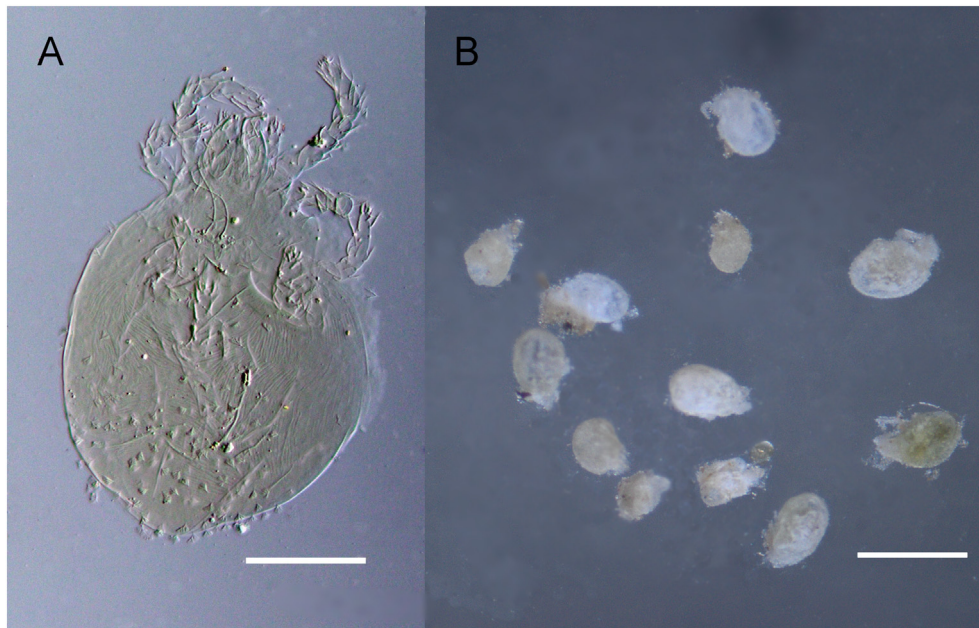
Fig. 3. Nanorchestes nivalis (Trouessart, 1914) from cryoconite holes: A- tritonymph mounted on slide (scalebar 100 \mu\text{m} ), B- nymphs and few adults (scalebar 500 \mu\text{m} ).
