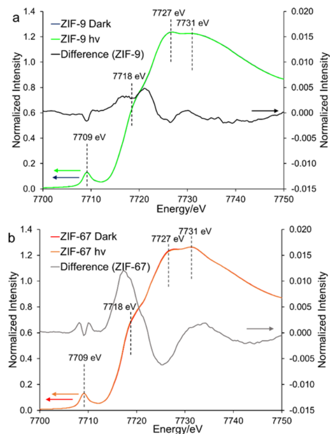
Fig. 3 Normalised XANES data highlighting the difference in the cobalt environment under both 'Dark' and 'hv' conditions for a) ZIF-9 and b) ZIF-67. Note, the similarities between 'Dark' and 'hv' spectra mean they are essentially super-imposed on this scale. Difference spectra are calculated by subtracting the 'Dark' spectra from the 'hv'.
