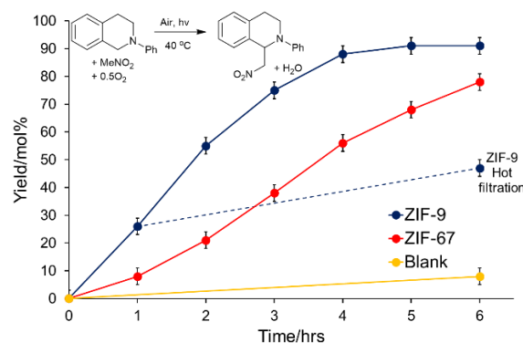
Fig. 6 Kinetic photocatalytic data for the aza-Henry reaction of nitromethane with PhTHIQ to MeNO 2 -PhTHIQ. Reaction conditions: PhTHIQ (0.11 mmol) and catalyst (10 wt%) were stirred in nitromethane (1 mL), with mesitylene as an internal 1 H NMR standard, for 6 h at 40 °C, using a solar simulator with a 515 nm longpass filter. Note: Yields for the ZIF species are higher than for a single measurement as the reaction mixture was opened to the air to sample each hour, refreshing the oxidant.
