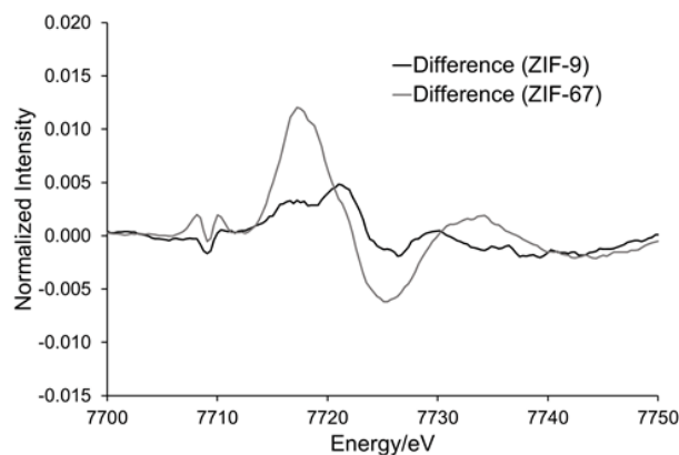
Fig. 5 Comparing the difference spectra of ZIF-9 and ZIF-67 between dark and hv XAS spectra.
