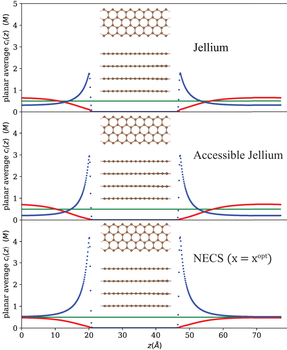
Figure 7: Concentration profiles for Boltzmann-ions with different neutralization schemes for a graphite slab with +2 charge in 0.5 M AB-type electrolyte. Colour scheme: red: positive electrolyte A, blue: negative electrolyte B, green: asymptotic value of 0.5 M concentration. The top and front views of AA-stacked H-terminated graphite slab ( C_{240}H_{32} ) are shown.
