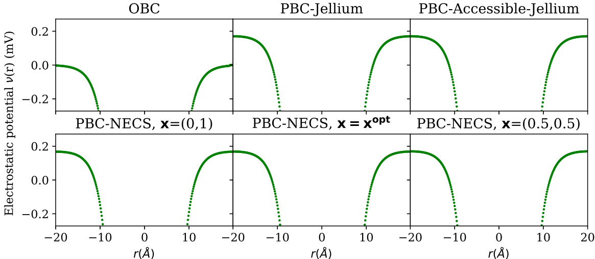
Figure 4: Electrostatic potential in OBCs and with different neutralization schemes in PBCs for a \text{K}^+ ion in 0.5 M \text{A}_2\text{B} electrolyte.
