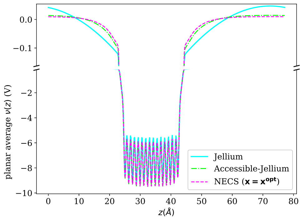
Figure 8: Planar average electrostatic potential with different neutralization schemes for the graphite slab with +2 charge in 0.5 M AB-type electrolyte.
