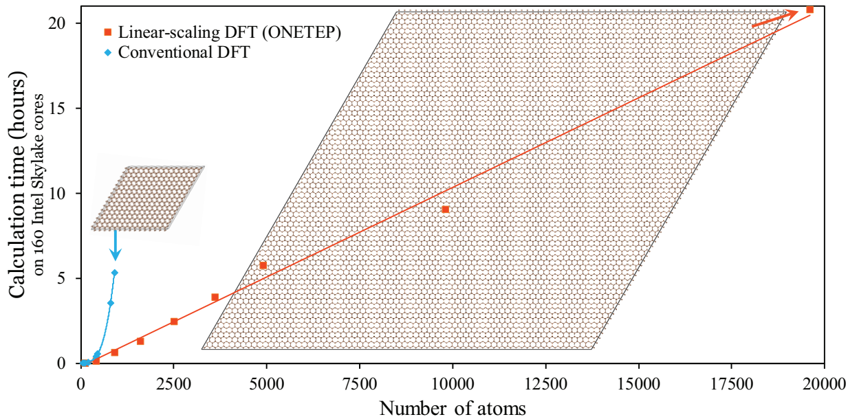
Figure 1: Comparison of the computational time using the ONETEP linear-scaling DFT code against using a conventional plane wave DFT code for periodic graphite systems with varying number of atoms. The computations were performed on the Iridis 5 supercomputer at the University of Southampton on 40 MPI processes with 4 OpenMP threads each (160 cores in total).
