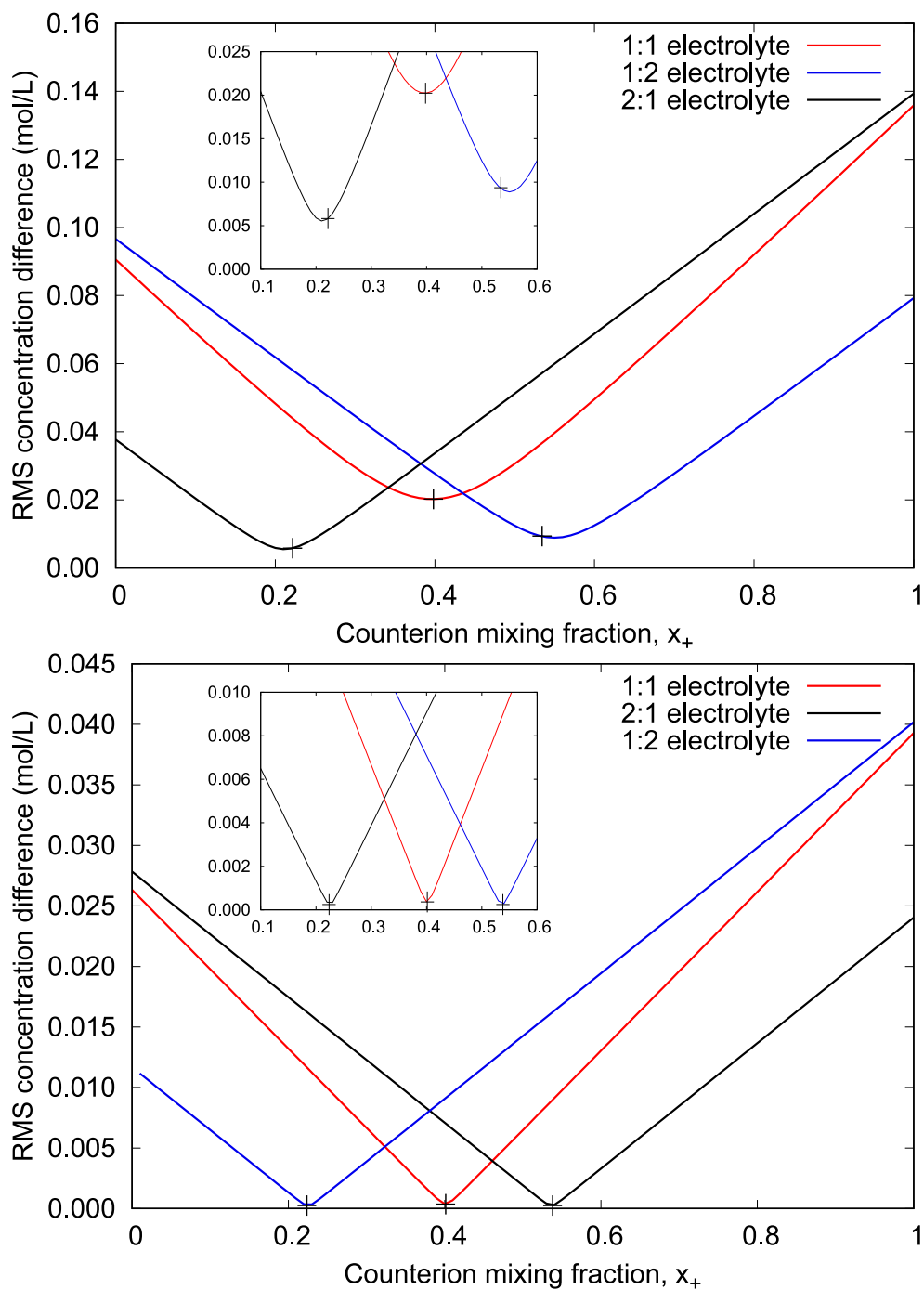
Figure 5: RMS difference in electrolyte ion concentration, relative to the bulk concentration, on the faces of the simulation cell parallel to the graphene sheet (lower is better). Top: smaller cell (17.16 Å × 17.33 Å × 31.75 Å). Bottom: larger cell (17.16 Å × 17.33 Å × 91.75 Å). Crosses denote values obtained from x_+ = x_+^{opt} .
