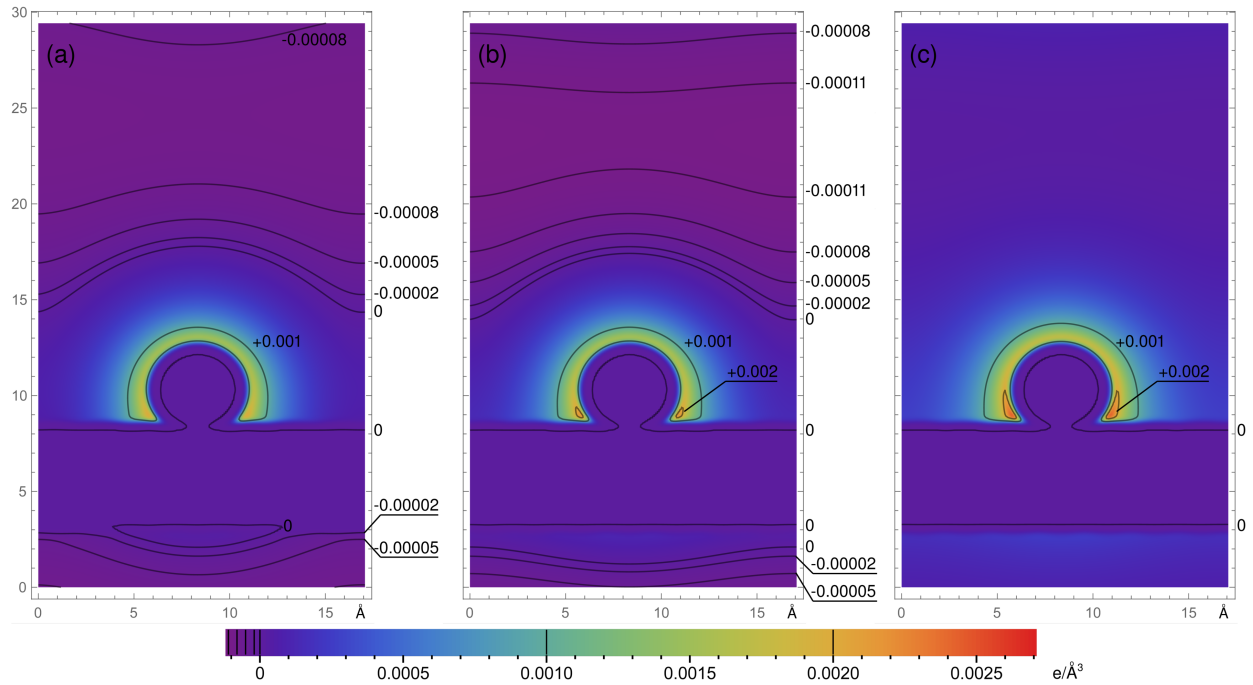
Figure 6: Total charge density ( e/\text{Å}^3 ) of electrolyte in three charge neutralization models: (a) jellium, (b) accessible jellium, (c) NECS with \mathbf{x} = \mathbf{x}^{\text{opt}} in a x-z plane cross-section through the \text{Na}^+ ion. For clarity of presentation anionic charge is shown as positive (warm colors) and the system has been shifted to position the graphene closer to the bottom. The uniform background charge of jellium models is not shown.
