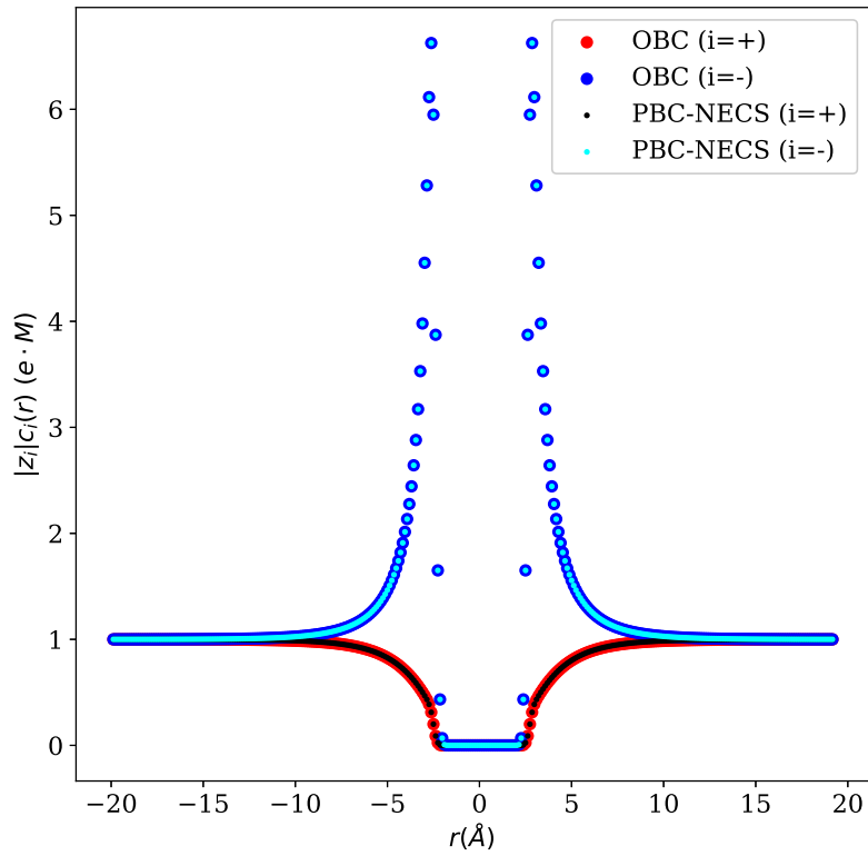
Figure 3: Direct comparison of concentration profiles for positive ( i=+ ) and negative ( i=- ) Boltzmann ions in OBCs with NECS ( \mathbf{x} = \mathbf{x}^{\text{opt}} ) along a straight line containing the \text{K}^+ ion placed at the center of a unit cell in 0.5 M \text{A}_2\text{B} electrolyte.
