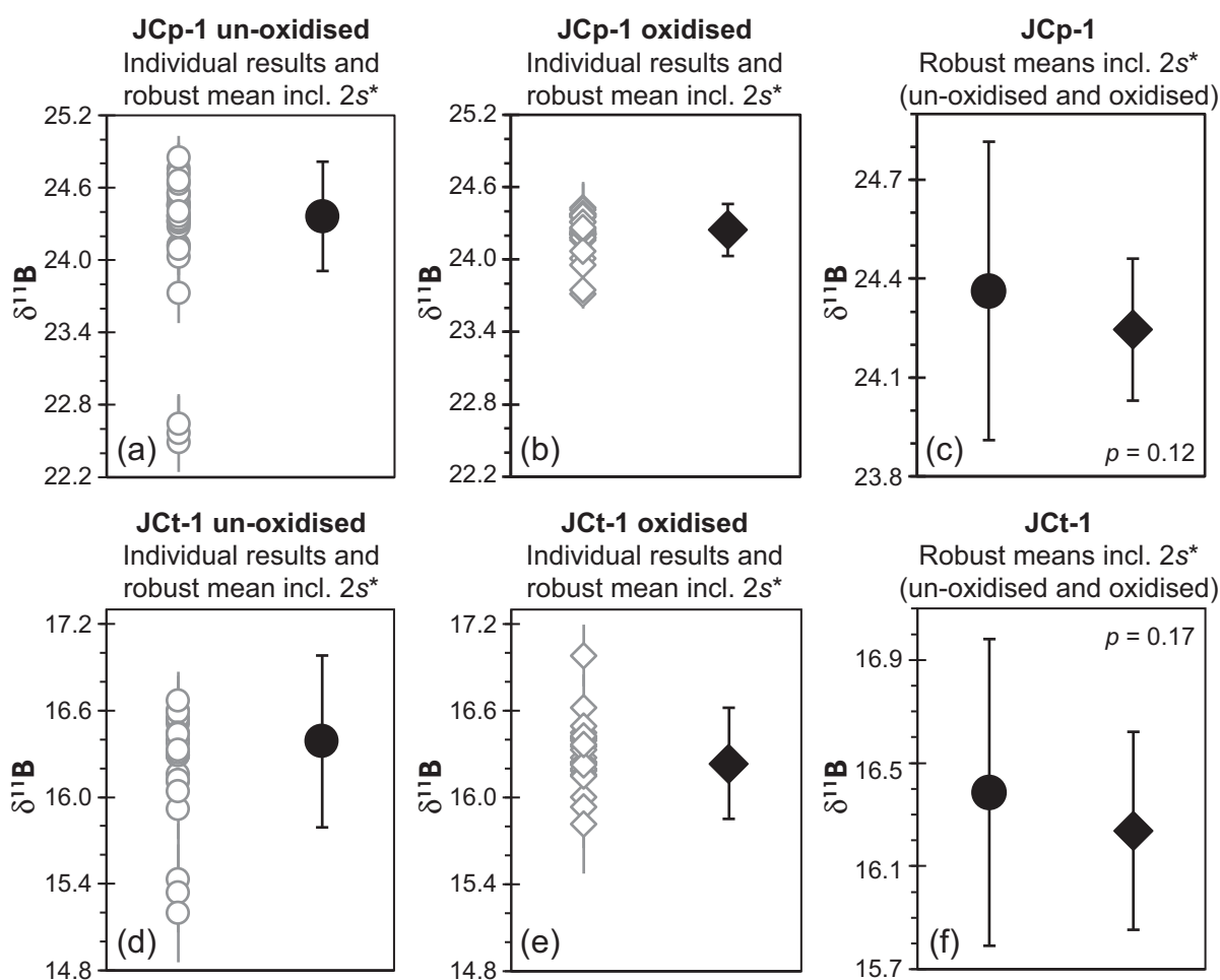
Figure 4. Summary of robust mean \delta^{11}\text{B} and robust standard deviation ( 2s^* ) of (a) un-oxidised and (b) oxidised JCp-1 next to individual data provided by all laboratories, presented in delta notation relative to NIST SRM 951. (c) Comparison of un-oxidised and oxidised robust mean \delta^{11}\text{B} data. (d, e, f) show the same comparisons for JCt-1. Note that panels (a) and (b) and panels (d) and (e) have the same y-axis scale for better comparability, while those for panels (c) and (f) are plotted at finer scale for the presentation of robust means including respective double robust standard deviation. The p -value of a two-sided Student's t -test is also shown for the respective data sets in panels (c) and (f).
