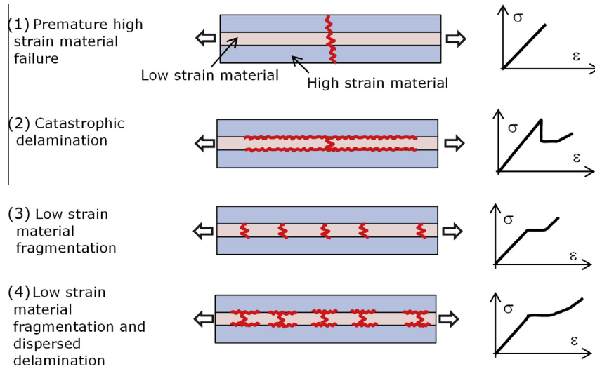
Fig. 2. Different damage scenarios of UD hybrid laminates. (For interpretation of the references to colour in this figure legend, the reader is referred to the web version of this article.)
