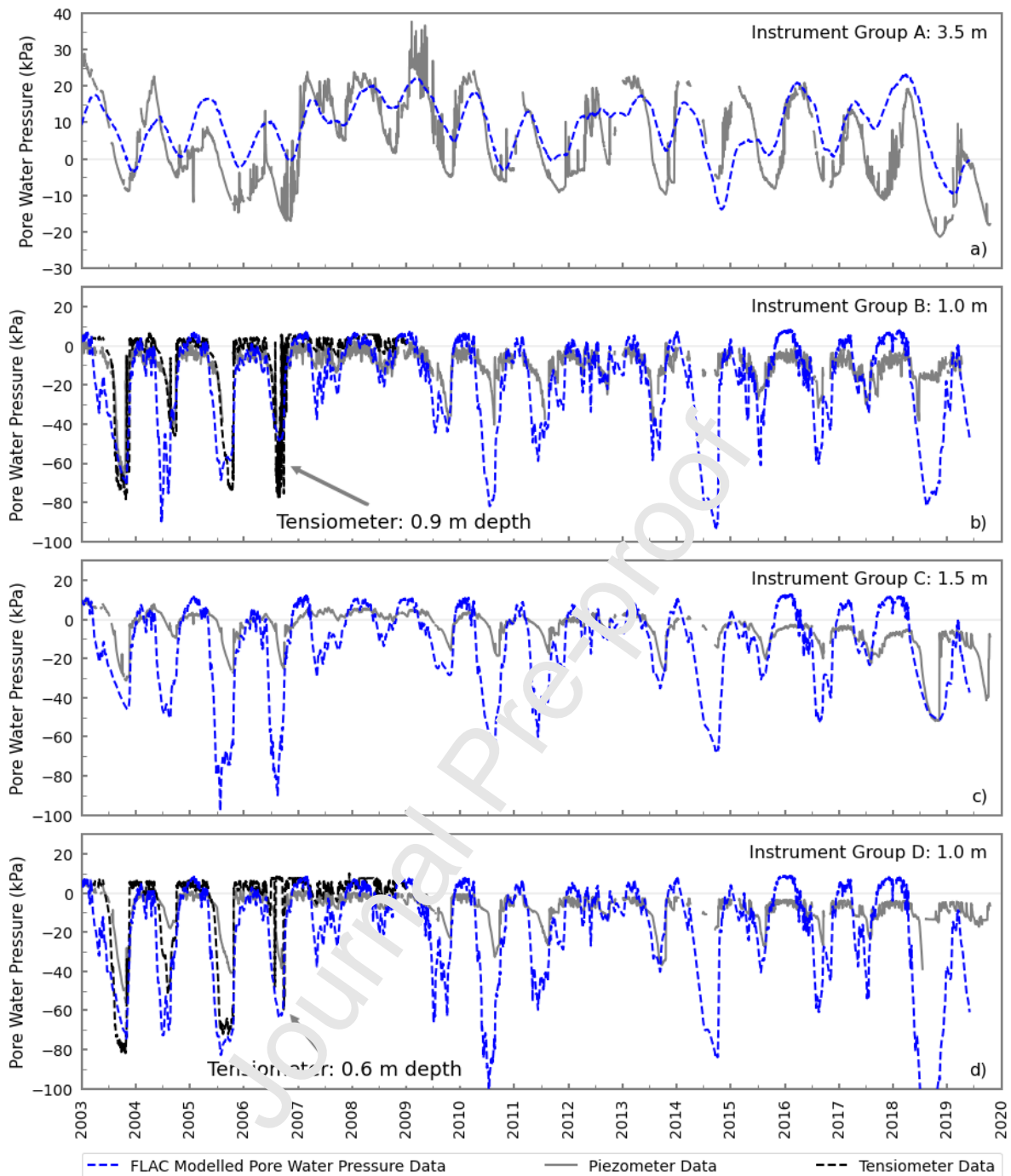
Figure 12: Comparison of hydrogeological response of numerical model and field monitored data for differing piezometers (after Smethurst et al., 2012); a) Group A 3.5 m; b) Group B 1.0 m; c) Group C 1.5 m; d) Group D 1.0 m. Tensiometers at depths indicated.
