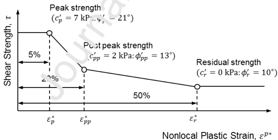
Figure 4: London Clay strain-softening model
