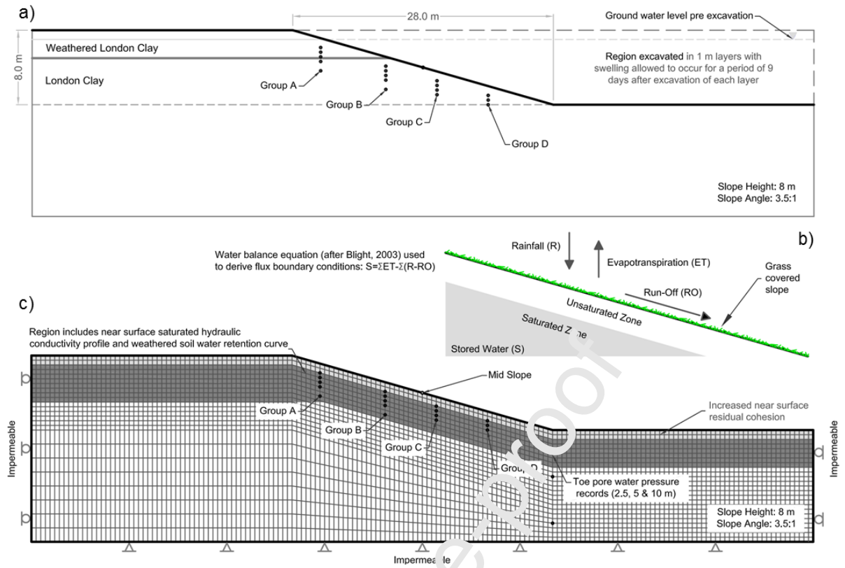
Figure 6: Numerical model configuration (a), schematic boundary conditions (b) and model mesh with monitored history points (c)
