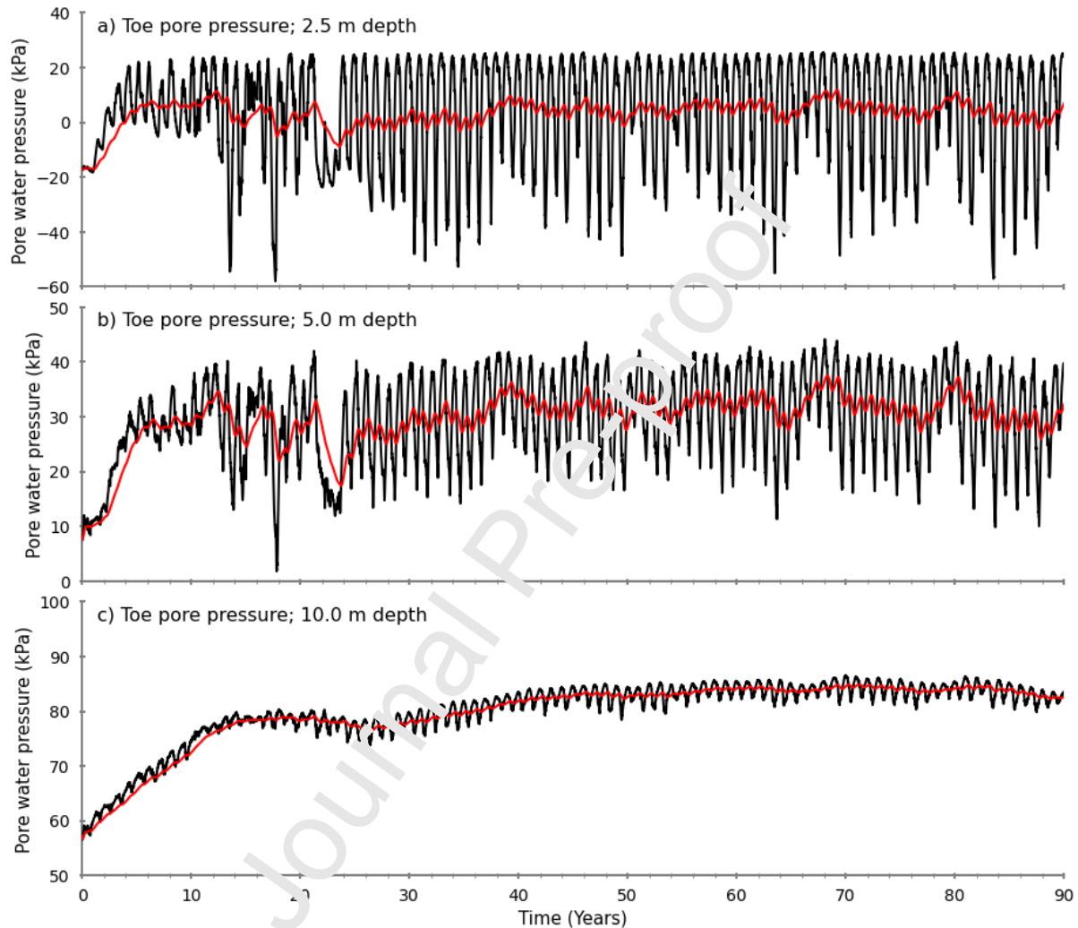
Figure 13: Pore water pressure response post-excavation below toe of slope; a) 2.5 m below toe; b) 5.0 m below toe; c) 10 m below toe.
