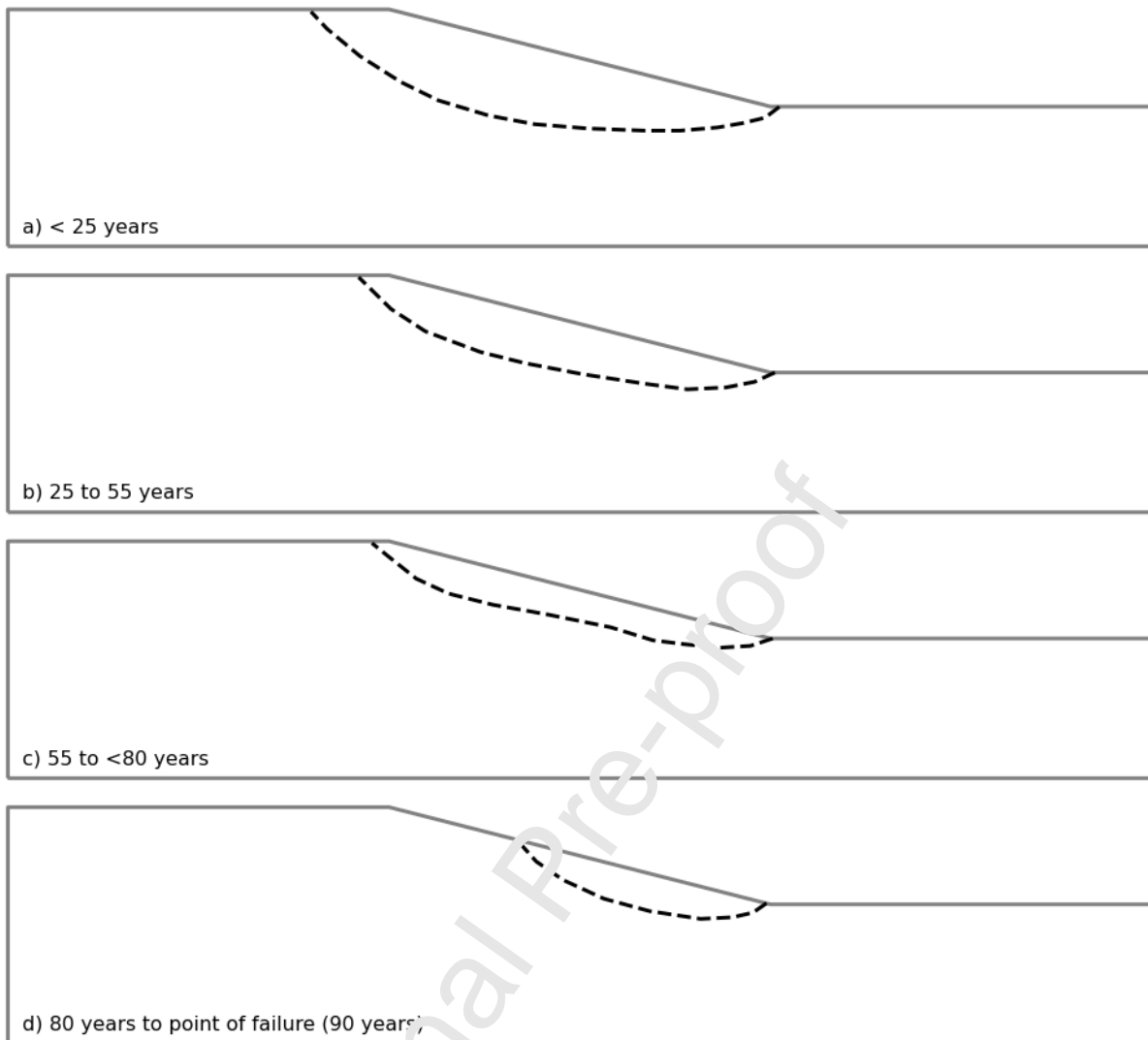
Figure 16: Typical critical failure surfaces for: a) < 25 years; b) 25 to < 55 years; c) 55 to < 80 years and d) 80 years to point of failure.
