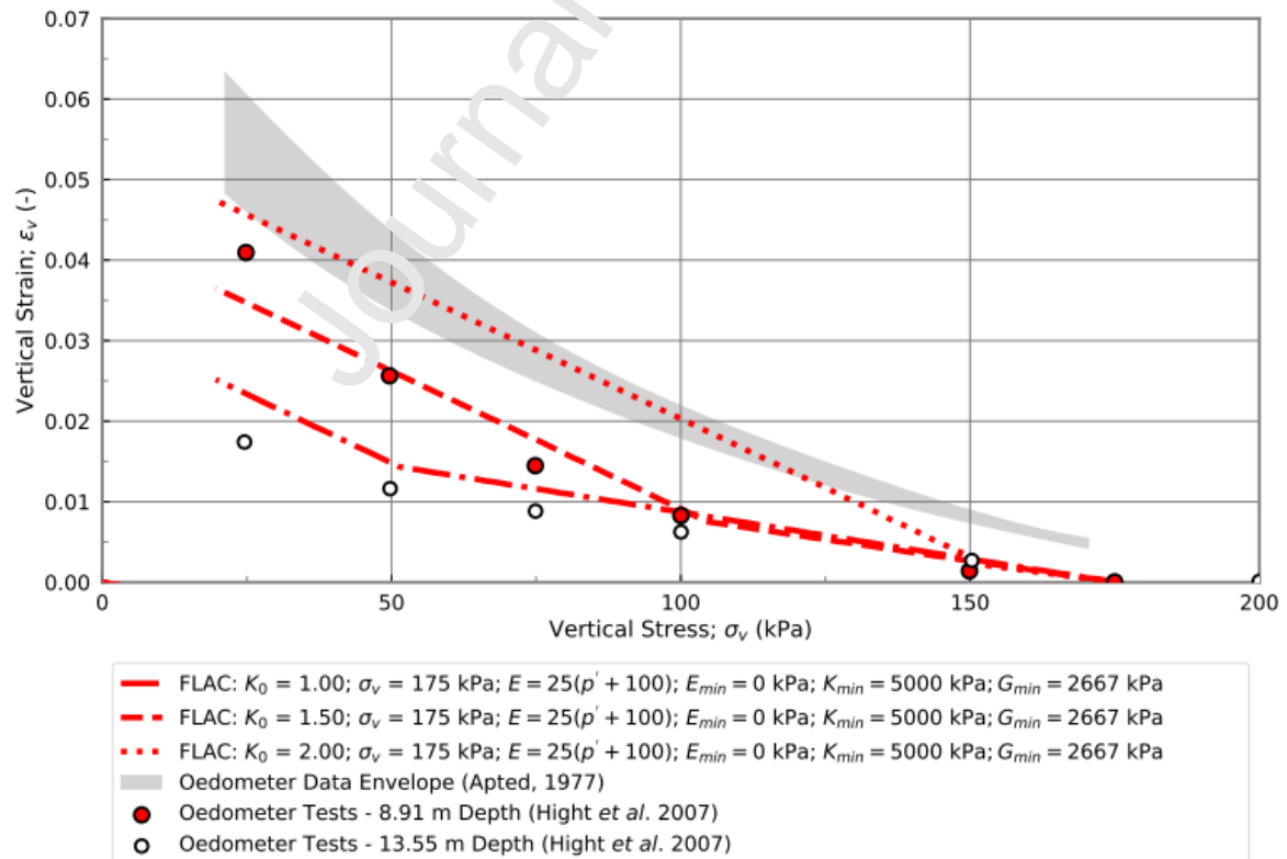
Figure 7: Effect of adopted K_0 value on modelled swelling response
