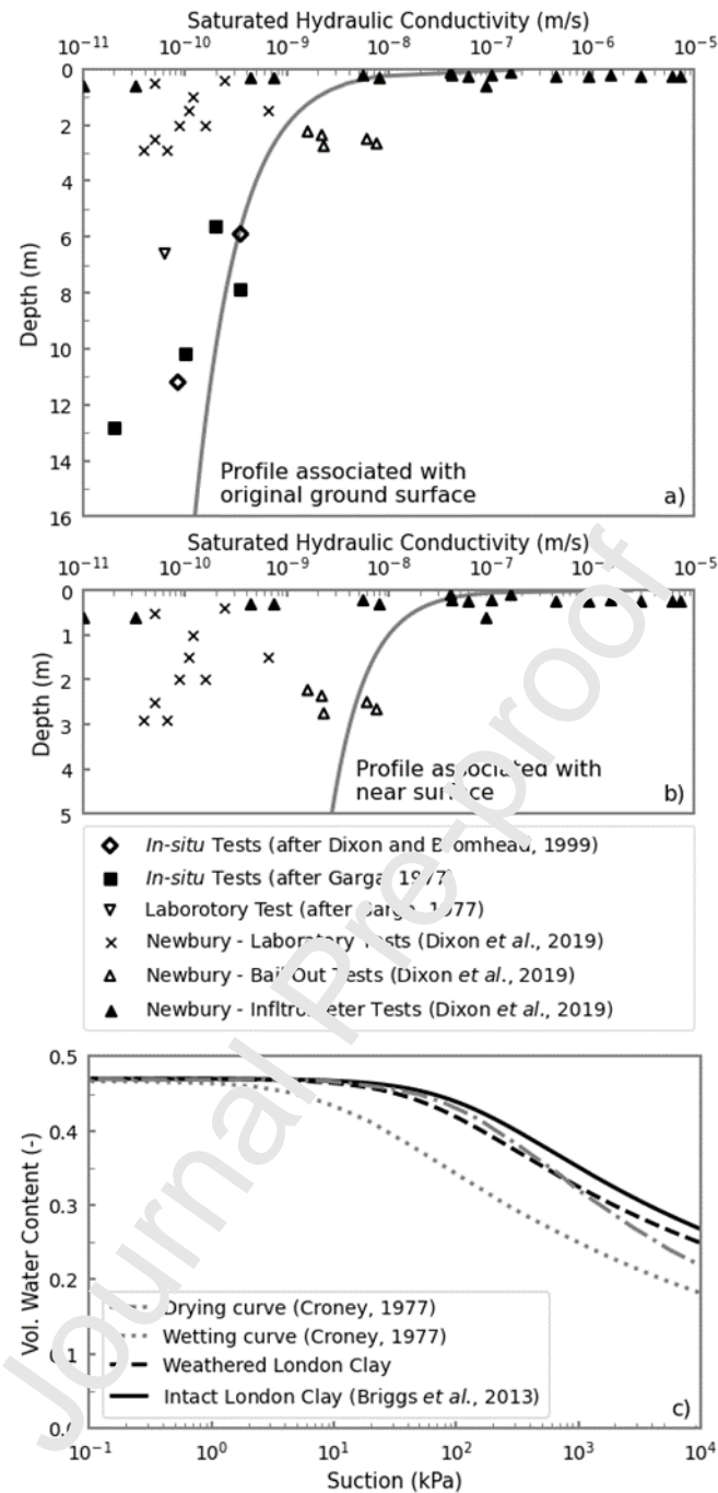
Figure 5: Hydrogeological material properties; a) depth dependent saturated hydraulic conductivity profile associated with original ground surface; b) depth dependent saturated hydraulic conductivity profile associated with near-surface; c) soil water retention properties (after Briggs et al., 2013)
