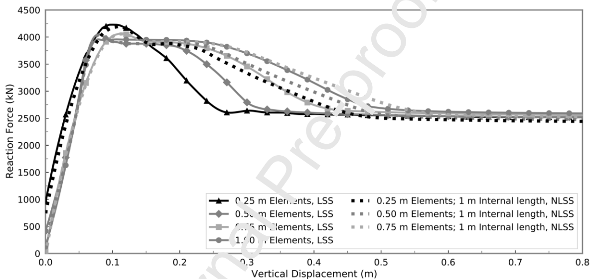
Figure 3: Results of numerically modelled biaxial tests on meshes with different densities and using local (LSS) and non-local strain softening (NLSS) to allow calibration of the softening model.
