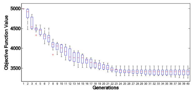
Fig. 5. GA performance in 10 runs with P_c = 0.7 , initialP_m = 0.01 and Pop = 100 for the case with 50 containers, five AGVs, three QCs and five YCs.
