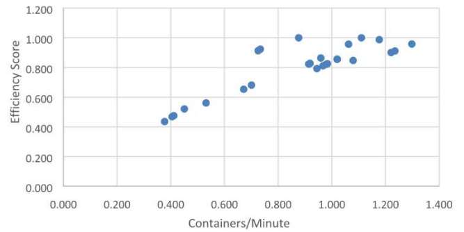
Fig. 6. Correlation between efficiency scores and the number of containers handled per minute.
