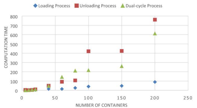
Fig. 7. A comparison of computation times (in seconds) for single-cycle and dual-cycle operations.
