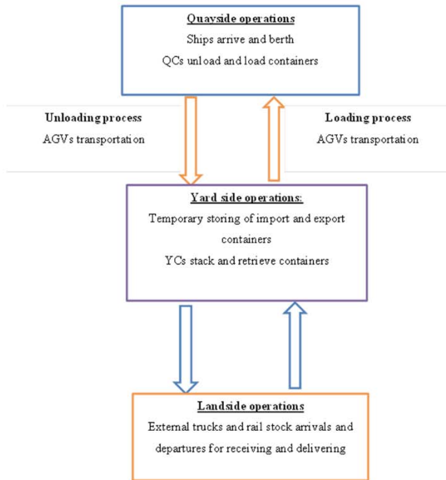
Fig. 1. Unloading and loading processes in a container terminal.
