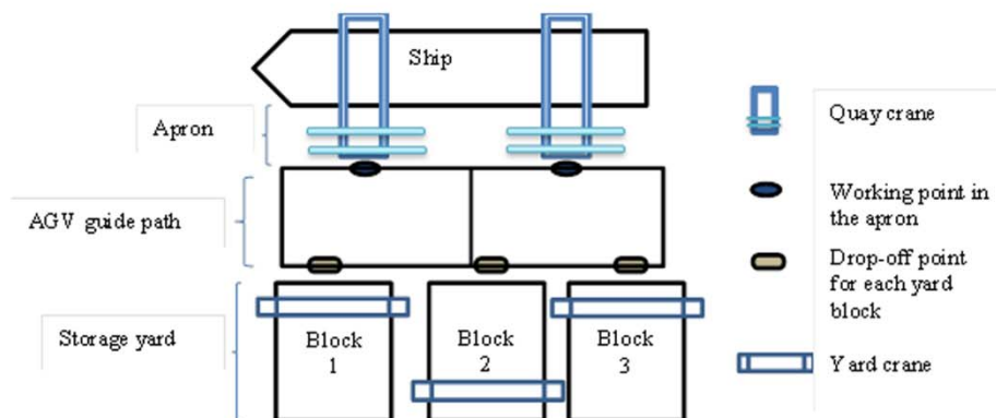
Fig. 2. The layout of an automated container terminal being analysed.
