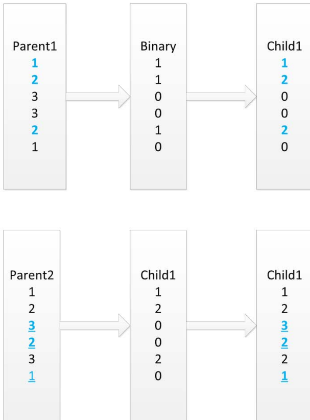
Fig. 4. An illustration of uniform crossover for an example of six containers, three AGVs and three YCs.
