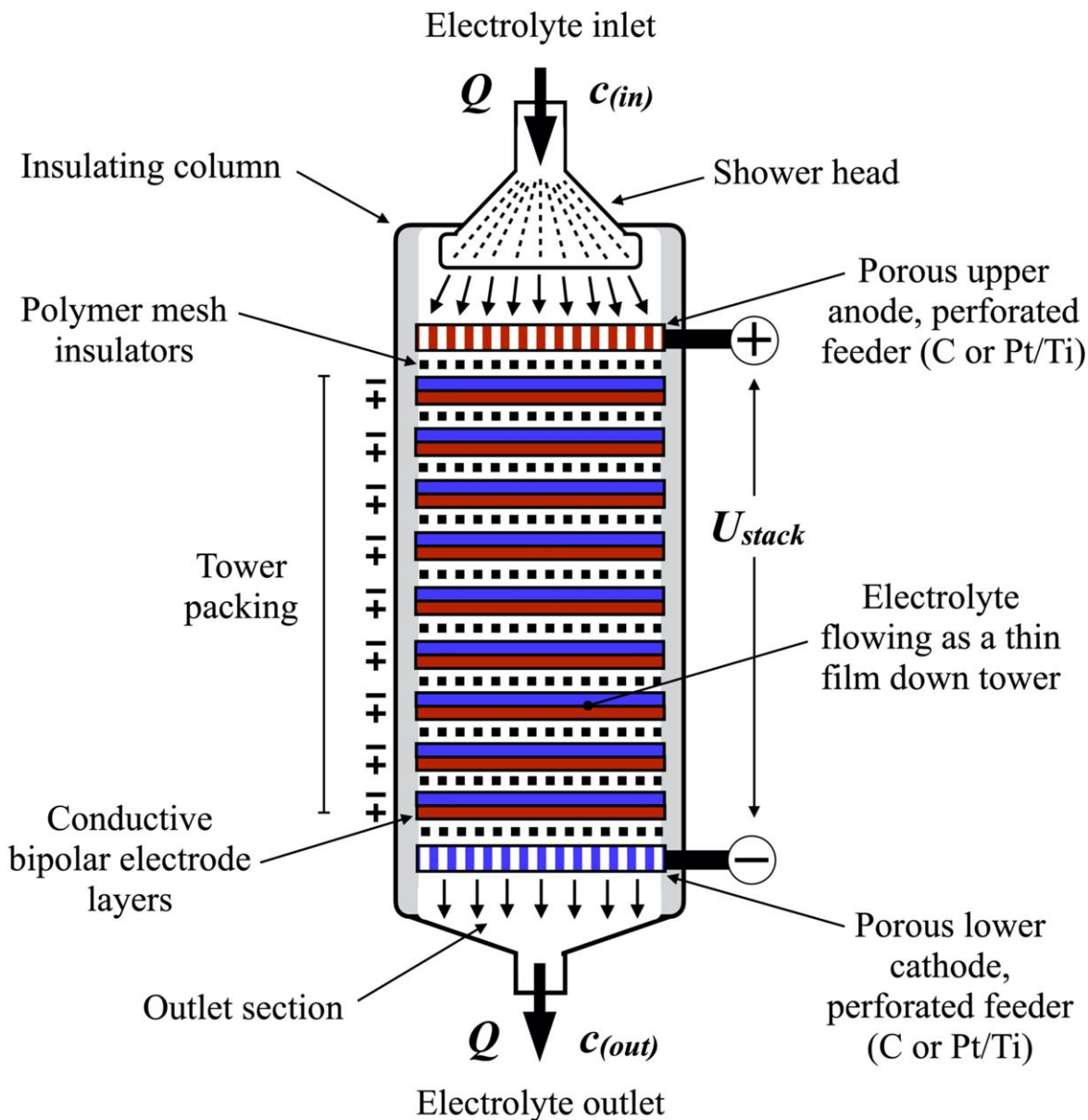
Figure 1. The bipolar trickle tower reactor concept, in which a thin film of electrolyte flows down a column past a series of identical bipolar electrode layers.
