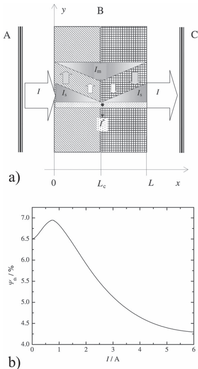
Figure 9. An example of the simulation of bipolar 3D electrodes in a flooded, vertical reactor which could be adapted for BTTRs. (a) Diagram of a stack with a single bipolar porous electrode. A, terminal anode; B, bipolar electrode; C, terminal cathode. The current at the metal ( I_m ) and solution phases ( I_s ) is represented schematically as a function of the distance along the bipolar layer ( L ). (b) Simulated leakage current fraction ( \Psi_{th} ) for increasing cell current ( I ). Adapted with permission from González Perez and Bisang, 2010, Theoretical and experimental study of electrochemical reactors with three-dimensional bipolar electrodes. J. Appl. Electrochem. , 40, p. 709–718. 39
