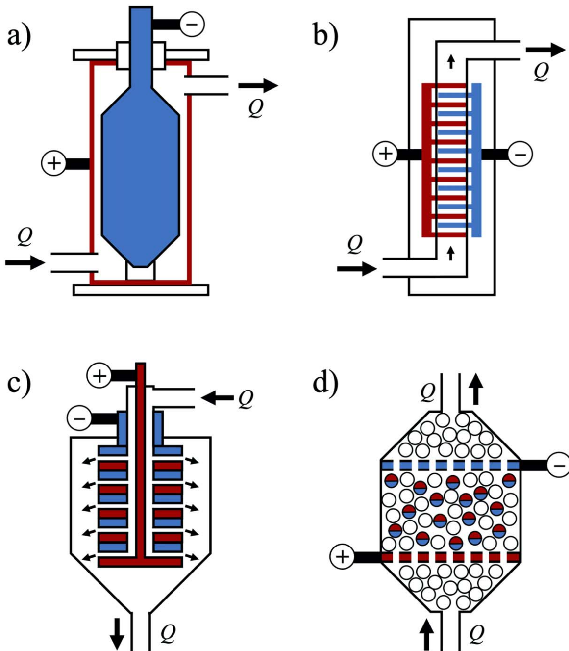
Figure 3. Concepts for thin film electrolyte and bipolar electrode reactors. (a) Monopolar concentric capillary gap (Eberson) cell, 42 (b) flow over monopolar interdigitated band electrodes, 46 (c) bipolar stacked disc, capillary radial outflow (Beck) cell 44 and (d) bipolar packed bed cell. 45
