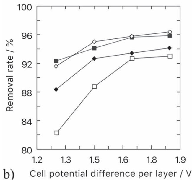
Figure 15. Removal rate of textile dyes vs applied potential at different volumetric flow rates for a BTTR with an internal diameter of 22 mm and 27 bipolar layers formed by four 6 mm × 6 mm graphite Raschig rings. (a) For Congo Red. (b) For Xiron Blau 2RHD. Open squares: 1.38 \times 10^{-4} m 3 h -1 ; solid squares: 2.28 \times 10^{-4} m 3 h -1 ; solid diamonds: 3.12 \times 10^{-4} m 3 h -1 ; open diamonds: 3.96 \times 10^{-4} m 3 h -1 . Data taken from Ögütveren and Koparal, 1992, Electrochemical treatment of water containing dye-stuffs: anodic oxidation of Congo Red and Xiron Blau 2RHD. Intern. J. Environmental Studies , 42, p. 41–52. 18
