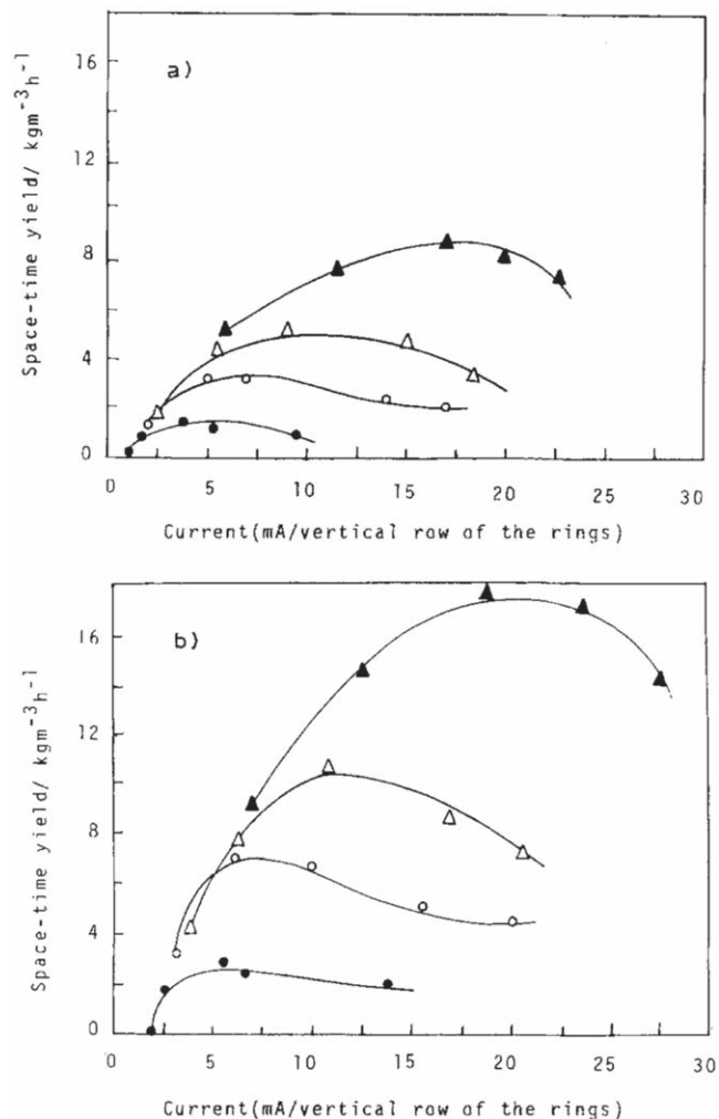
Figure 10. Application of the BTTR to electrosynthesis of cobalt compounds. Change in the space-time yield with current per layer of rings for initial Co(II) concentrations of: (a) 50 mol m -3 and (b) 100 mol m -3 of Co(II) ions at different mean linear flow velocity of electrolyte falling past the electrode surface. Closed circles: 6.7 × 10 -2 ; open circles: 2.0 × 10 -2 ; open triangles: 1.34 × 10 -2 ; closed triangles: 4.0 × 10 -2 cm s -1 . Adapted with permission from Ogutveren et al., 1992, The behaviour of a trickle tower electrolytic cell for the production of cobalt(III) acetate from cobalt(II) acetate. J. Appl. Electrochem. , 22, p. 351–357. 97
