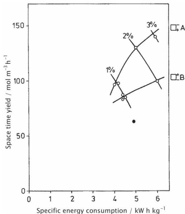
Figure 11. Application of the BTTR to electrosynthesis. The effects of polarity and sodium bromide concentration on performance of a BTTR used for synthesis of propylene oxide. A (upper curve) and B (lower curve) denote the polarity. The carpet plot shows space time yield vs specific energy consumption. After 60 recycles of electrolyte. Q = 500 \text{ cm}^3 \text{ min}^{-1} ; 3.5 V per layer; 1% NaBr. Open circles: aligned layer configuration; closed circle (one point): staggered arrangement. Adapted with permission from Ellis and Jansson, 1981, Further studies on the epoxidation of propylene in a bipolar trickle bed. J. App. Electrochem. , 11, p. 531–535. 29
