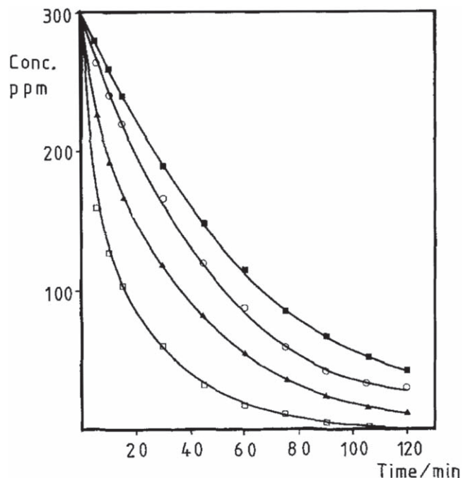
Figure 13. Application of the BTTR to cyanide oxidation. Concentration decay of cyanide ion during batch recycling of an approx. 2000 cm 3 volume at 0.5, 1.0, 1.5 and 2.0 dm 3 min -1 through the BTTR of 7.5 cm internal diameter, which consisted of 20, 34 or 48 layers of 12.5 mm long, 12.5 mm diameter Raschig rings, operated at 2 or 3 V per layer. Initial CN - concentration: 300 mg dm -3 (ppm) at pH 10.4. Closed squares: 49 layers, 3 V/layer, 2 dm 3 min -1 ; open circles: 49 layers, 3 V/layer, 0.5 dm 3 min -1 ; solid triangles: 21 layers, 2 V/layer, 1.0 dm 3 min -1 ; open circles: 21 layers, 2 V/layer, 0.5 dm 3 min -1 . Reproduced with permission from El-Ghaoui et al., 1982, Application of the trickle tower to problems of pollution control. II. The direct and indirect oxidation of cyanide. J. Appl. Electrochem. , 12, p. 69–73. 33
