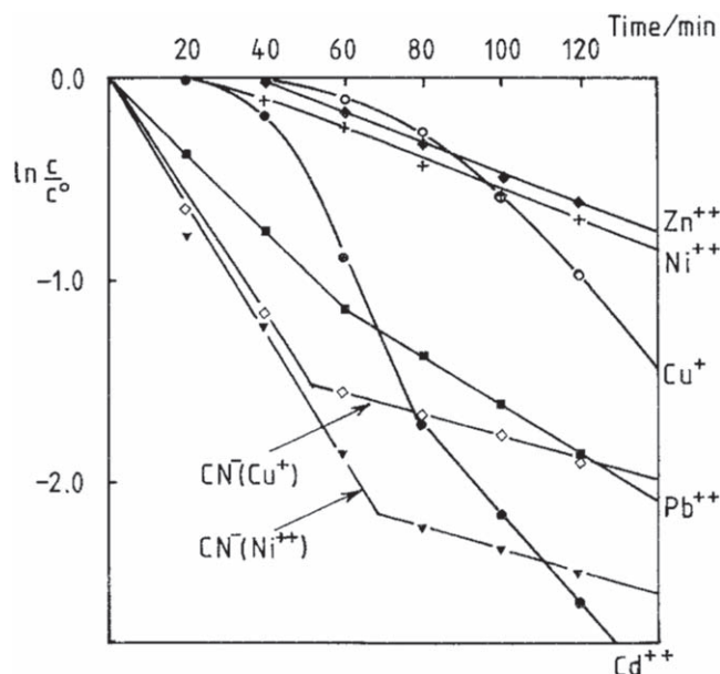
Figure 14. Application of the BTTR to environmental remediation of Zn, Ni, Cu, Pb and Cd and cyanide removal from metal cyanide complex solutions. Concentration decay during batch recycling of an approx. 1000 cm 3 volume at 0.6 dm 3 min -1 through the BTTR of 6.2 cm internal diameter, which consisted of 7 layers of 6.5 mm long, 6.5 mm diameter Raschig rings, operated at 2.25 V per layer. Initial metal and CN - concentrations were 100 and 300 mg dm -3 (ppm) at pH 10. Reproduced with permission from El-Ghaoui and Jansson, 1982, Application of the trickle tower to problems of pollution control. III. Heavy-metal cyanide solutions. J. Appl. Electrochem. , 12, p. 75–80. 35
