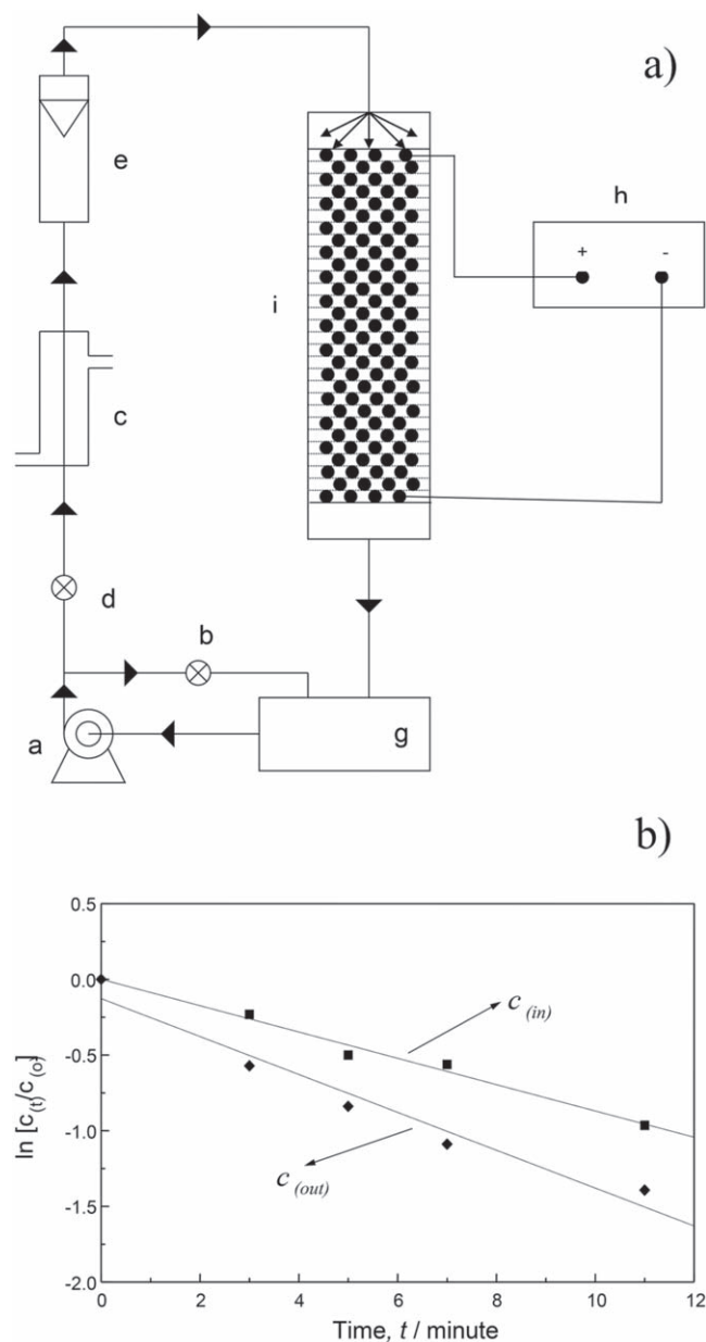
Figure 12. A Raschig ring laboratory BTTR for the study of operational parameters. (a) Experimental arrangement. a, magnetically-coupled pump; b, by-pass valve; c, water-cooled glass coil condenser; d, flow control valve; e, rotameter; f, carbon electrode packing material; g, electrolyte reservoir (3 dm 3 ); h, direct current power supply (200 V/10 A); i, tower. (b) Inlet and outlet concentrations from the BTTR for Cu(II) ion removal from acid sulphate solution at pH 2 as a function of time at 2.0 V per layer, Q = 33.3 \text{ cm}^3 \text{ s}^{-1} and c_{(0)} = 100 \text{ mg dm}^{-3} . Reproduced with permission from Trinidad et al., 2004, The effect of operational parameters on the performance of a bipolar trickle tower reactor. J. Chem. Technol. Biotechnol. 79 (9), p. 954–960. 37
