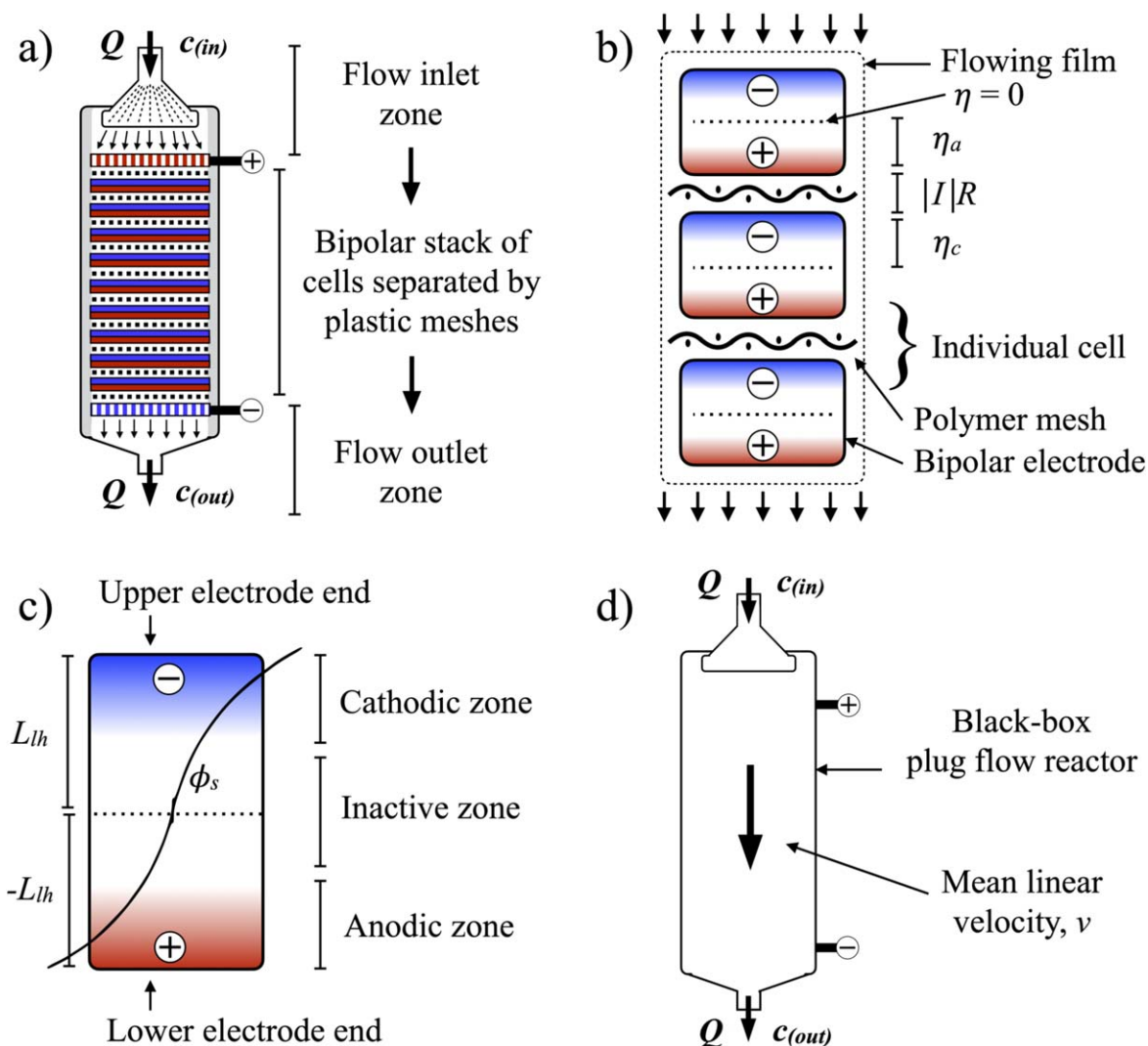
Figure 6. The zoned behaviour of the BTTR. (a) the progress of electrolyte down the reactor involves an entry (inlet and flow conditioning) zone, the bipolar stack of electrodes separated by plastic meshes in the tower packing, then a drainage, outlet zone, (b) an individual cell is formed between electrode layers across a thin electrolyte film in the region of the polymer mesh separator, (c) an individual bipolar layer can be divided into 3 regions. At very negative overpotential at the top edge, a cathodic region exists; at the opposite, lower end of there is an anodic region; a central zone of the layer having little or no electrochemical activity, (d) in a simple, black-box approach, the BTTR can be viewed as a single pass PFR experiencing a steady volumetric flow rate, Q resulting in a mean linear velocity, v of electrolyte, with the inlet reactant concentration at the top, c_{(in)} progressively falling to the outlet concentration, c_{(out)} at the bottom.
