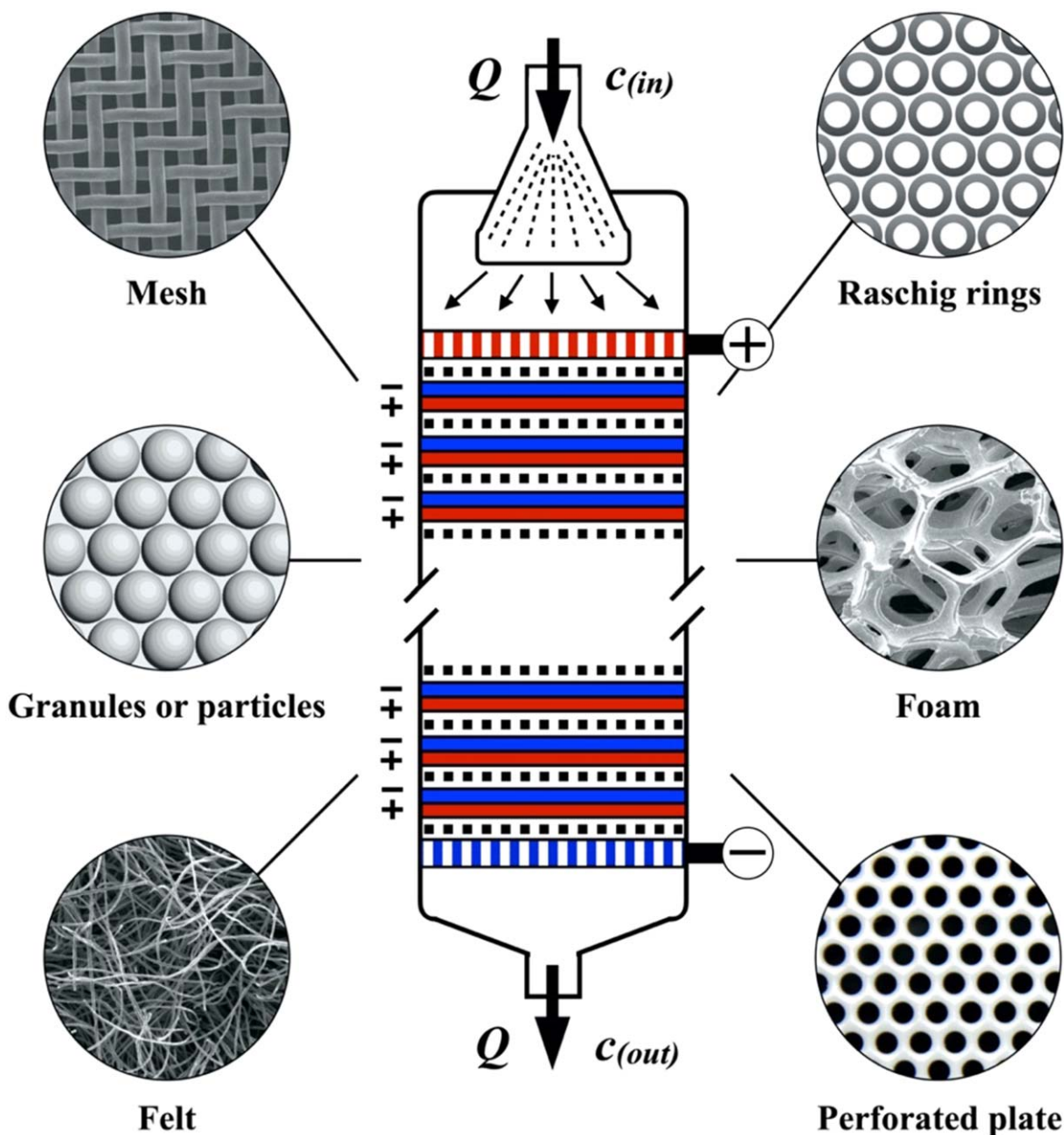
Figure 5. Types of electrodes used in the BTTR. (a) carbon or metal Raschig rings, (b) titanium mesh, (c) graphite granules, (d) carbon or metal foam, (e) titanium felt, and (f) perforated carbon plate. Metal substrates can be coated with a catalyst such as platinum or BDD.
