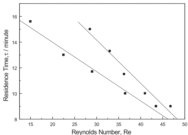
Figure 7. Mean residence time measurements in a Raschig ring BTTR as a function of film Re number. Solid circles: actual values calculated from analysis of the first moment of KCl concentration vs time curves. Solid squares: nominal values calculated from the relationship: \tau_R = V_R/Q . Reproduced with permission from Trinidad et al., 2004, The effect of operational parameters on the performance of a bipolar trickle tower reactor. J. Chem. Technol. Biotechnol. 79(9), p. 954–960. 37
