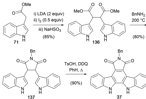
Scheme 20 Bergman and co-workers' synthesis of the arcyriaflavin A derivative 37 .
