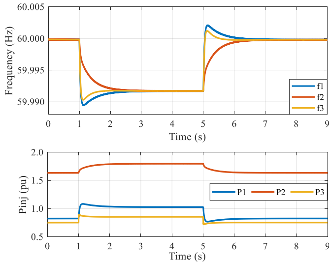
Fig. 17. Frequency and power injection in All GFC case subject to a load change.
