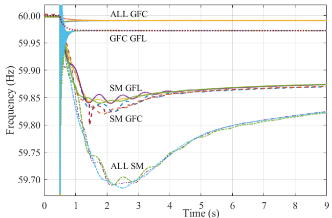
Fig. 22. Frequency variation in all five cases due to a load increment at bus 6.
