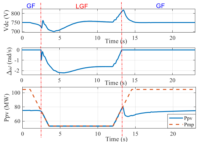
Fig. 16. Performance of the proposed control strategy in the SM GFC case subject to irradiance change.
