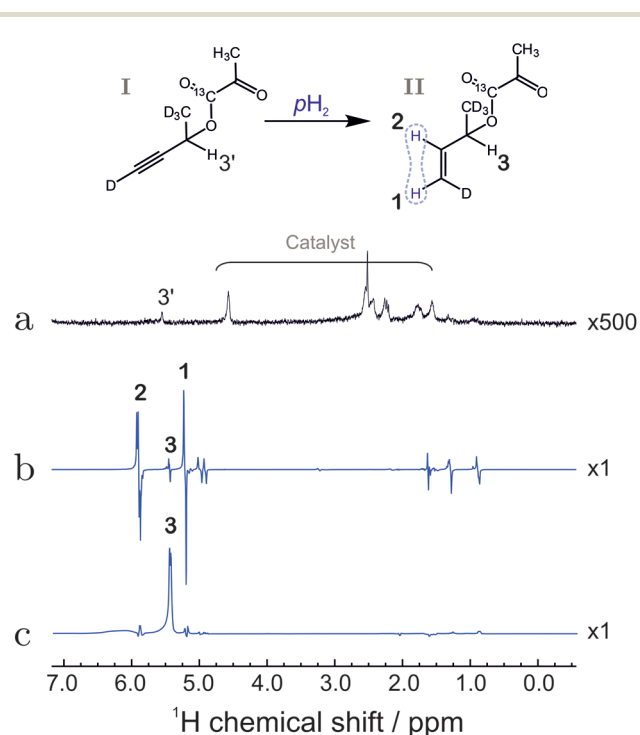
Fig. 4 (a) Spectrum of compound I before hydrogenation, recorded by applying a \pi/2 pulse to a sample in thermal equilibrium (expanded vertically by a factor of 500). (b) Hyperpolarized ^1\text{H} spectrum of compound II , recorded by applying a \pi/4 pulse to the sample after reaction with para -enriched hydrogen; (c) ^1\text{H} spectrum after reaction of substance I with para -enriched hydrogen, and application of the pulse sequence in Fig. 3 up to time point 6. The spectrum displays the strongly enhanced signal of the relay proton (labelled 3). The bold numbers indicate the spectral lines associated with the protons of interest. For the chemical shifts, see the caption to Fig. 2. The other anti-phase features in the spectrum (b) originate from the fully hydrogenated form of the precursor (signals at 1.3 ppm and 0.9 ppm) as well as a hydrogenated 1,5-cyclooctadiene (signal at 1.6 ppm). The origin of the line at 5 ppm is not fully understood but may be associated with trans -hydrogenation product or impurities.
