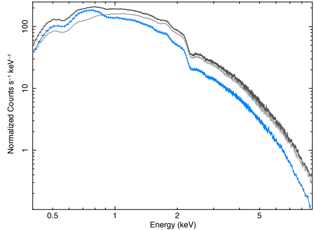
Figure 3. Comparison of the 0.4 – 9 keV counts spectra for the NICER observations reported here (blue) and the observations from 2017 intervals A (light grey) and E (dark grey) from Ludlam et al. (2019b). The source is at a lower flux in 2020 in comparison to the previous NICER observations.
