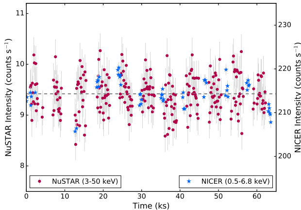
Figure 1. Light-curve for the NuSTAR/FPMA (circles) and NICER (stars) observations of 4U 1543–624 binned to 128 s. The grey dashed line indicates the average count rate for both NuSTAR and NICER. The time elapsed is from the start of the NICER observation on 2020-04-19 at 07:12:55UT. The source exhibits \lesssim 10\% variability over the course of the observation. Only one FPM is shown for clarity.
