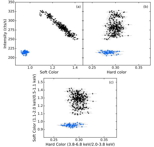
Figure 2. A comparison of the NICER observations of 4U 1543–624 during the 2017 outburst (black circles) reported in Ludlam et al. (2019b) to the observations obtained in 2020 (blue stars) for: a) the soft color versus the source intensity in the 0.5–6.8 keV band, b) the hard color versus intensity, and c) the soft color versus the hard color. The new observations probe different regions on these planes.
