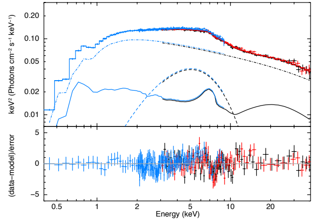
Figure 5. The unfolded spectrum with model components for the NICER (blue) and NuSTAR (FPMA: black, FPMB: red) data for the reflection modeling reported in Table 1. The dashed line indicates the single-temperature blackbody, the dot-dashed line is the power-law component, the solid line is the reflection component from XILLVERCO.
