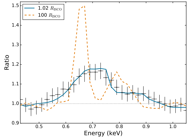
Figure 6. Best-fit reflection model reported in Table 1 at 1.02 R_{\text{ISCO}} (solid line) and contrasting 100 R_{\text{ISCO}} (dashed line) overlaid on the NICER data to highlight the broad O line component. The larger inner disk radius relaxes the relativistic effects to show the local rest-frame emission. The O VIII Lyman \alpha and \beta components can be seen when relativistic effects are removed. For clarity, the data were rebinned.
