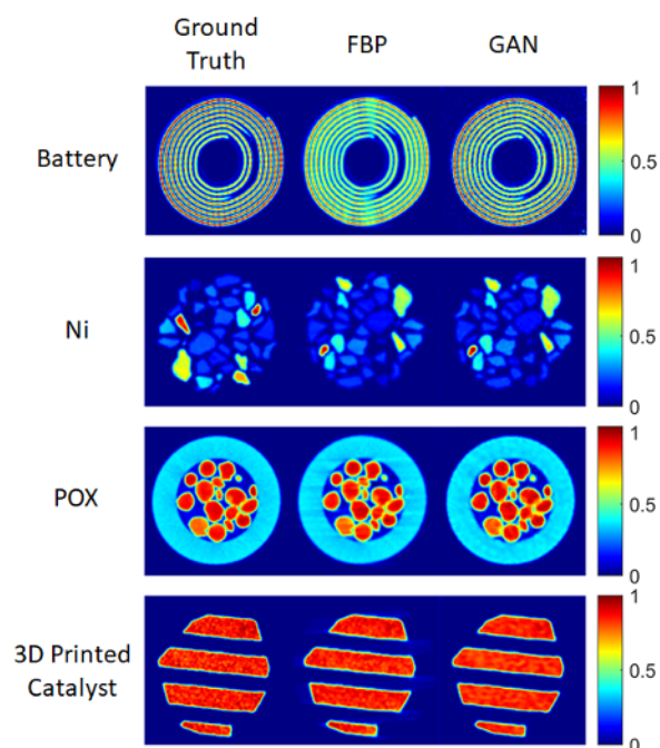
Figure 7: Comparison between reconstructed images using the filtered back-projection algorithm (middle) and the GAN (right).
