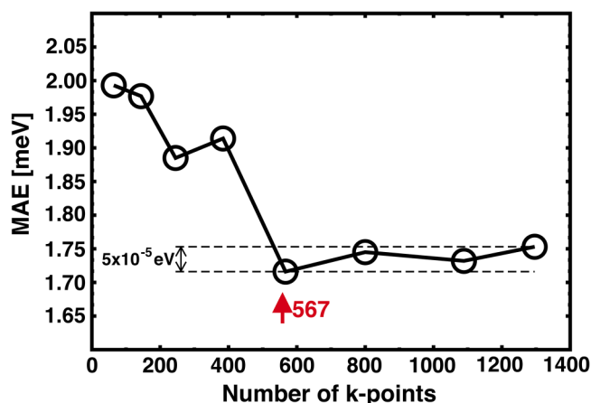
FIG. 7. Magnetocrystalline anisotropy of the optimized Y_2Fe_{14}B bulk alloy as a function of the number of the k -points. The interval between the two dashed lines shows the magnetic anisotropy dispersion for the higher k -point values. The red arrow represents the number of k -points chosen in order to have accurate MAE values.
