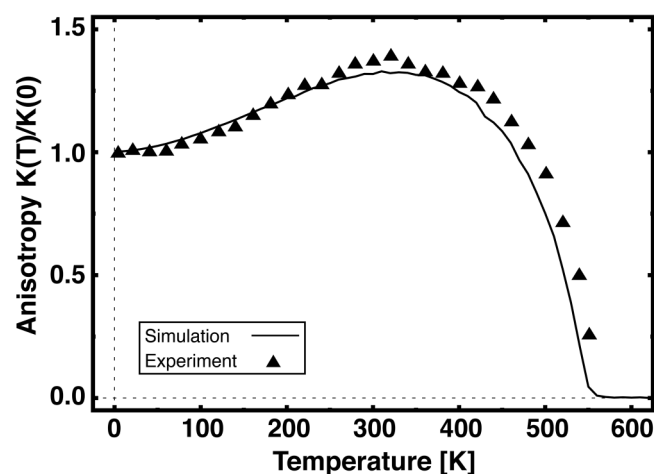
FIG. 10. Atomistic simulation of the temperature dependent effective anisotropy of \text{Y}_2\text{Fe}_{14}\text{B} with a mixture of 2-ion and single ion anisotropies (line) in comparison with the experimental data of Grossinger et al. 34 (points). The simulation and experimental data show very good agreement, suggesting that mixed anisotropies are an important component of anisotropy in \text{R}_2\text{Fe}_{14}\text{B} alloys.
