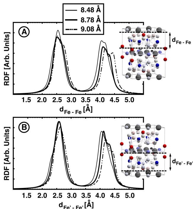
FIG. 3. Lorentzian broadening of the bond distances between Fe species for different groups of atoms, d_{Fe-Fe} and d_{Fe'-Fe'} , A and B graphs, respectively. To the right on each graph is shown the schematic representation of Y_2Fe_{14}B UC which clarifies, between black dashed lines, each one of the Fe groups atoms under consideration.
