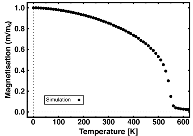
FIG. 9. Simulated temperature dependent magnetization for \text{Y}_2\text{Fe}_{14}\text{B} .
