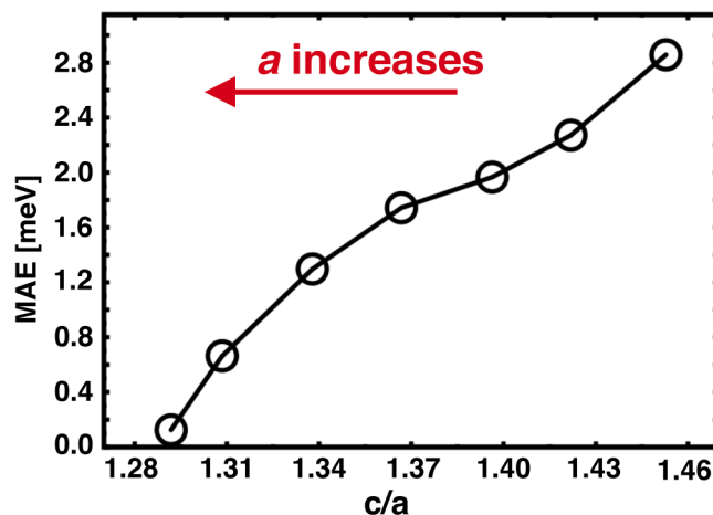
FIG. 8. Magnetic anisotropy energy as a function of the out-of-plane c/a parameter.
