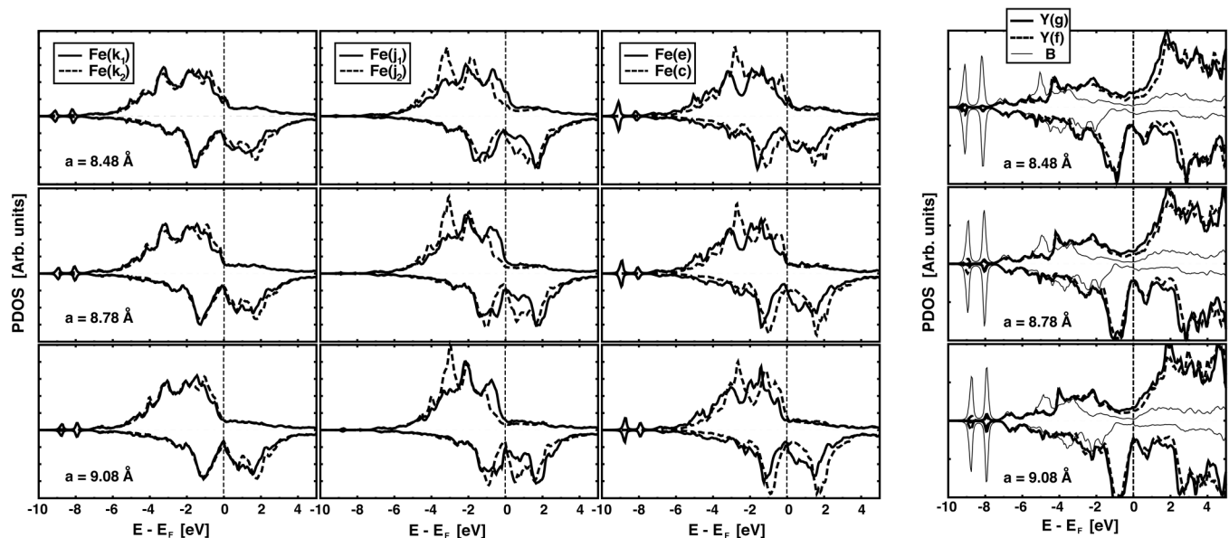
FIG. 4. (Left) Spin-resolved density of states for k_{1/2} , j_{1/2} and c, e different Fe sites, first second and third column, respectively. In a row is depicted the PDOS for a = 8.48, 8.78, and 9.08 Å lattice values; (right) spin-resolved density of states for the Y( g ), Y( f ), and B atomic species, thick solid, dashed, and thin solid black lines, respectively. From top to bottom, the smaller ( a = 8.48 Å), intermediate ( a = 8.78 Å), bigger ( a = 9.08 Å) size lattices are presented.
