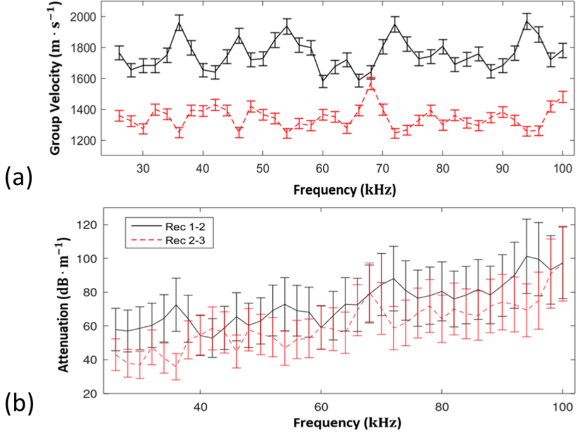
Figure 3: (Color online) Equivalent plane wave group velocity and attenuation (i.e. the effects of geometrical spreading having been corrected out from these data) in gassy sediment in the frequency range 26 - 100 kHz as measured by the hydrophones 1 and 2 (unbroken black line) and hydrophones 2 and 3 (red dashed lines) at Calshot. The error bars indicate the standard deviation.
