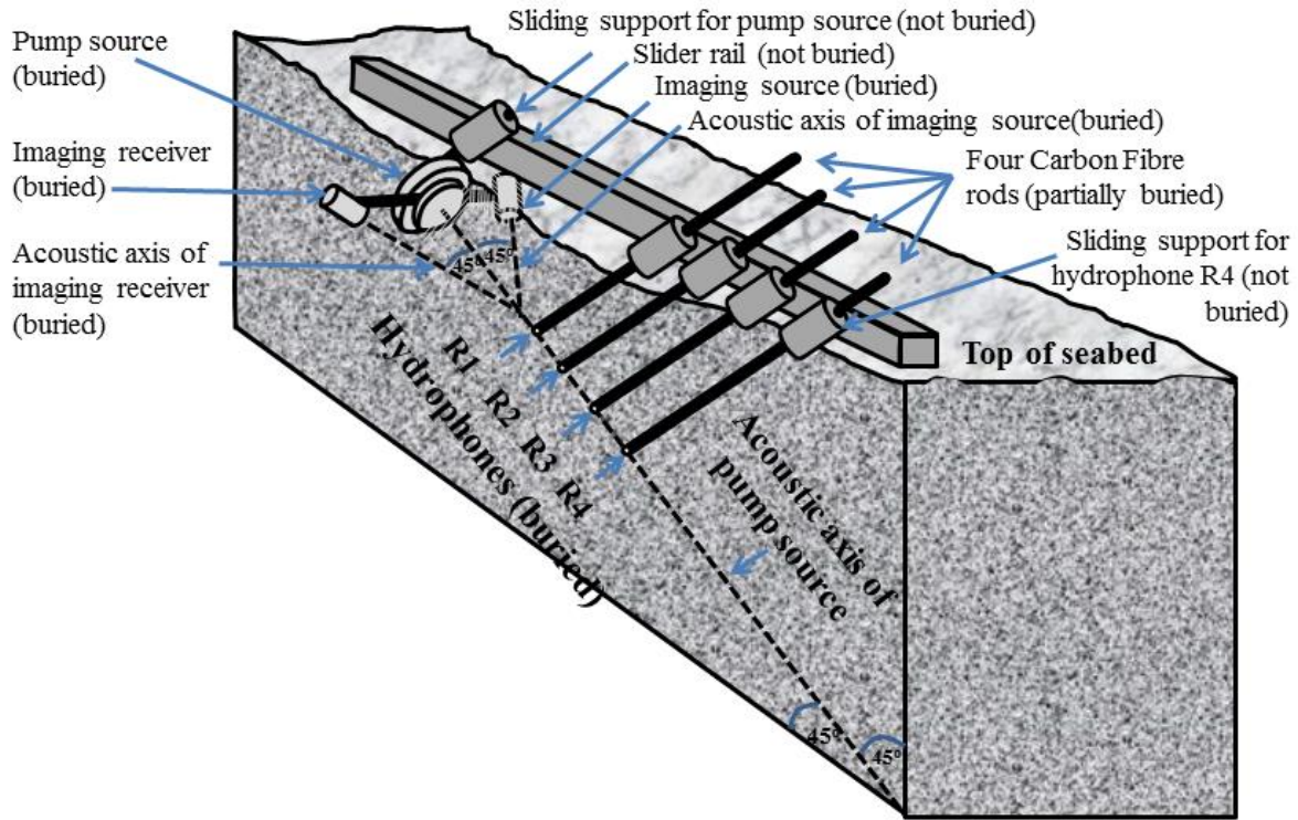
Figure 1: The gassy sediment experiment rig. R1, R2, R3 and R4 denote the locations of four hydrophone receivers which record the signals sent out from the pump source. The combination frequency apparatus consists of the high (imaging) frequency transmitter, the pump source and the high-frequency receiver. The imaging source and receiver have equal angular distances ( 45^\circ ) from the pump axis.
