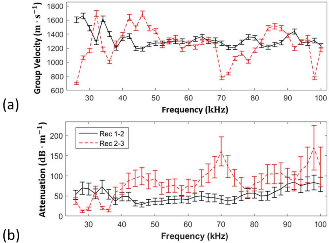
Figure 4: (Color online) Equivalent plane wave group velocity and attenuation in gassy sediment in the frequency range 26 - 100 kHz as measured by the hydrophones 1 and 2 (unbroken black line) and hydrophones 2 and 3 (red dashed lines) of the propagation rig at the Mercury site. The error bars indicate the standard deviation.
