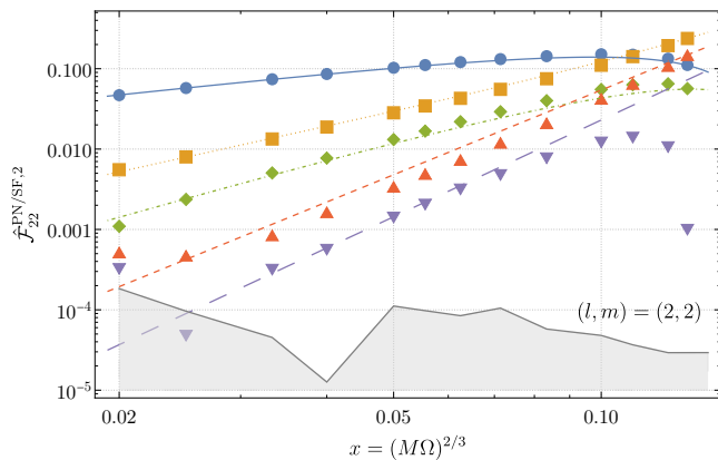
FIG. 7. The (Newtonian-normalized) second-order flux, \hat{\mathcal{F}}_{22}^{\text{PN/SF},2} , vs the \mathcal{O}(\nu^3) contributions to the PN series, \hat{\mathcal{F}}_{22}^{\text{PN},2} , for the (l, m) = (2, 2) mode. The solid (blue) curve shows the \mathcal{O}(\nu^3) contribution to the 3.5PN flux and the circles show our 2SF result. We then subtract the leading \mathcal{O}(\nu^3) PN term, 55x/21 , from both and get the (orange) dotted curve and the squares. After subtracting all the PN terms through x^2 , we get the (green) dot-dashed and diamonds. Subtracting all the PN terms through x^3 , we get the (red) dashed curve and the triangles. Finally, after subtracting all the PN terms through x^{7/2} , i.e., all the known PN terms, the subdominant residual is shown with (purple) upside down triangles. The residual appears to approach the x^4 reference curve shown by the long dashed (purple) line. The gray shaded region shows the estimated error in our 2SF flux. We see similar agreement for other modes.
