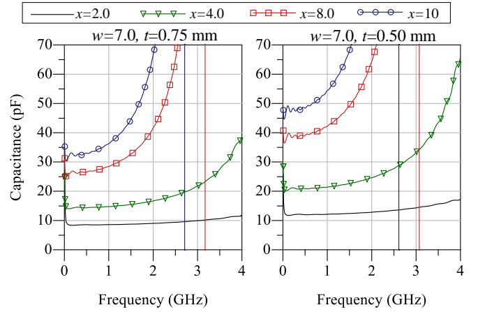
FIGURE 3. Simulated capacitance of the standalone capacitors, with no microstrip feed, for two dielectric heights t .
