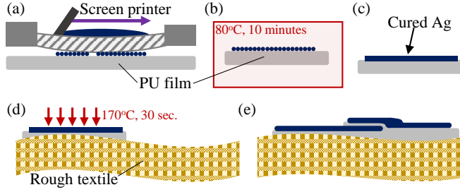
FIGURE 4. Fabrication steps of the proposed multi-layered screen-printed microstrip: (a) screen printing of the silver traces on the PU film; (b) silver traces curing; (c) the cured silver-on-PU trace ready for lamination onto other substrates; (d) heat-pressing on a rough textile substrate; (e) the assembled multi-layered structure using steps (a)-(d).
