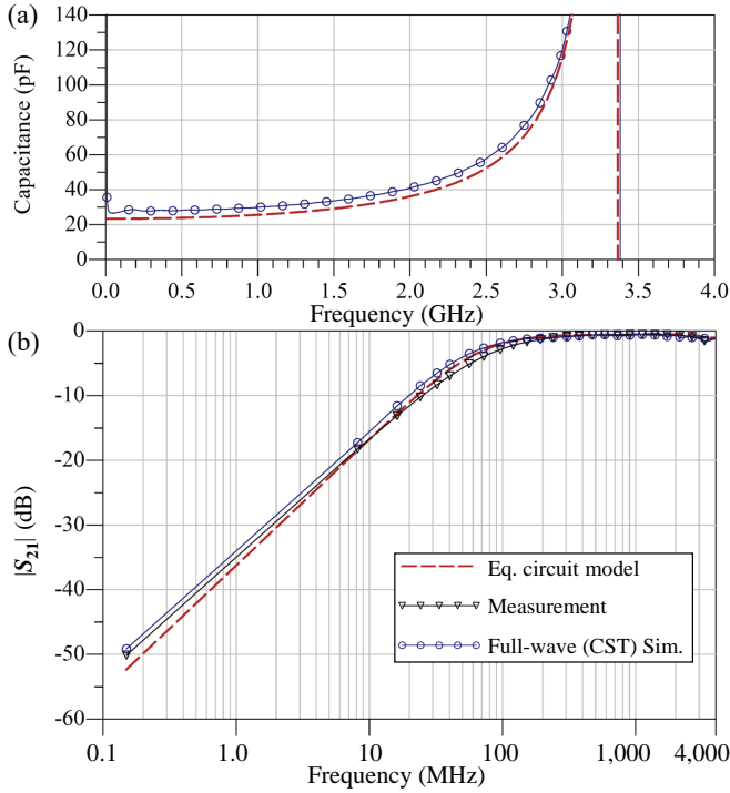
FIGURE 6. Performance of the 10 mm-long capacitor-impregnated microstrip: (a) analytical and full-wave numerical capacitance of the standalone capacitor; (b) analytical, numerical, and experimental S_{21} of the 10 cm-long microstrip line on felt with a 10 mm capacitor.
