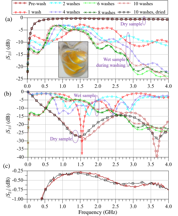
FIGURE 9. Measured s-parameters of the printed microstrip line with x=5 mm (20 pF) capacitor for 10 washing cycles: (a) S_{21} before, during (wet), and after (dried) washing; (b) S_{11} before, during (wet), and after (dried) washing; (c) the pass-band of the lines showing minimal attenuation variation.
