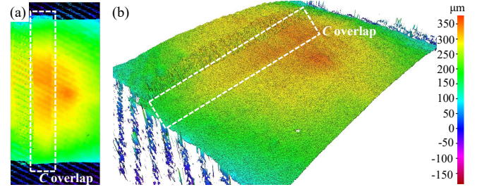
FIGURE 12. Measured surface profile of the DC blocking line on a woven polyester-cotton substrate: (a) 2D plot of the height at the signal-line capacitor; (b) 3D plot of the ground plane capacitor.
