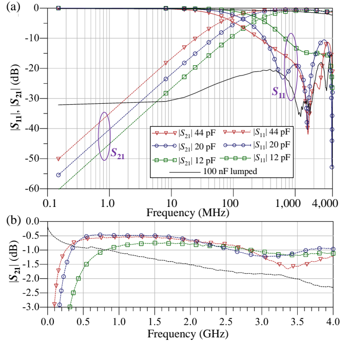
FIGURE 7. Measured s-parameters of the capacitor-impregnated microstrip lines showing over 60 dB S_{21} isolation at 150 kHz: (a) broadband |S_{21,11}| logarithmic plot; (b) the pass-band of the lines; the 12-44 pF capacitances refer to the low-frequency parallel-plate printed capacitors.
