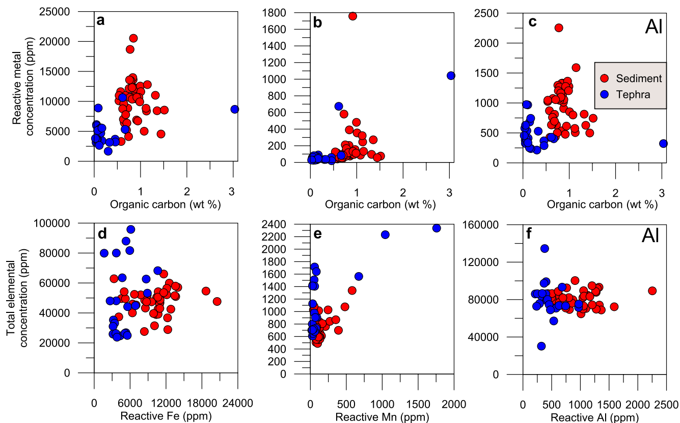
Figure 3. Comparison of total metal contents, reactive metal contents and organic carbon (OC) content of sediments and tephtras from Site U1339D. Panels a–c display reactive metal concentrations plotted against OC whilst panels d–f show total elemental content for Fe, Mn and Al against respective reactive metal content. Tephra samples are colored blue, with sediments in red.
