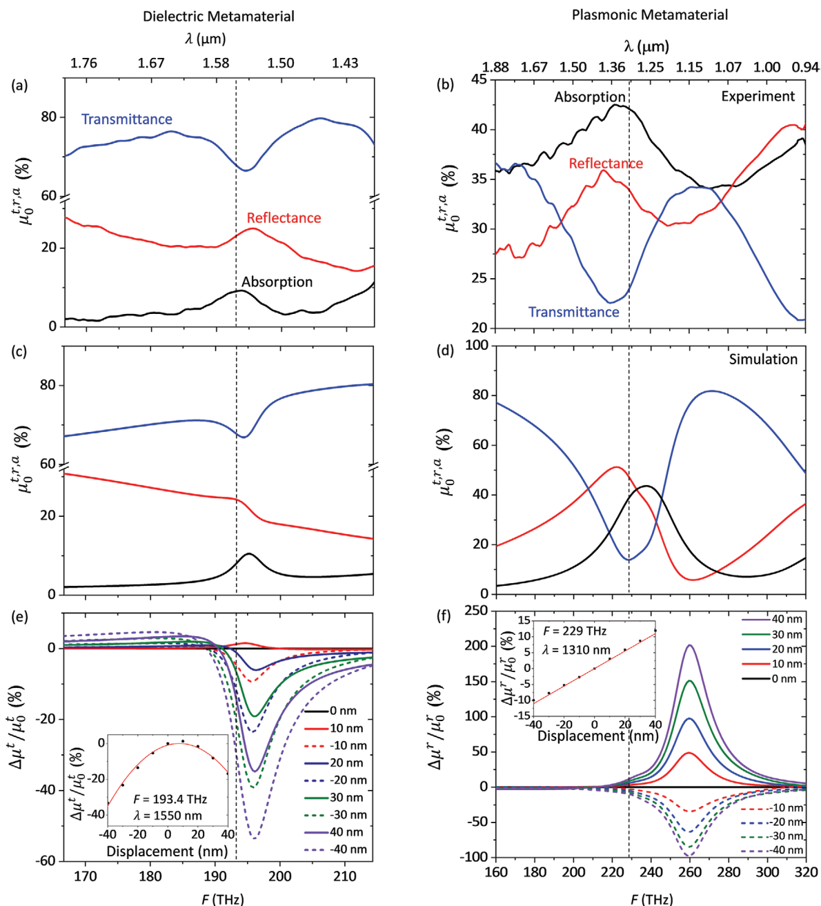
Figure 3. Optical properties of the dielectric and plasmonic nanomechanical metamaterials. a,b) Experimentally measured and c,d) computed optical reflection ( \mu_0^r ), transmission ( \mu_0^t ) and absorption ( \mu_0^a ) spectra of the dielectric and plasmonic metamaterials. e,f) Computed values of (\Delta\mu^t/\mu_0^t) , a figure of merit of responsivity of the metamaterial's optical properties to the relative displacement of neighboring beams along z at different levels of displacement. The insets show the dependence of (\Delta\mu^t/\mu_0^t) on displacement at wavelengths of 1550 and 1310 nm, respectively. Positive displacement corresponds to the movement of narrower beams along +z relative to wider beams; all results are for x -polarized light.
