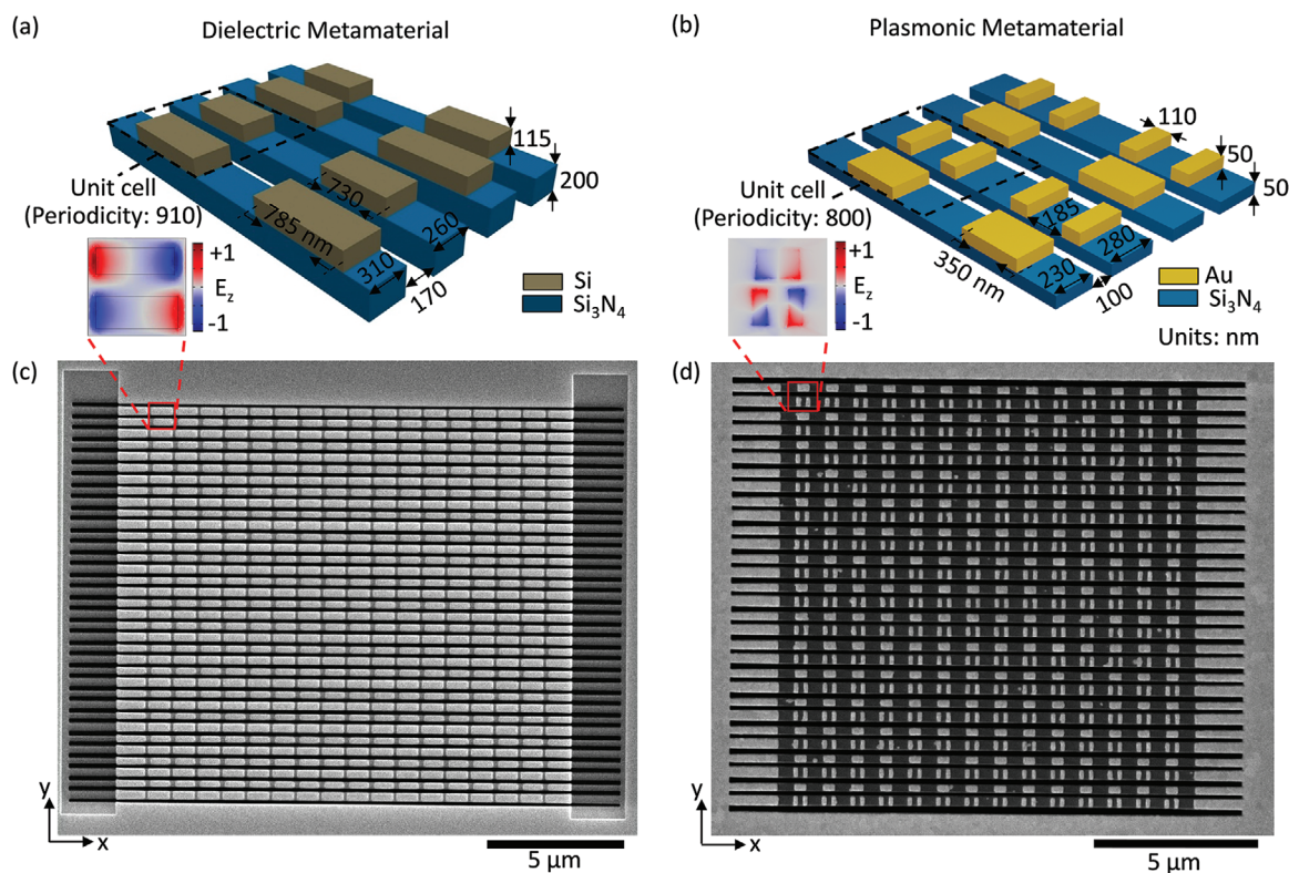
Figure 2. Nanomechanical photonic metamaterials. Structural schematic and SEM images of planar a,c) dielectric and b,d) plasmonic metamaterials fabricated on silicon nitride membranes. Insets show the resonant field distributions excited by x-polarized incident light at wavelengths of a) 1550 and b) 1310 nm.
