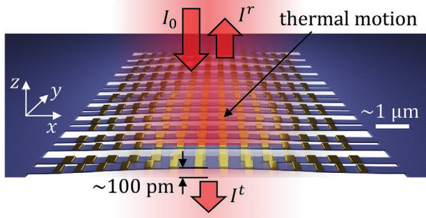
Figure 1. Thermal fluctuation of nanomechanical metamaterial optical properties. The photonic metamaterial is an array of beams of nanoscale width and thickness in the xy plane. The beams, typically a few tens of microns long, support a periodic array of optical resonators of nanoscale (subwavelength) dimensions. The optical properties of such arrays can be controlled via nanostructural reconfiguration driven by external stimuli such as electromagnetic forces, optical and acoustic waves. [2–4,7,8] Pico-metric thermal displacements of the individual beams also modulate the optical properties of the metamaterial, causing small fluctuations of its transmittance and reflectance.
