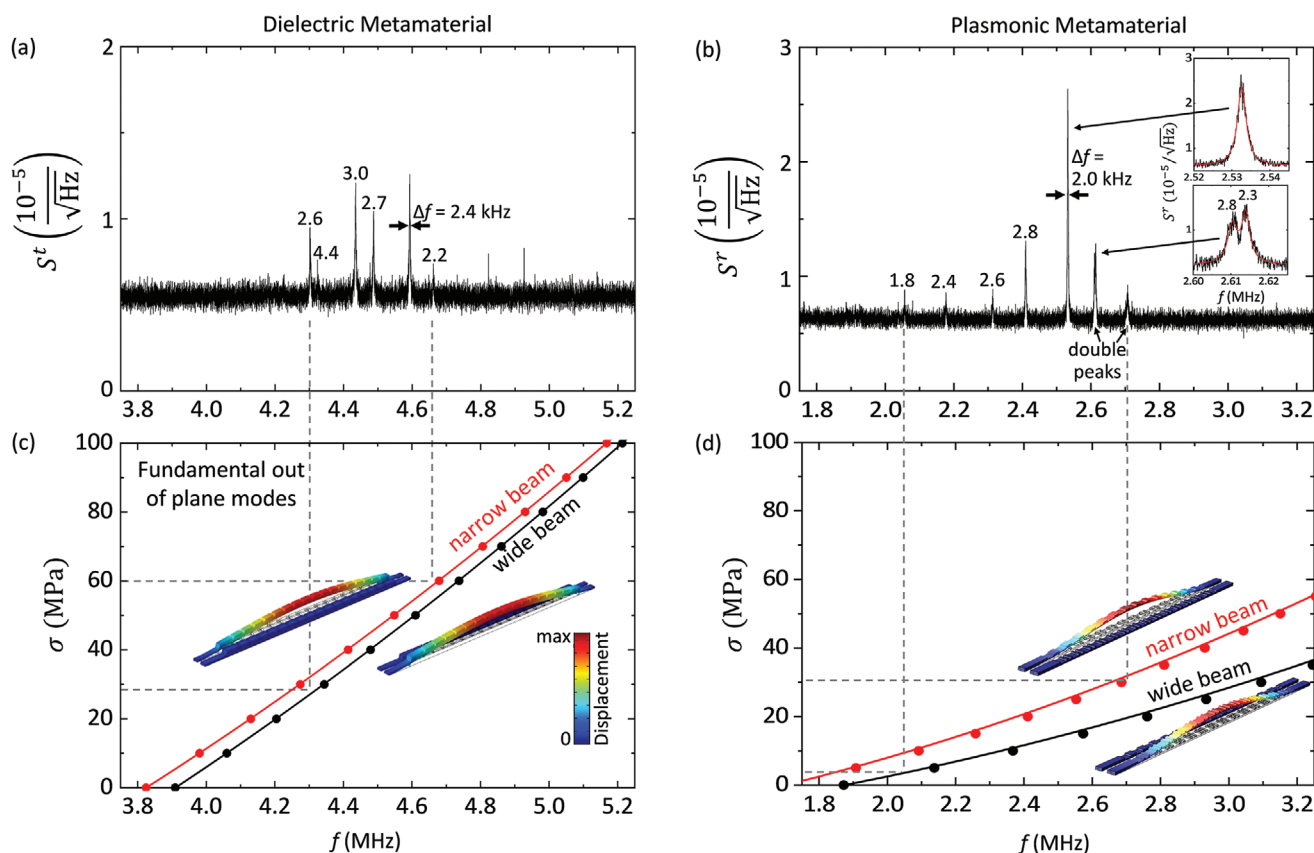
Figure 4. Thermal fluctuation of nanomechanical metamaterial optical properties. Measured spectral density of a) transmittance modulation S^t and b) reflectance modulation S^r by dielectric and plasmonic metamaterials, respectively. Resonant peak widths \Delta f are labeled in kHz and insets show enlarged examples of single (double) resonant peaks with single (double) Lorentzian fits. Frequencies of the fundamental out-of-plane resonances (insets) of the c) dielectric and d) plasmonic metamaterial beams for different levels of tensile stress \sigma . Simulated resonance frequencies of the nanostructured beams (data points) are shown with a fit according to Equation (8) (lines).
