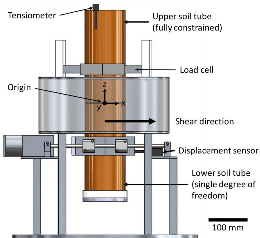
Figure 1: Schematic diagram of direct shear test rig. A photograph of the rig within the XCT scanner is given in [21].
