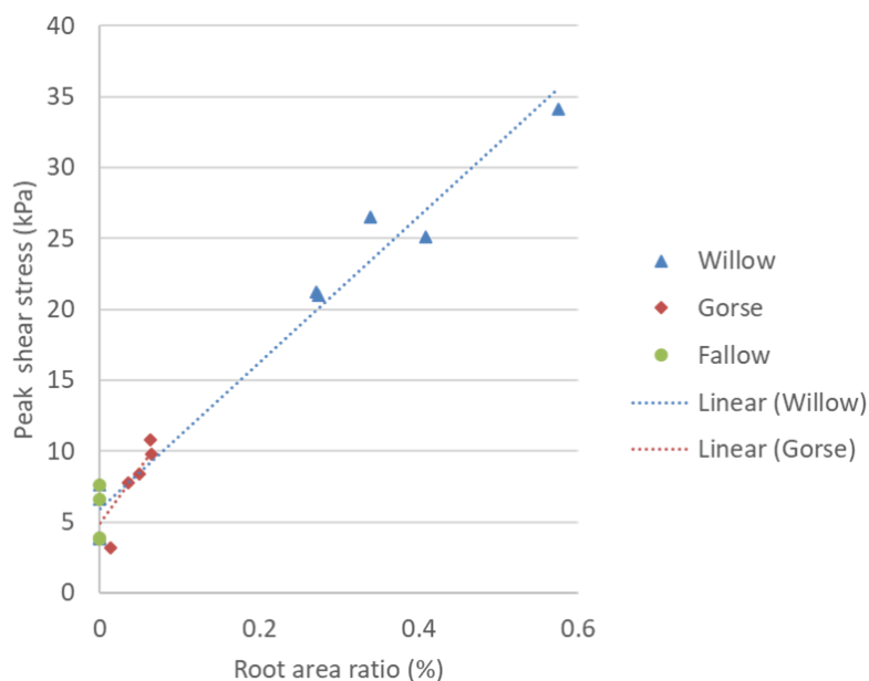
Figure 5: Effect of root area ratio (RAR) on peak shear stress reached during direct shear tests. RAR was calculated by summing the cross-sectional areas of each root passing through the shear plane.
