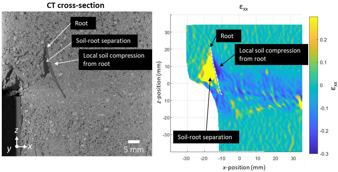
Figure 12: Local soil root behaviour in the region where root bending is observed. Local features are illustrated on the XCT cross-section (left) and DVC x-direction axial strain ( \epsilon_{xx} ) strain map (right).
