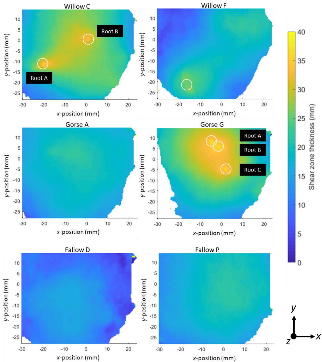
Figure 7: Shear zone thickness maps at the final load step for each specimen. Roots >1 mm in diameter are circled.
