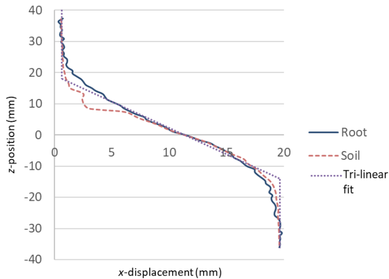
Figure 13: Plot showing x-displacement paths through the depth of the soil column (z-position). Different paths are observed between direct measurement of the root, DVC measurement of the soil near the root, and the tri-linear fit.
