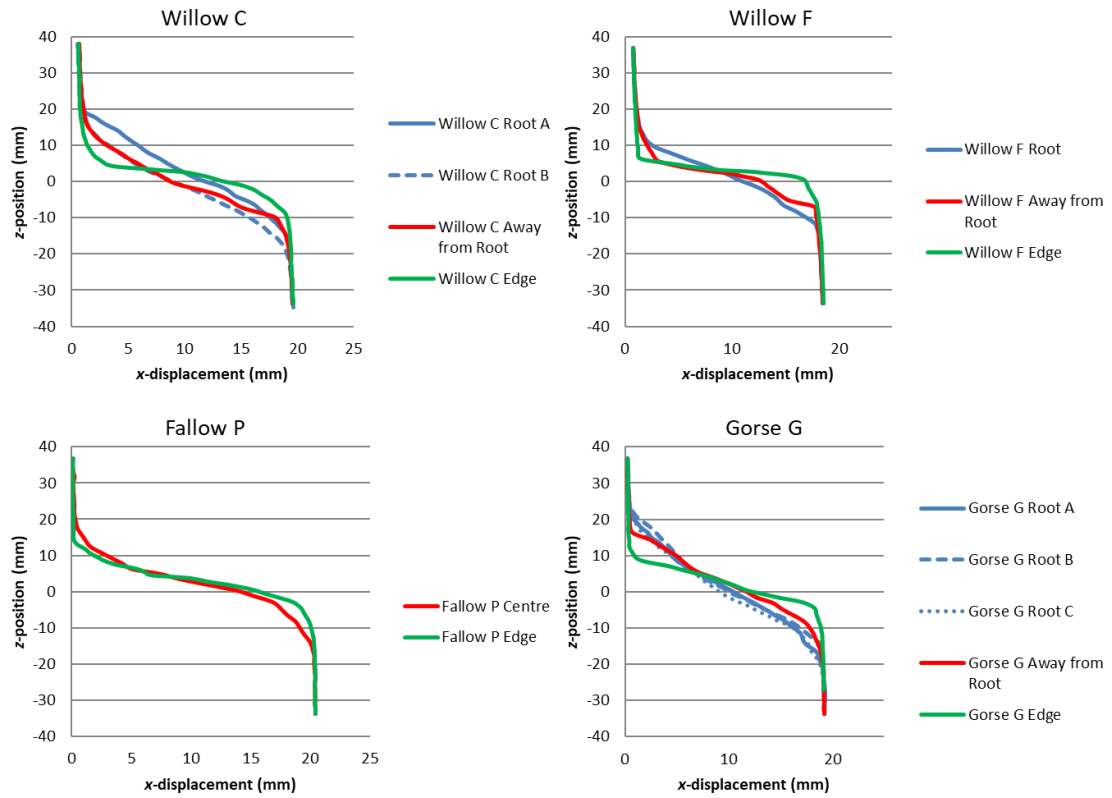
Figure 8: Depth vs x-displacement line profiles comparing responses at the root (blue lines), about 5 mm away from the root or at the centre of the specimen (red lines), and towards the edge of the DVC field of view (green lines). The displacements are determined from the DVC, and are the difference between step 7 and the undeformed volume.
