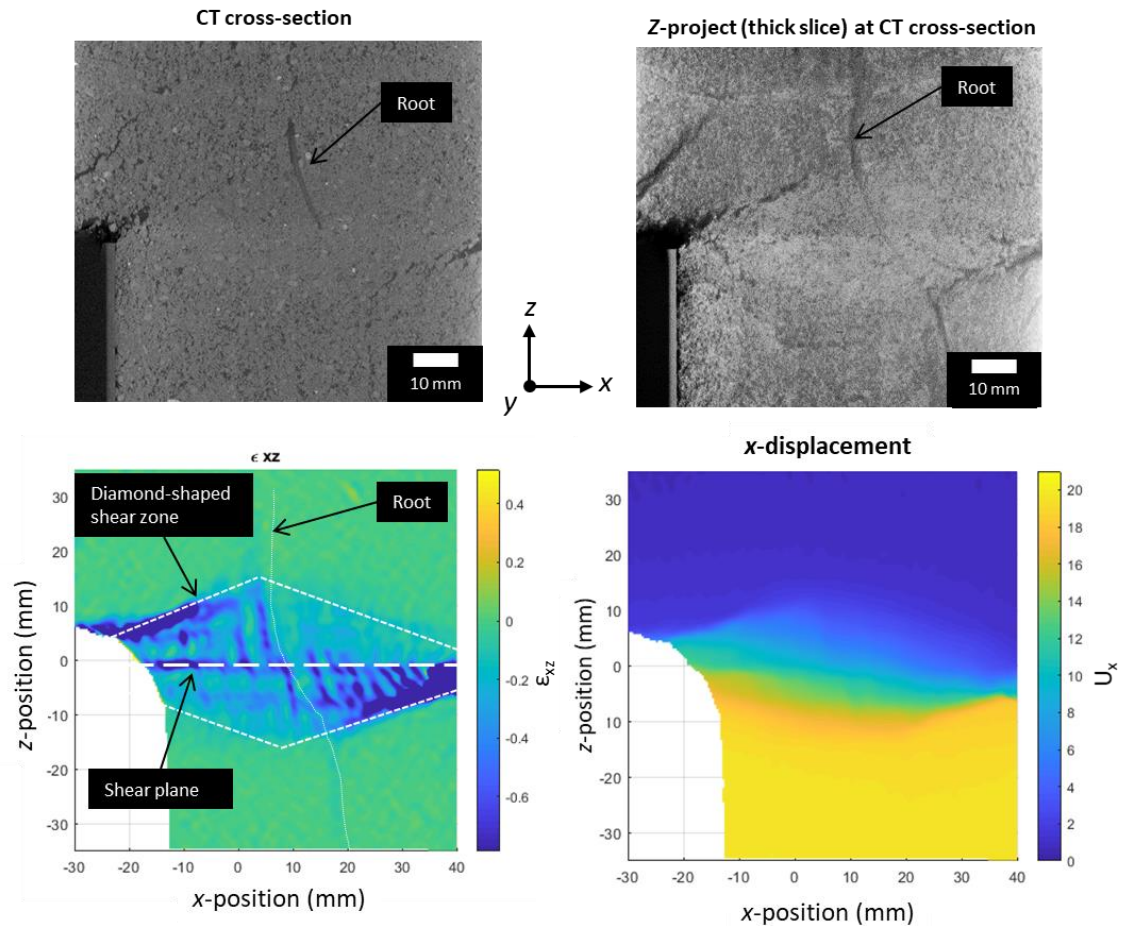
Figure 6: XCT cross-section and Z-project (thick slice) of Willow C specimen after the final shear displacement step. A diamond-shaped shear zone is observed as highlighted in the shear strain ( \epsilon_{xz} ) and x-displacement ( U_x ) DVC data.
