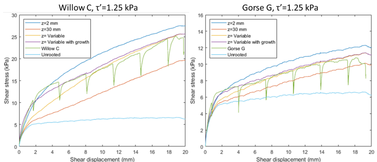
Figure 16: Shear stress vs shear displacement for Willow C and Gorse G specimens. Plots show modified Waldron model ( Z = 2 mm, 30 mm, spatially variable, and variable with shear zone thickness growth) and experimental results (Willow C, Gorse G and Unrooted). In the Z = variable case, the shear zone thickness Z is determined from the position of the root on the shear plane.
