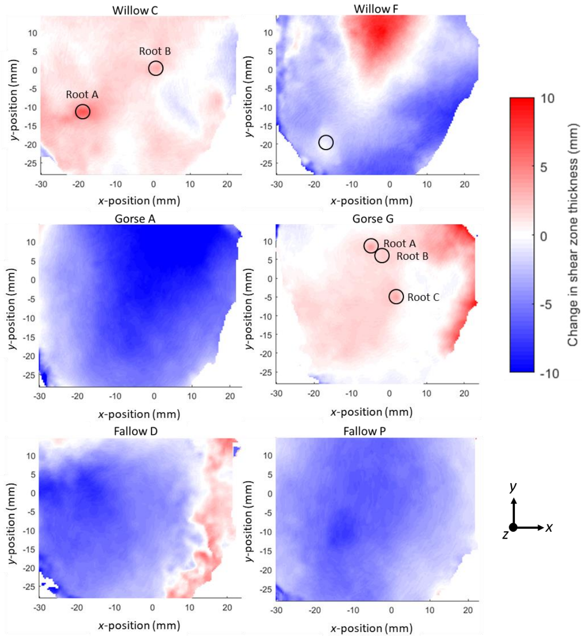
Figure 9: Change in shear zone thickness between displacement steps 3 and 7. Positive values represent an increase in shear zone thickness with increasing shear displacement. Roots >1 mm in diameter are circled.
