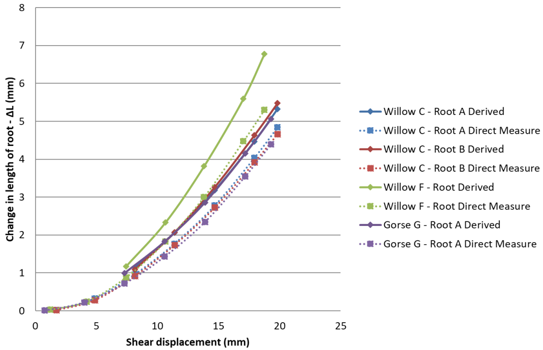
Figure 11: Comparison between changes in root length derived using Equation 5 and measured directly from the root path geometry.
