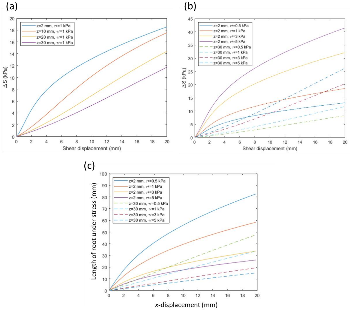
Figure 15: Waldron model parameter sensitivity study. (a) effect of shear zone thickness ( z ) on the additional soil resistance provided by the roots ( \Delta S ). (b) effect of soil-root interconnectivity ( \tau' ) and shear zone thickness on \Delta S . (c) effective length of a 1.0 mm diameter root under stress for different values of \tau' and Z=2 or Z=30 mm.
