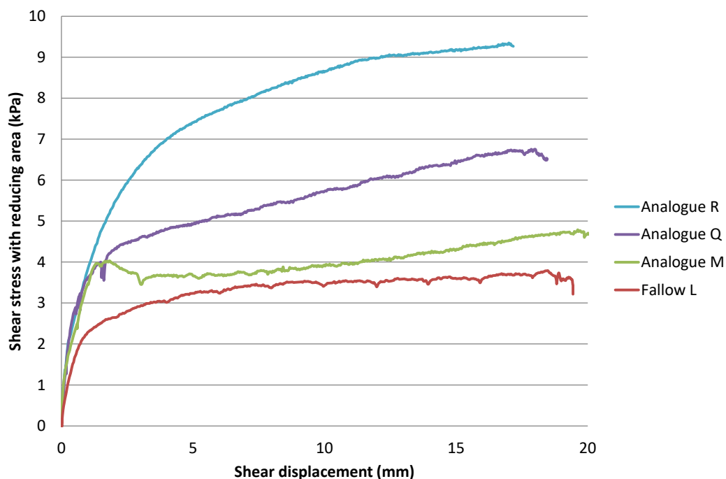
Figure 14: Shear stress-displacement curves for specimens containing an artificial root, and a fallow specimen.
