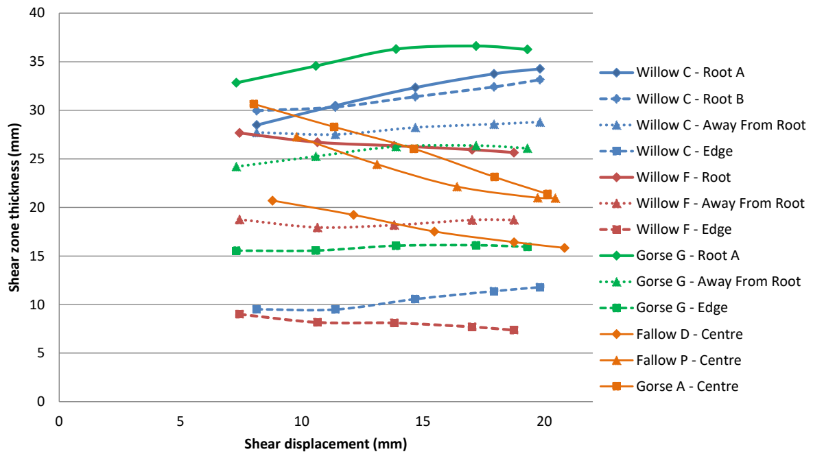
Figure 10: Change in shear zone thickness against shear displacement at different positions within rooted and unrooted test specimens. The results are for locations on or as near as possible to the segmented roots, from an x-y position about 5 mm away from segmented roots in the direction of the centre of the tube (marked on the plot as ‘away from root’), from the centre of the tube (fallow specimens), and from the edge of the DVC field of view (which did not extend to the edge of the specimen; see Figure 4).
