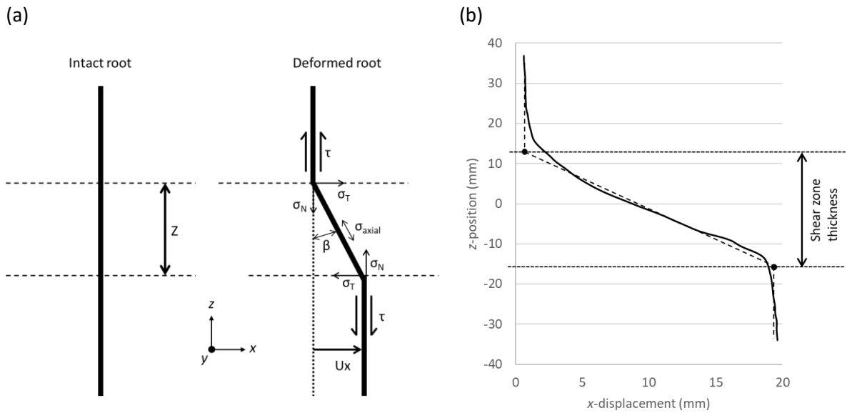
Figure 2: (a) Schematic illustrating the development of root stresses during direct shear [22]. (b) Example of tri-linear fit (dotted line) used to determine local shear zone thickness from z-position vs x-displacement (solid line) DVC data. The shear zone thickness was calculated at every (x,y) position on the shear plane, for each displacement step in the test.
