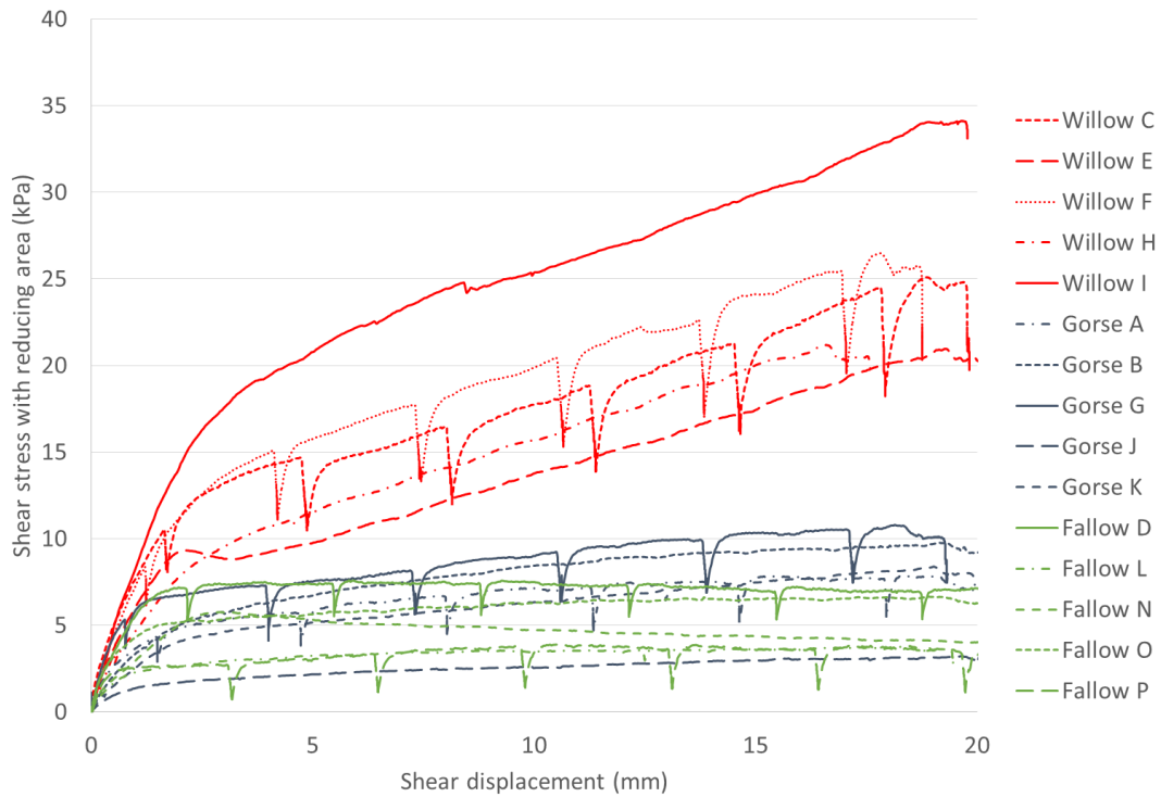
Figure 3: Direct shear stress - displacement plots for Willow (red), Gorse (blue) and Fallow (green) specimens.
