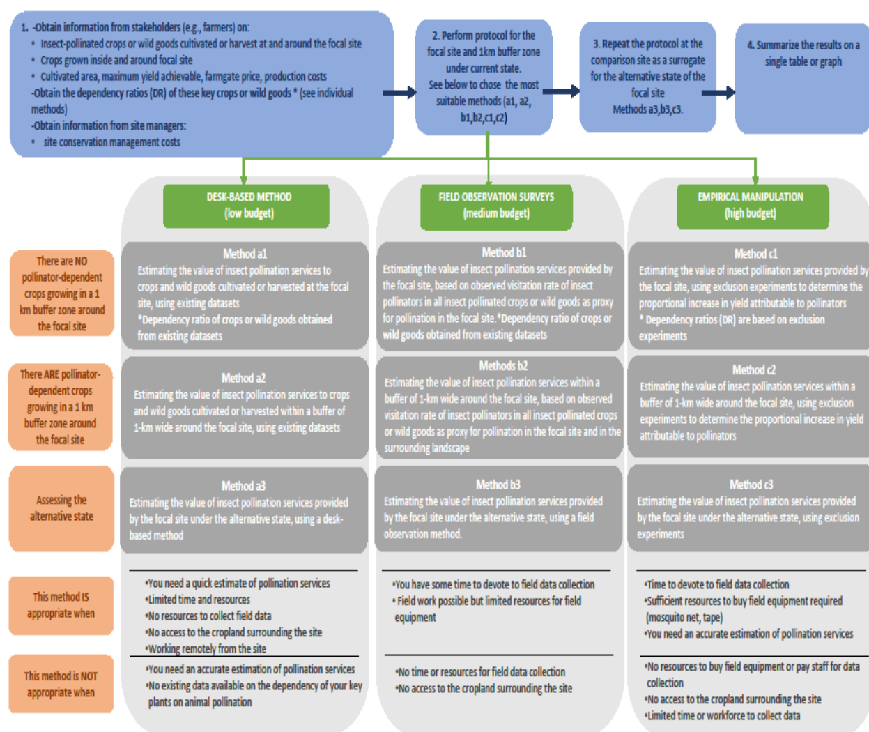
Figure 1. Flowchart detailing the steps to follow to perform the insect pollination service protocol and guiding the selection the most appropriate method. Dependency ratio is defined as the proportional increase in yield directly attributable to pollinators. The buffer is the area within 1-km radius from the focal site.
