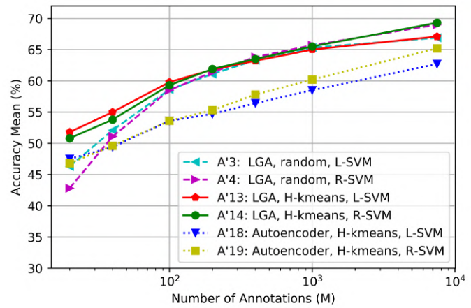
(b) Annotations ( M ) vs F_1 (macro-average) means averaged over the Mountain, Island and Urban Aerial Datasets
