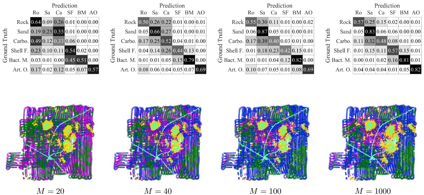
Fig. 5: Confusion matrices and habitat maps predicted by ResNet18 trained using the proposed LGA-SS method with hierarchical k means based data selection and pseudo-labelling (configuration D7 in TABLE 3). Compared to Fig. 4, the results show improved learning efficiency, especially for small values of M , where both the 'Artificial Object' and 'Bacterial Mat' classes are efficiently learned using just 20 human annotations, despite these being rare classes with a small number of data samples. The performance with M = 100 shows similar performance to when the same CNN architecture is trained using an order of magnitude more annotations from randomly selected data (i.e Fig. 4).
