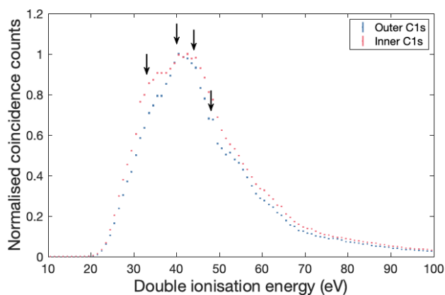
Fig. 3 Double ionization spectra of allene measured with 300.5 eV photon energy. The spectra have been selected on outer and inner C1s core electron, respectively. The inner C1s electron has a binding energy of 290.8 eV and the outer C1s electron has 290.6 eV 29 , and the selections comprise binding energy ranges of \pm 0.1 eV. The arrows indicate structures in the ionization spectra at energies of about 33, 40, 44 and 48 eV.
