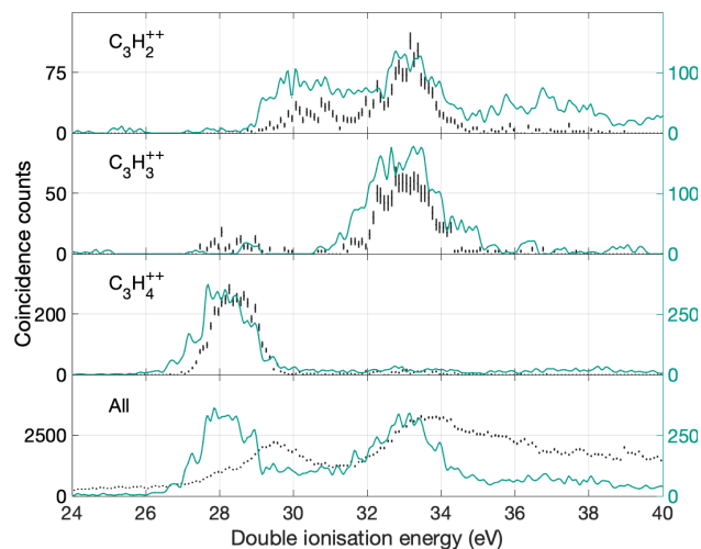
Fig. 9 Double ionization spectra based on electrons that were detected in coincidence with the charge retaining parent species or with charge retaining fragments which lost one or two hydrogen atoms. Because the detected species is doubly ionised and triple ionization is impossible at this photon energy, no other ions can be involved in these events. The green line indicates the double ionization of the entire peak estimated from a Gaussian fit to three peaks to three overlapping peaks in the ion spectrum. The lowermost plot in black is the entire double ionization spectrum of all ions and the green line indicates the double ionization of the three peaks in green in the above panels, combined. All green spectra lack error bars because of the scaled number of counts with respect to the peak area.
