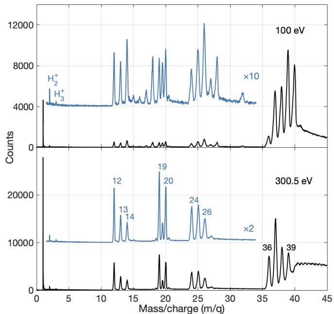
Fig. 5 Mass spectra of allene at photon energies 100 eV (upper panel) and 300.5 eV (lower panel). The mass spectrum at 40.8 eV (not shown) is very similar to the 100 eV spectrum. The black spectra are multiplied by a factor of 10 and 2 in the upper and lower panel, respectively. The numbers refer to the mass over charge assigned to the specific peaks.
