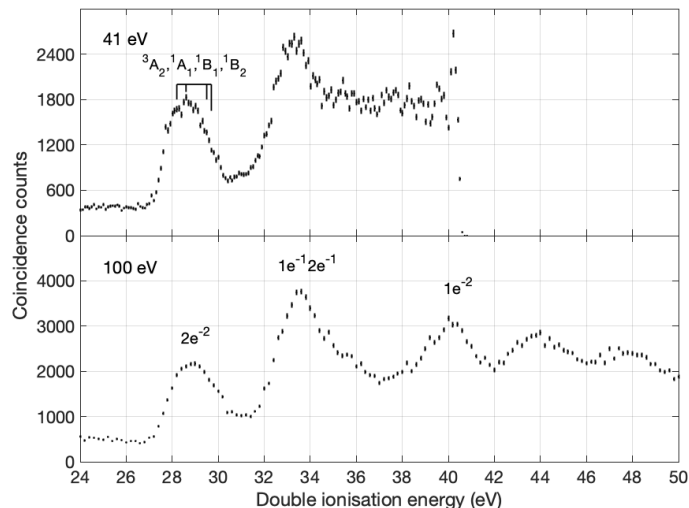
Fig. 2 Double ionization electron spectra of allene measured at the photon energies of 40.8 eV (upper panel) and 100 eV (lower panel). The 40.8 eV data were taken in Gothenburg with a helium gas discharge lamp and the 100 eV data were taken at BESSY-II in Berlin. Both spectra are based on electron pair measurements. Assignments in terms of leading configuration (lower panel), and for the lowest structure in the 40.8 eV spectrum in terms of different electronic states (upper panel) are included.
