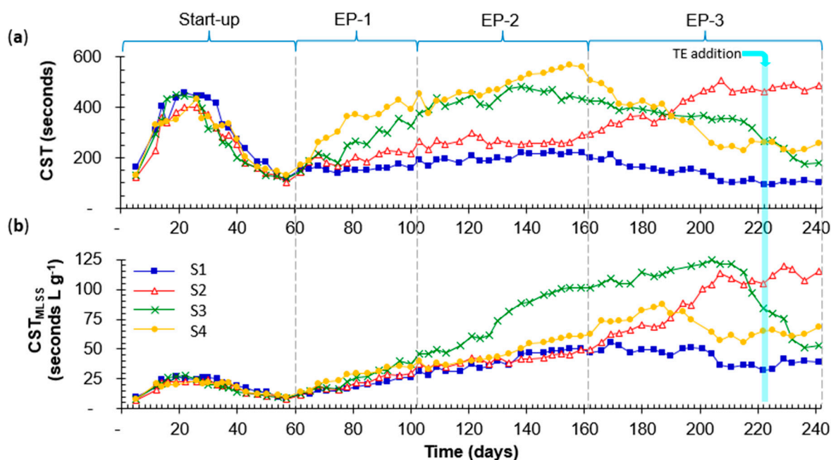
Figure 4. Mixed liquor filterability in SAnMBRs during the whole experimental period: (a) CST; (b) CST_{MLSS} . Vertical dotted lines indicate the start of experimental phases. Values for control parameters (SRT and TMP) in each phase are shown in Figure 2 and Table A2.
