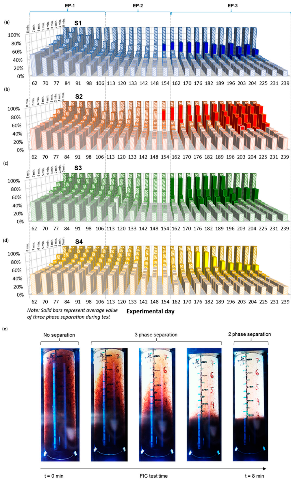
Figure 5. Mixed liquor centrifugation during experimental period: FIC test – Separated sludge volumes as % of original sample volume in (a) S1, (b) S2, (c) S3 and (d) S4, (e) separation phases during FIC test in centrifuged mixed liquor from S2 on day 204. Vertical dotted lines indicate start of experimental phases.
