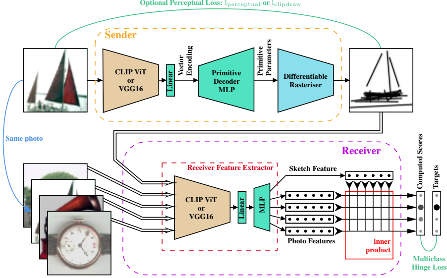
Figure 1: Model overview. Two agents are trained to play an image guessing game in which they communicate through a simple line drawing. As indicated, unlike in Mihai & Hare (2021b)’s original model, we also experiment with a more powerful pretrained Vision Transformer encoder module (ViT-B/32 from CLIP (Radford et al., 2021)). An additional perceptual loss (not shown) between the sender’s input photo and output sketch induces the sketch to be more understandable. Figure adapted from Mihai & Hare (2021b).
