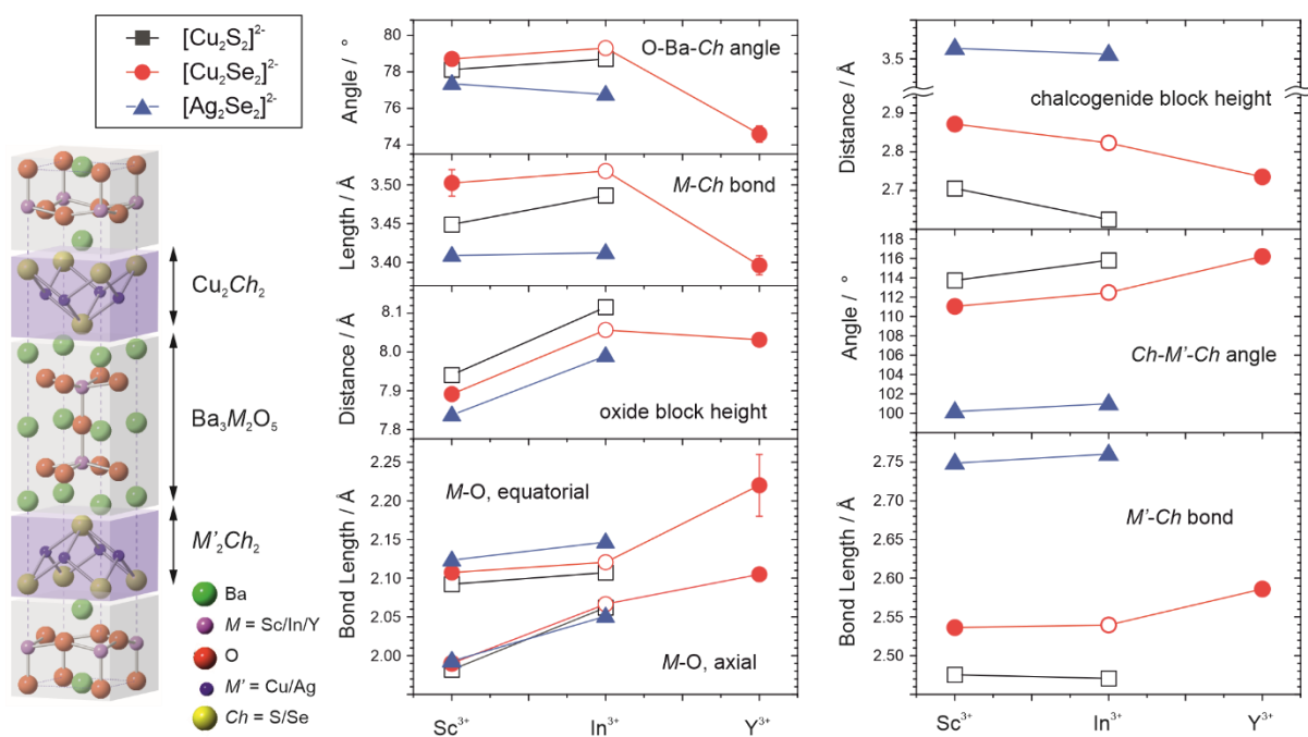
Figure 4. Left: Schematic diagram of the unit cell of the Ba_3M_2O_5M'_2Ch_2 ; ( M = Sc, In, Y ), ( M' = Cu, Ag ) and ( Ch = S, Se ). Centre and Right: Plots of the key angles, bond lengths and distances within the structure for the oxide and chalcogenide blocks. Values plotted as a function of the M ion in the oxide block, with chalcogenide layer distinguished by black squares for [Cu_2S_2]^{2-} , red circles for [Cu_2Se_2]^{2-} , and blue triangles for [Ag_2Se_2]^{2-} . Filled symbols are for new materials reported here, empty symbols are from prior literature, references 3,4 and 9. The lines shown connect samples with the same chalcogenide layer as a guide to the eye. Where they are not shown, the error bars are smaller than the symbols used.
