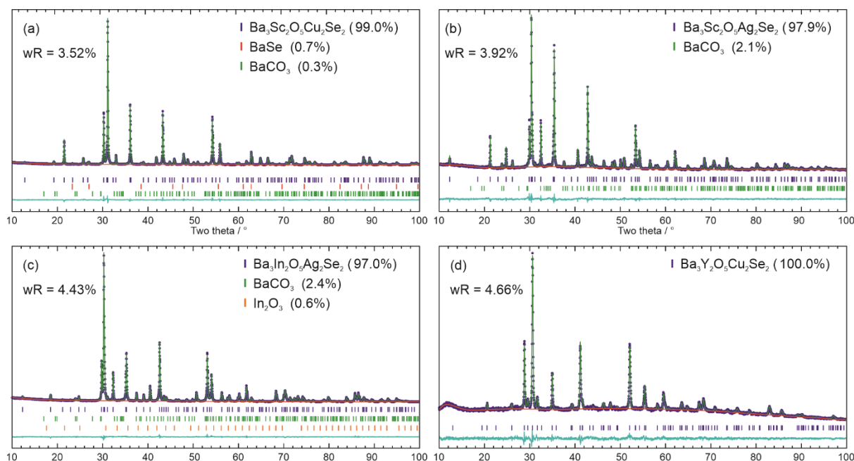
Figure 2. Rietveld refinement fits of the I4/mmm structure to diffraction data, with purity by mass and wRp fit values given for each data set: a) Ba_3Sc_2O_5Cu_2Se_2 ; b) Ba_3Sc_2O_5Ag_2Se_2 ; c) Ba_3In_2O_5Ag_2Se_2 ; d) Ba_3Y_2O_5Cu_2Se_2 . In each plot the diffraction data is shown in blue, the model in in green and the background in red. Below the data are tick marks indicating the positions of the peaks, and a cyan difference curve.
