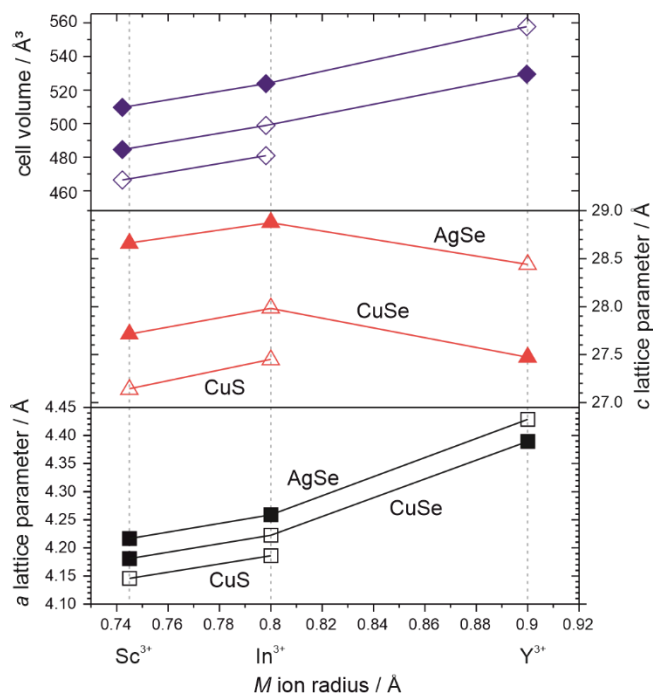
Figure 3 Plot of the lattice parameters for the I4/mmm structured Ba_3M_2O_5M'_2Ch_2 phase plotted against the ionic radius of the M^{3+} ion present in each sample. Guidelines indicate and connect the samples with the same heavy anion layer. The a parameter is shown in the lower graph with squares, and the c lattice parameter in the middle graph with triangles. The top graph depicts the cell volume versus M ionic radii. Open symbols indicate previously reported materials, from references 3, 4 and 9, closed symbols represent novel materials reported in this paper.
