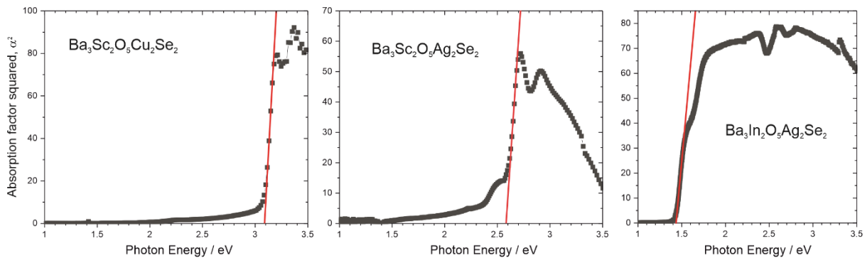
Figure 6. Plots of \alpha^2 against photon energy for novel compositions, \text{Ba}_3\text{Sc}_2\text{O}_5\text{Cu}_2\text{Se}_2 , \text{Ba}_3\text{Sc}_2\text{O}_5\text{Ag}_2\text{Se}_2 , and \text{Ba}_3\text{In}_2\text{O}_5\text{Ag}_2\text{Se}_2 , to allow band gaps to be determined from tangents shown in red. Absorption co-efficient determined using the Kubelka-Munk transformation. Spectra for yttrium containing samples could not be obtained due to air sensitivity.
