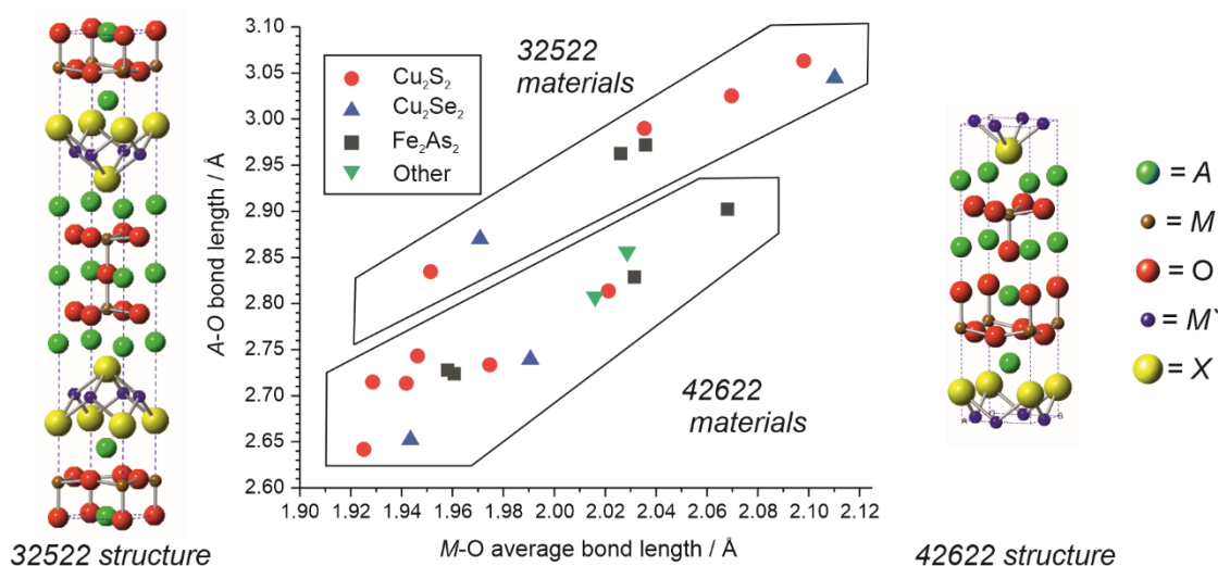
Figure 1. Structure Map of layered mixed anion phases showing adoption of either 32522 or 42622. Examples with copper sulphide heavy layers are indicated by red circles, copper selenide by blue triangles, iron arsenides by black squares, and the less common layers (iron phosphide, cobalt arsenide, nickel phosphide and nickel arsenide) by green triangles.
