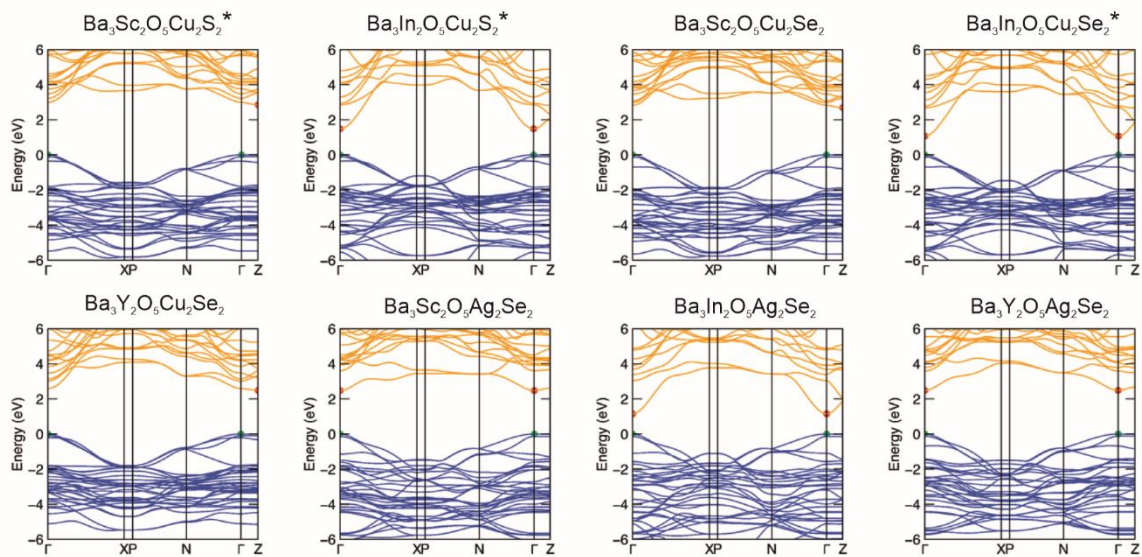
Figure 5. Electronic band structures of the eight thermodynamically stable \text{Ba}_3\text{M}_2\text{O}_5\text{M}'_2\text{Ch}_2 compounds calculated using the HSE06 DFT functional. Red and green dots mark the conduction band minimum (CBM) and valence band maximum (VBM), respectively. Compositions marked with an asterisk have been published previously. 3-4
