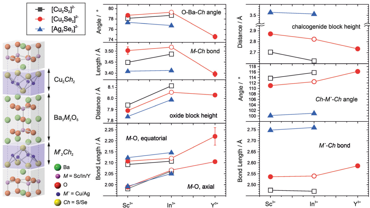
Fig. 4 Left schematic diagram of the unit cell of the Ba_3M_2O_5M'_2Ch_2 ; [(M = Sc, In, Y), ( M' = Cu, Ag) and (Ch = S, Se)]. Centre and right plots of the key angles, bond lengths and distances within the structure for the oxide and chalcogenide blocks. Values plotted as a function of the M ion in the oxide block, with chalcogenide layer distinguished by black squares for [Cu_2S_2]^{2-} , red circles for [Cu_2Se_2]^{2-} , and blue triangles for [Ag_2Se_2]^{2-} . Filled symbols are for new materials reported here, empty symbols are from prior literature, ref. 3, 4 and 9. The lines shown connect samples with the same chalcogenide layer as a guide to the eye. Where they are not shown, the error bars are smaller than the symbols used.
